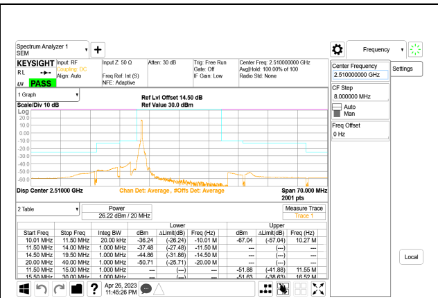
LTE B7 20MHz QPSK Low Channel RB1-0, ID:28567
