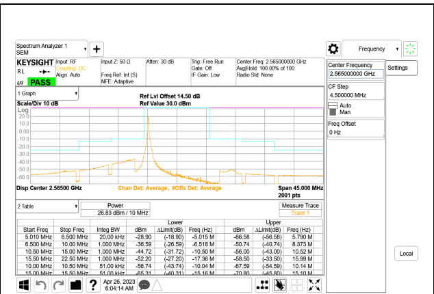
LTE B7 10MHz QPSK High Channel RB1-0, ID:28567
