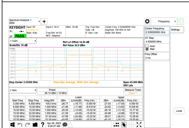
LTE B7 10MHz QPSK Middle Channel RB50-0, ID:28567
