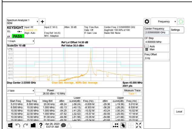
LTE B7 10MHz QPSK Middle Channel RB1-49, ID:28567
