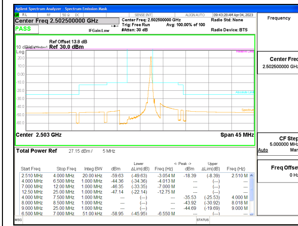
5G NR n7 5MHz BPSK Low Channel RB1-24, ID:28568
