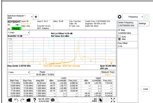
LTE B7 15MHz QPSK Low Channel RB1-74, ID:28567
