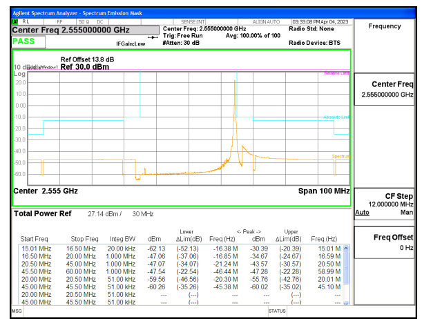
5G NR n7 30MHz BPSK High Channel RB1-159, ID:28568
