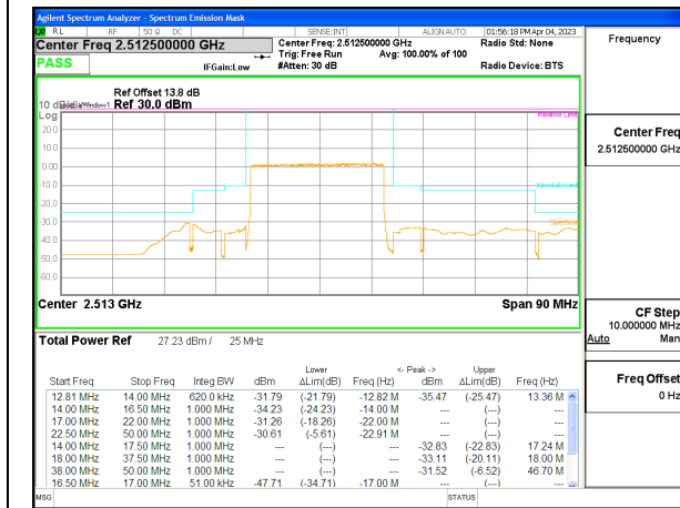
5G NR n7 25MHz BPSK Low Channel RB128-0, ID:28568
