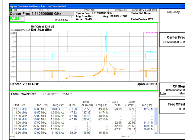
5G NR n7 25MHz BPSK Low Channel RB1-132, ID:28568
