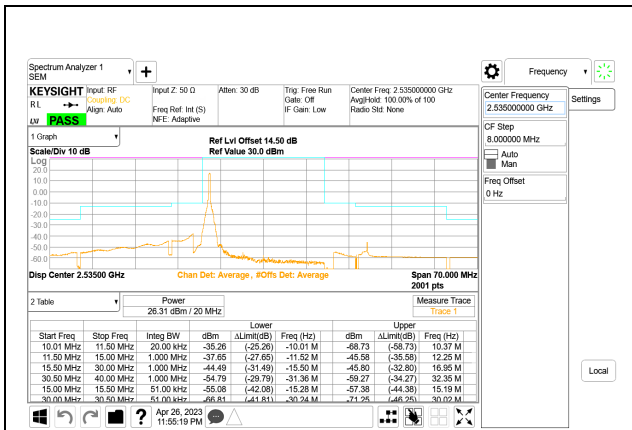
LTE B7 20MHz QPSK Middle Channel RB1-0, ID:28567
