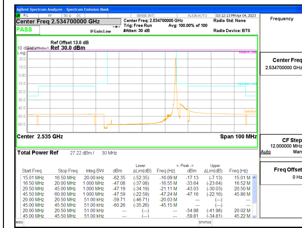
5G NR n7 30MHz BPSK Middle Channel RB1-159, ID:28568
