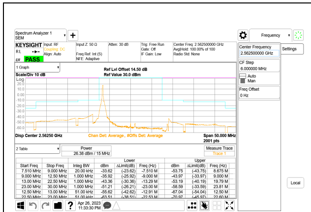
LTE B7 15MHz QPSK High Channel RB1-0, ID:28567
