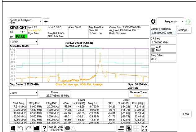
LTE B7 15MHz QPSK High Channel RB1-74, ID:28567
