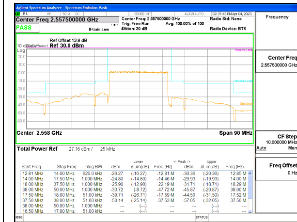
5G NR n7 25MHz BPSK High Channel RB128-0, ID:28568
