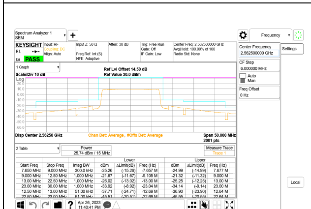
LTE B7 15MHz QPSK High Channel RB75-0, ID:28567
