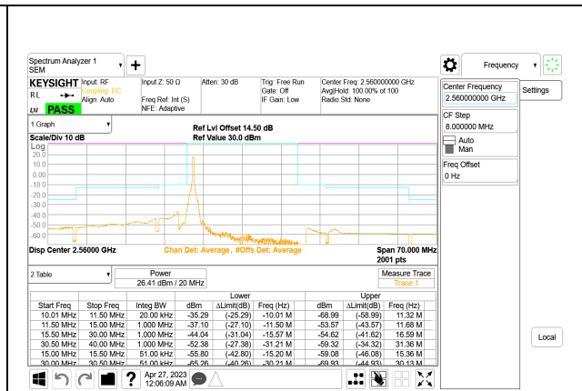
LTE B7 20MHz QPSK High Channel RB1-0, ID:28567
