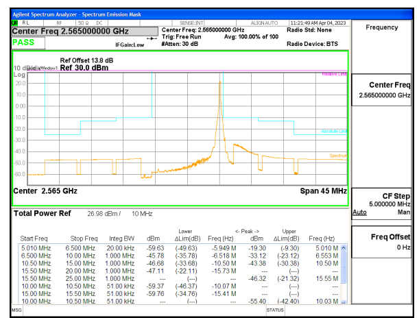
5G NR n7 10MHz BPSK High Channel RB1-51, ID:28568
