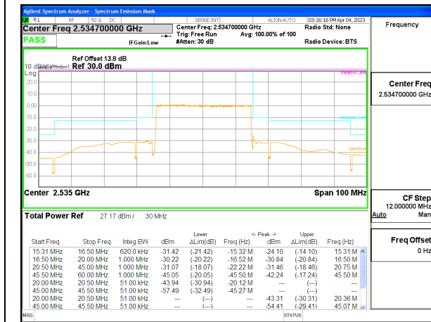
5G NR n7 30MHz BPSK Middle Channel RB160-0, ID:28568
