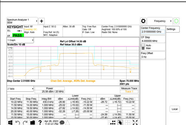
LTE B7 20MHz QPSK Low Channel RB100-0, ID:28567
