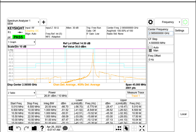
LTE B7 10MHz QPSK High Channel RB1-49, ID:28567
