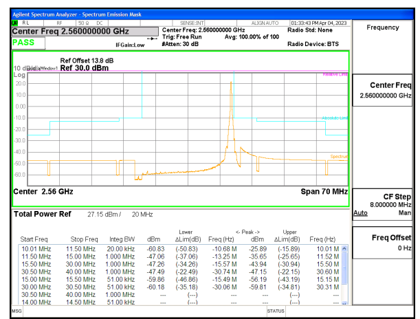
5G NR n7 20MHz BPSK High Channel RB1-105, ID:28568
