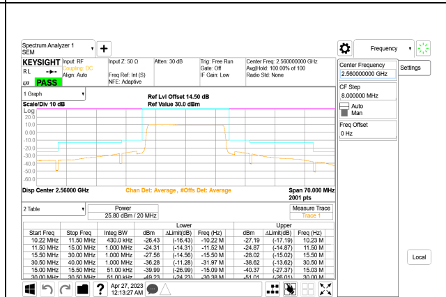
LTE B7 20MHz QPSK High Channel RB100-0, ID:28567
