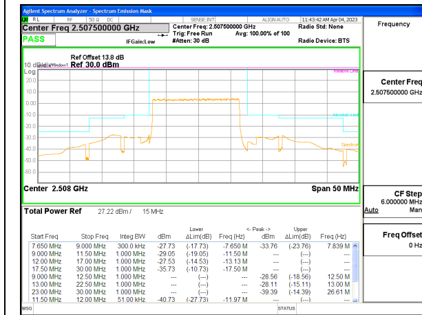
5G NR n7 15MHz BPSK Low Channel RB75-0, ID:28568
