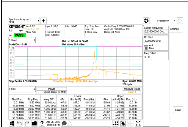
LTE B7 20MHz QPSK Middle Channel RB1-99, ID:28567
