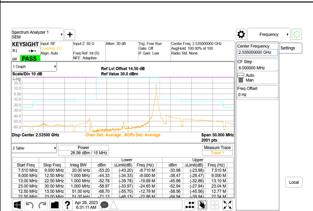
LTE B7 15MHz QPSK Middle Channel RB1-74, ID:28567
