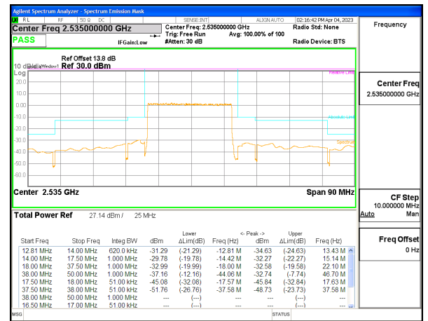
5G NR n7 25MHz BPSK Middle Channel RB128-0, ID:28568
