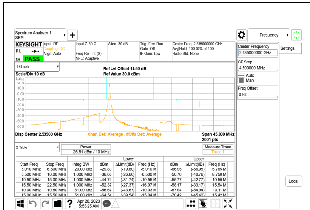
LTE B7 10MHz QPSK Middle Channel RB1-0, ID:28567
