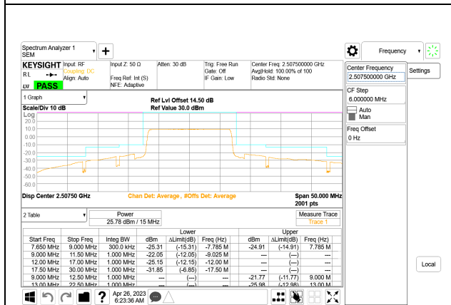
LTE B7 15MHz QPSK Low Channel RB75-0, ID:28567
