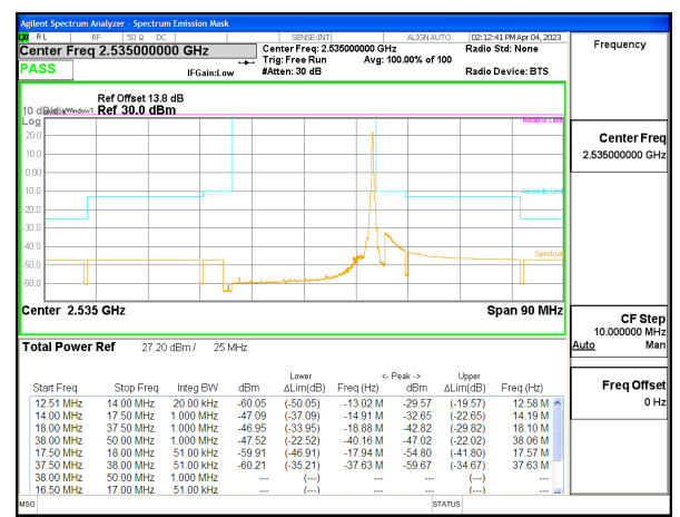
5G NR n7 25MHz BPSK Middle Channel RB1-132, ID:28568
