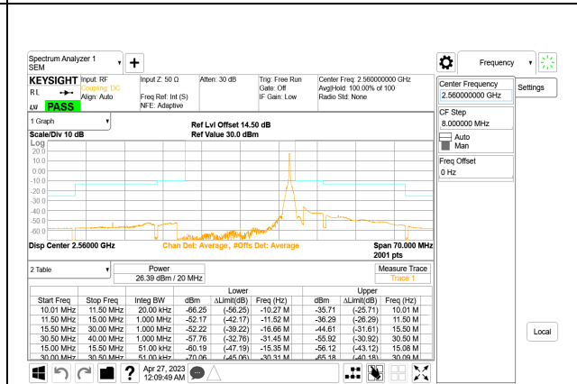
LTE B7 20MHz QPSK High Channel RB1-99, ID:28567
