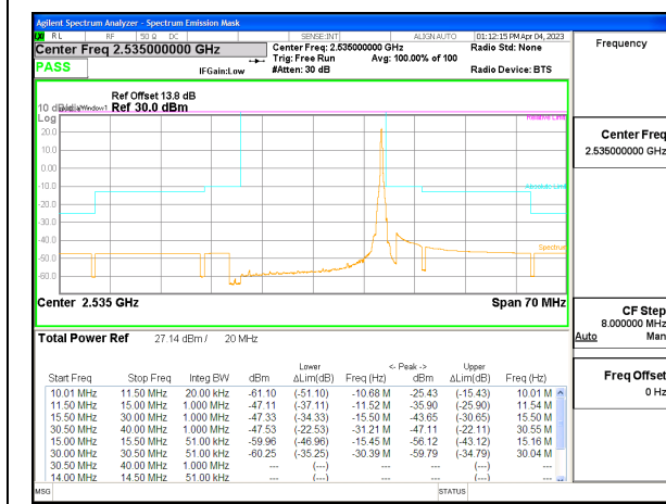
5G NR n7 20MHz BPSK Middle Channel RB1-105, ID:28568
