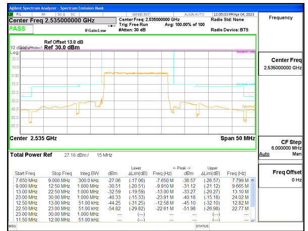
5G NR n7 15MHz BPSK Middle Channel RB75-0, ID:28568
