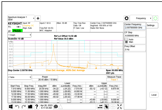
LTE B7 15MHz QPSK Low Channel RB1-0, ID:28567
