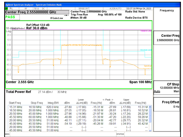
5G NR n7 30MHz BPSK High Channel RB160-0, ID:28568
