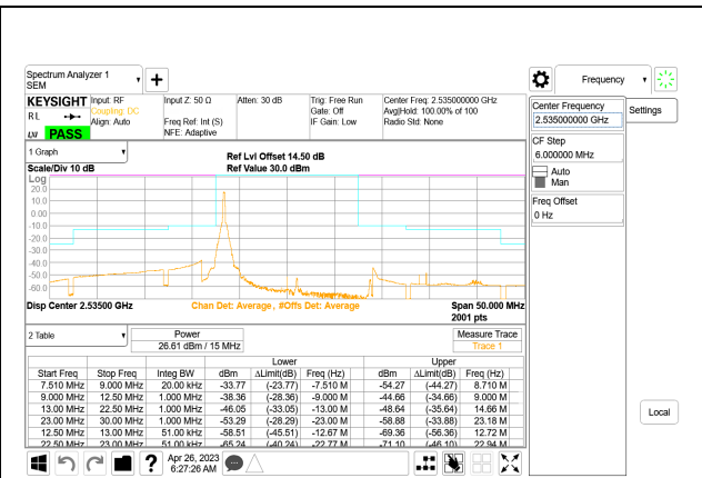
LTE B7 15MHz QPSK Middle Channel RB1-0, ID:28567
