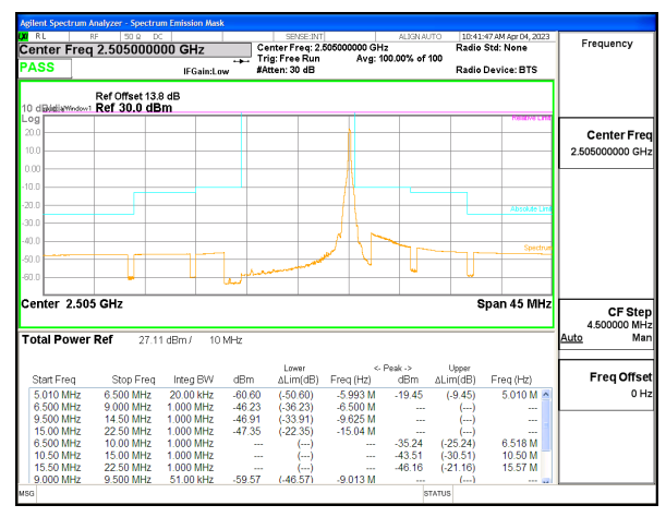
5G NR n7 10MHz BPSK Low Channel RB1-51, ID:28568
