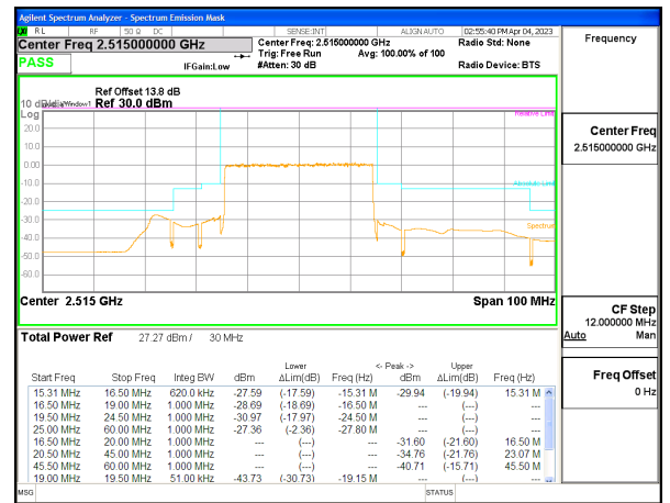
5G NR n7 30MHz BPSK Low Channel RB160-0, ID:28568
