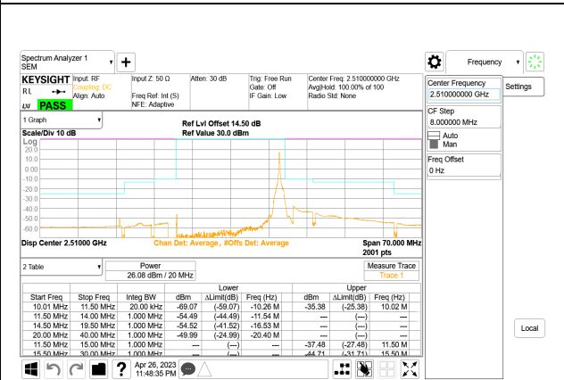
LTE B7 20MHz QPSK Low Channel RB1-99, ID:28567
