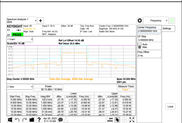
LTE B7 10MHz QPSK High Channel RB50-0, ID:28567
