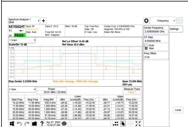
LTE B7 20MHz QPSK Middle Channel RB100-0, ID:28567
