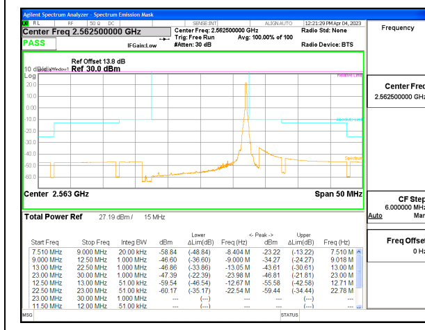
5G NR n7 15MHz BPSK High Channel RB1-78, ID:28568
