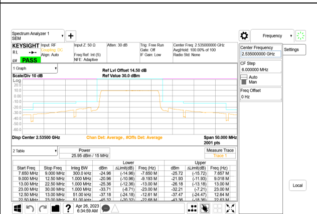
LTE B7 15MHz QPSK Middle Channel RB75-0, ID:28567
