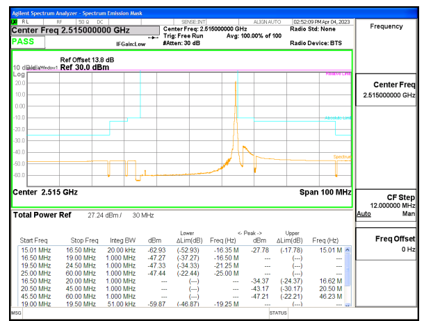
5G NR n7 30MHz BPSK Low Channel RB1-159, ID:28568
