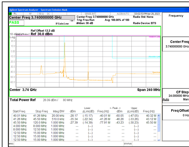
5G NR n77 80MHz BPSK Low Channel RB1-0, ID:28568
