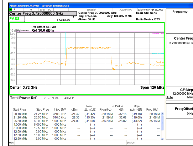
5G NR n77 40MHz BPSK Low Channel RB100-0, ID:28568
