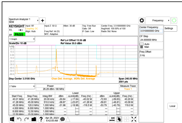
5G NR n77 80MHz BPSK High Channel RB1-0, ID:28568
