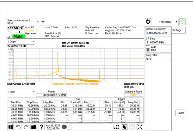
5G NR n77 70MHz BPSK Low Channel RB1-0, ID: 28568
