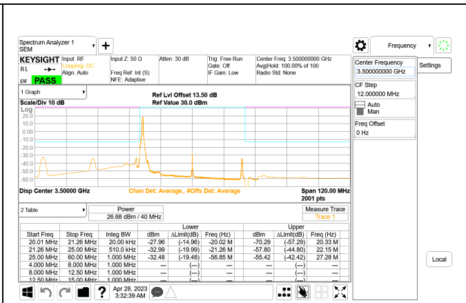
5G NR n77 40MHz BPSK Middle Channel RB1-0, ID:28568
