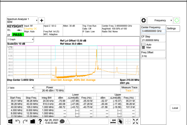
5G NR n77 70MHz BPSK Low Channel RB1-188, ID:28568
