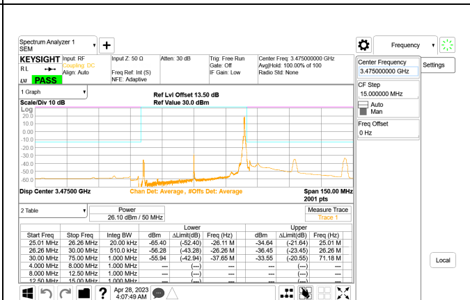
5G NR n77 50MHz BPSK Low Channel RB1-132, ID:28568
