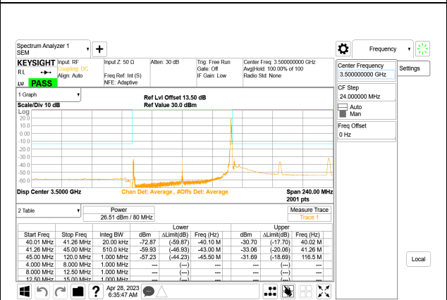
5G NR n77 80MHz BPSK Middle Channel RB1-216, ID:28568
