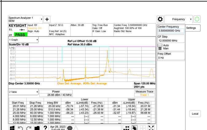
5G NR n77 40MHz BPSK Middle Channel RB1-105, ID:28568
