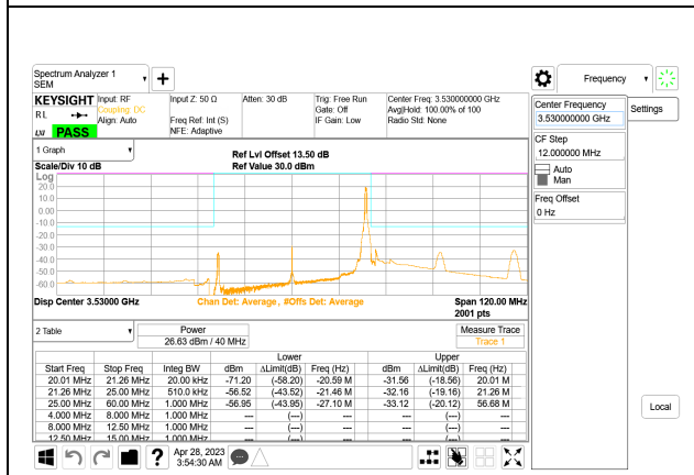
5G NR n77 40MHz BPSK High Channel RB1-105, ID:28568
