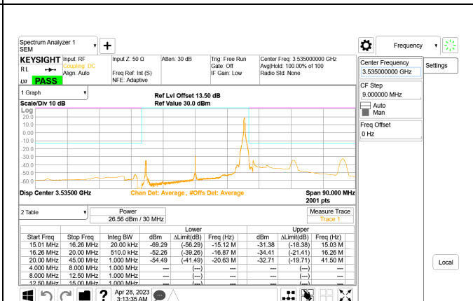
5G NR n77 30MHz BPSK High Channel RB1-77, ID:28568
