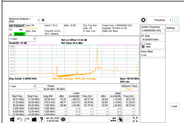
5G NR n77 60MHz BPSK Low Channel RB1-161, ID:28568
