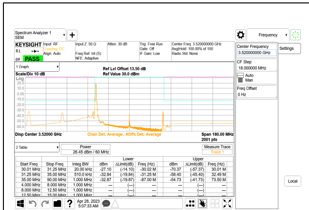
5G NR n77 60MHz BPSK High Channel RB1-0, ID:28568
