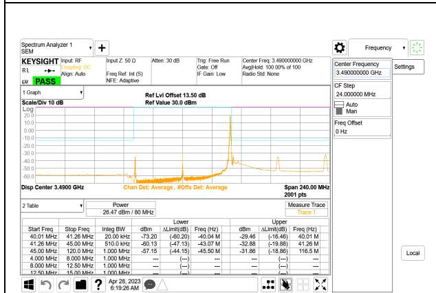
5G NR n77 80MHz BPSK Low Channel RB1-216, ID:28568
