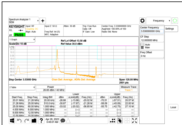
5G NR n77 40MHz BPSK High Channel RB1-0, ID:28568
