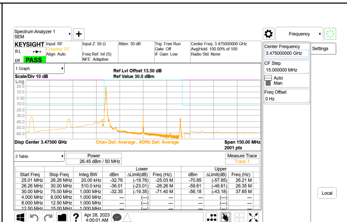
5G NR n77 50MHz BPSK Low Channel RB1-0, ID:28568
