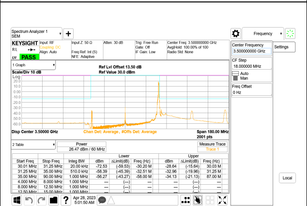
5G NR n77 60MHz BPSK Middle Channel RB1-161, ID:28568
