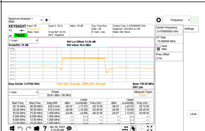
5G NR n77 50MHz BPSK Low Channel RB128-0, ID:28568
