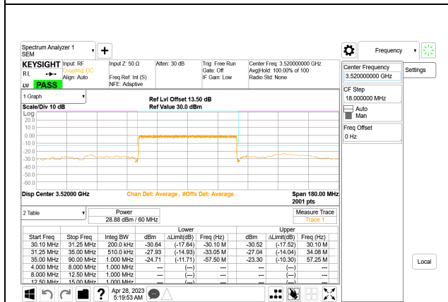
5G NR n77 60MHz BPSK High Channel RB162-0, ID:28568
