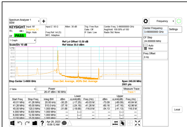
5G NR n77 80MHz BPSK Low Channel RB1-0, ID:28568
