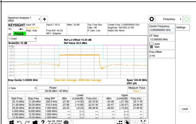
5G NR n77 40MHz BPSK Middle Channel RB100-0, ID:28568
