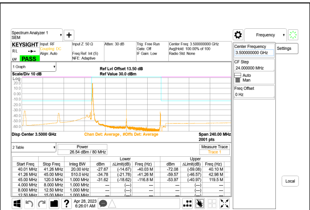
5G NR n77 80MHz BPSK Middle Channel RB1-0, ID:28568
