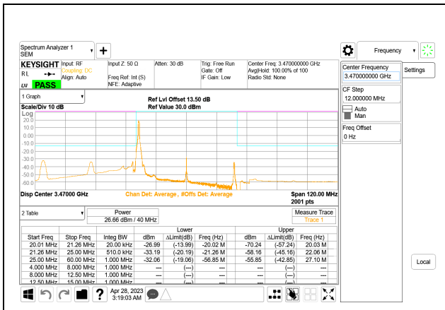
5G NR n77 40MHz BPSK Low Channel RB1-0, ID:28568
