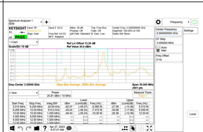
5G NR n77 10MHz BPSK Middle Channel RB1-23, ID:28568
