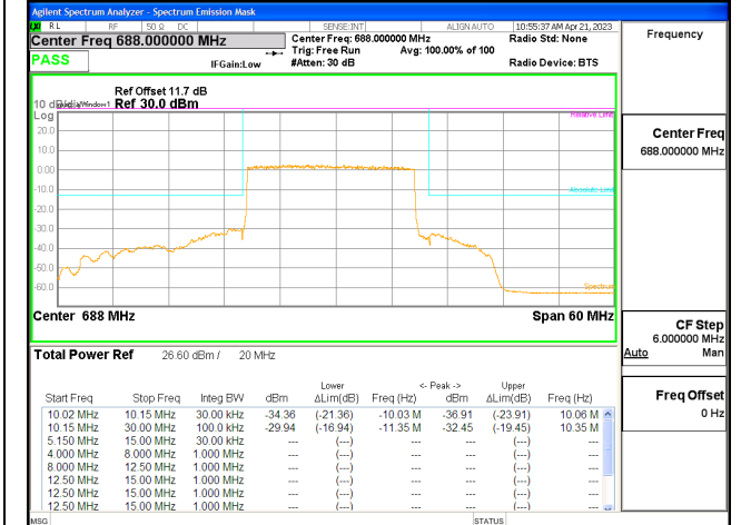
5G NR n71 20MHz BPSK High Channel RB100-0, ID:28568
