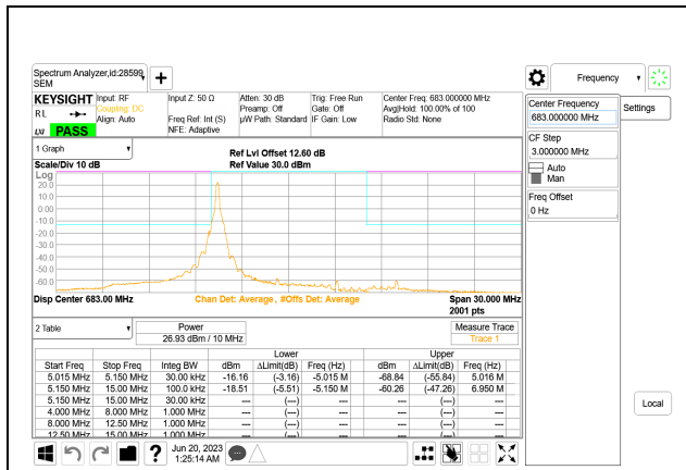
5G NR n71 10MHz BPSK Middle Channel RB1-0
