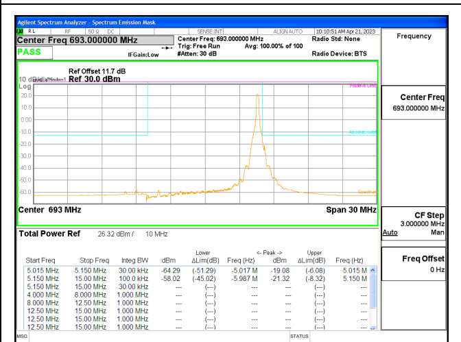
5G NR n71 10MHz BPSK High Channel RB1-51, ID:28568
