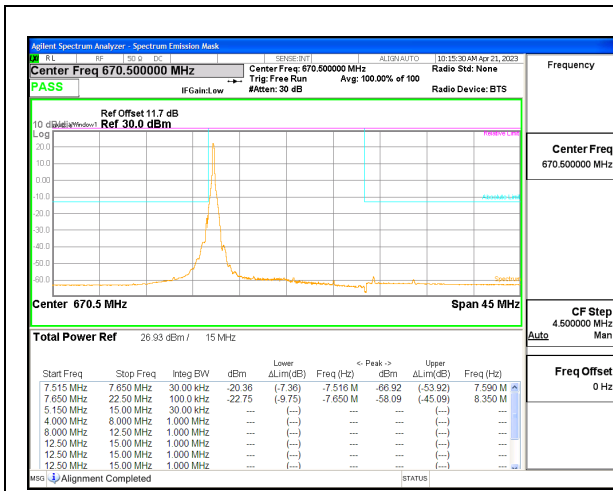
5G NR n71 15MHz BPSK Low Channel RB1-0, ID:28568
