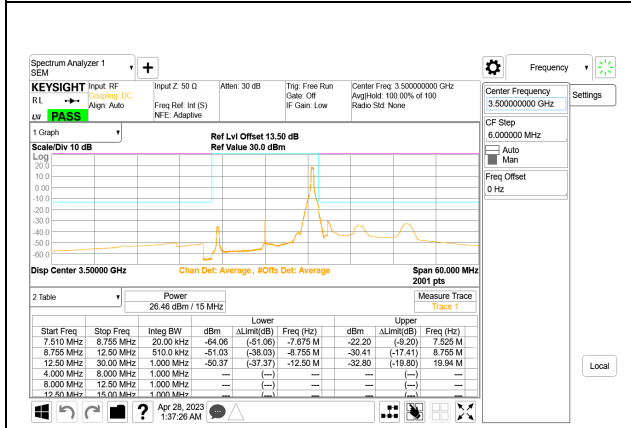
5G NR n77 15MHz BPSK Middle Channel RB1-37, ID:28568
