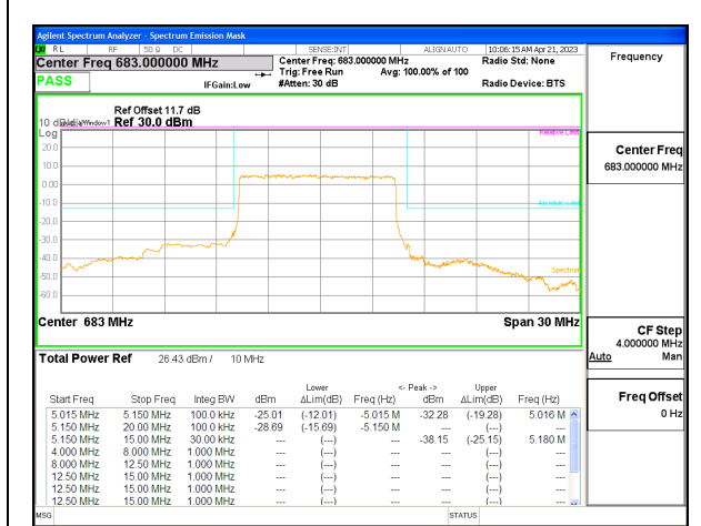
5G NR n71 10MHz BPSK Middle Channel RB50-0, ID:28568
