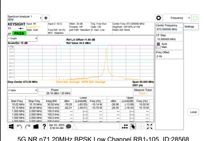
5G NR n71 20MHz BPSK Low Channel RB1-105, ID:28568
