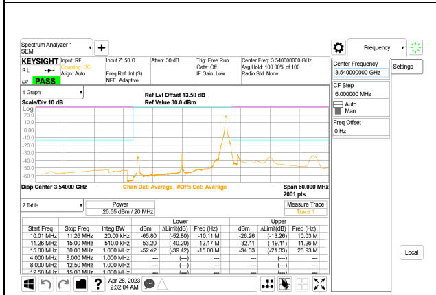
5G NR n77 20MHz BPSK High Channel RB1-50, ID:28568
