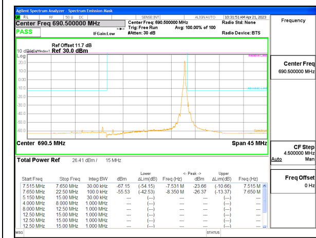
5G NR n71 15MHz BPSK High Channel RB1-78, ID:28568
