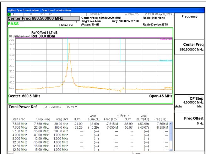
5G NR n71 15MHz BPSK Middle Channel RB1-0, ID:28568
