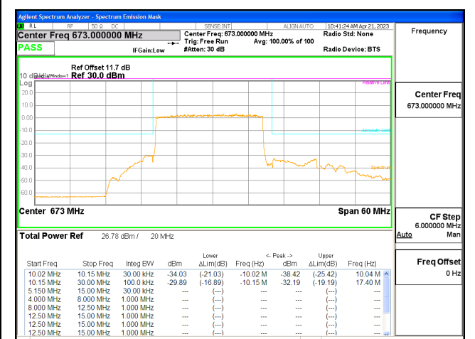
5G NR n71 20MHz BPSK Low Channel RB100-0, ID:28568
