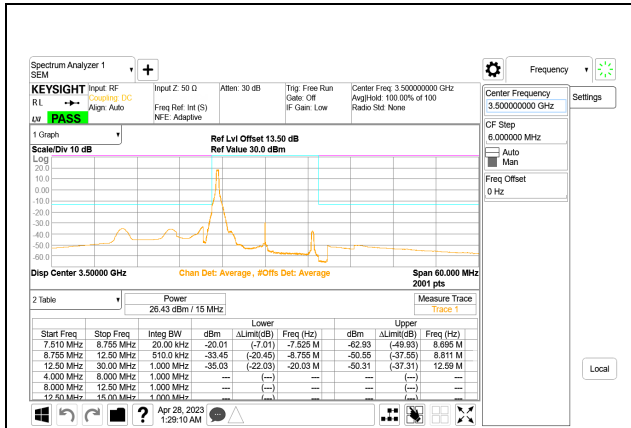
5G NR n77 15MHz BPSK Middle Channel RB1-0, ID:28568
