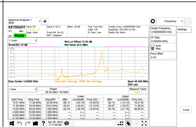
5G NR n77 20MHz BPSK Middle Channel RB1-50, ID:28568
