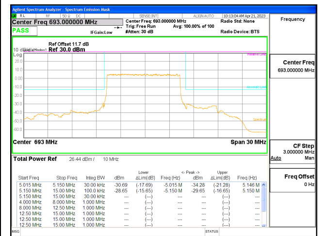
5G NR n71 10MHz BPSK High Channel RB50-0, ID:28568
