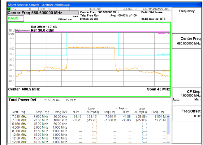
5G NR n71 15MHz BPSK Middle Channel RB75-0, ID:28568
