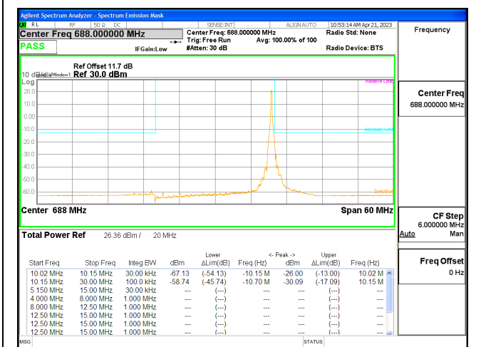
5G NR n71 20MHz BPSK High Channel RB1-105, ID:28568
