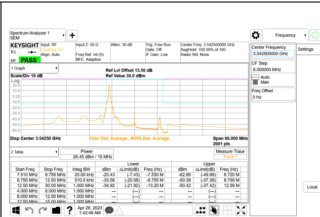
5G NR n77 15MHz BPSK High Channel RB1-0, ID:28568
