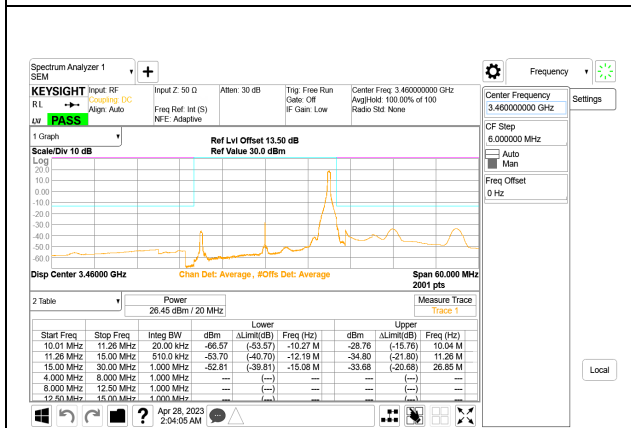
5G NR n77 20MHz BPSK Low Channel RB1-50, ID:28568
