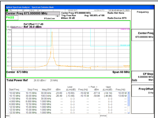
5G NR n71 20MHz BPSK Low Channel RB1-0, ID:28568
