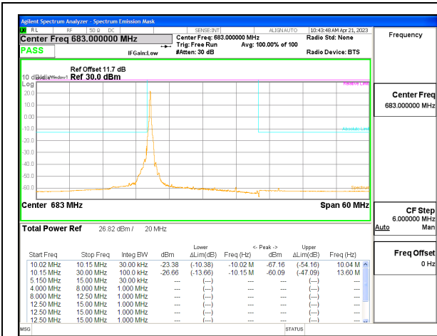
5G NR n71 20MHz BPSK Middle Channel RB1-0, ID:28568
