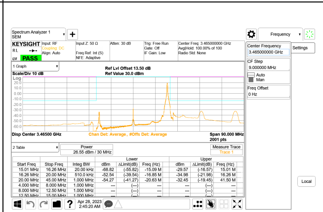
5G NR n77 30MHz BPSK Low Channel RB1-77, ID:28568
