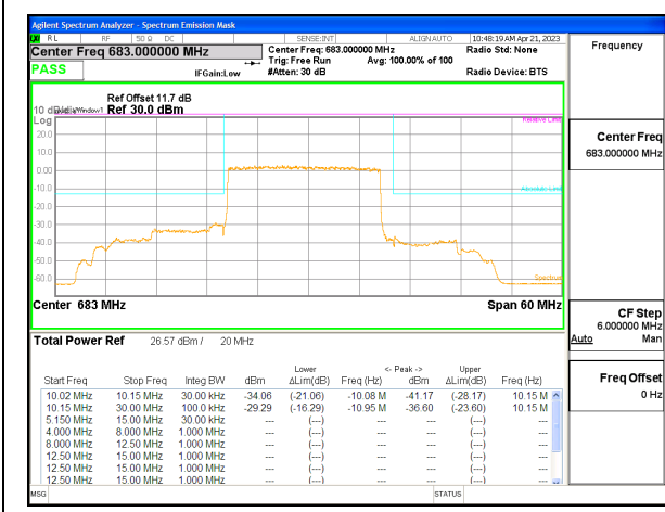
5G NR n71 20MHz BPSK Middle Channel RB100-0, ID:28568
