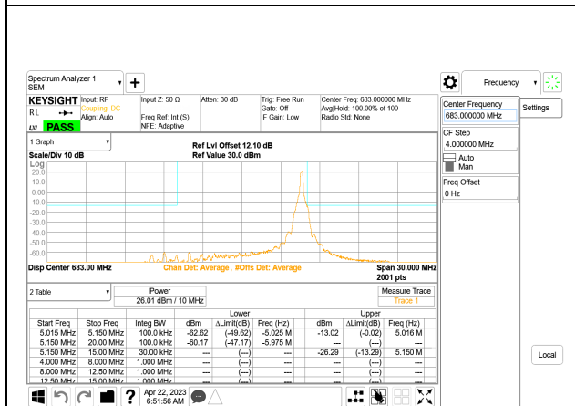
5G NR n71 10MHz BPSK Middle Channel RB1-51, ID:28568
