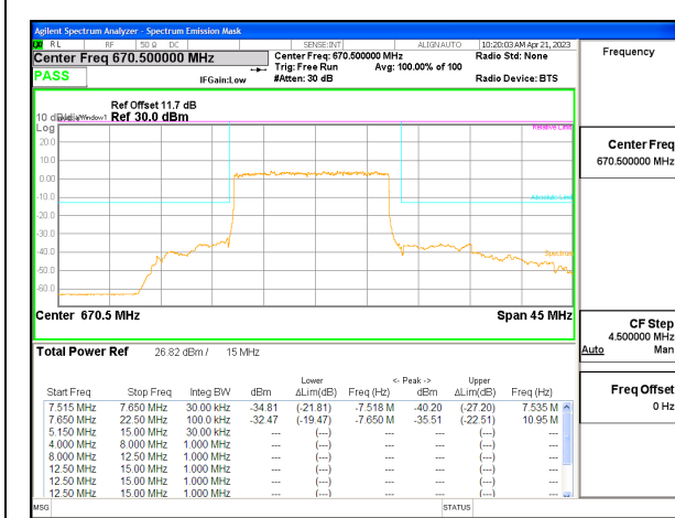
5G NR n71 15MHz BPSK Low Channel RB75-0, ID:28568
