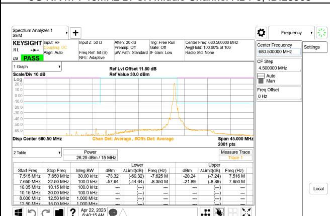
5G NR n71 15MHz BPSK Middle Channel RB1-78, ID:28568
