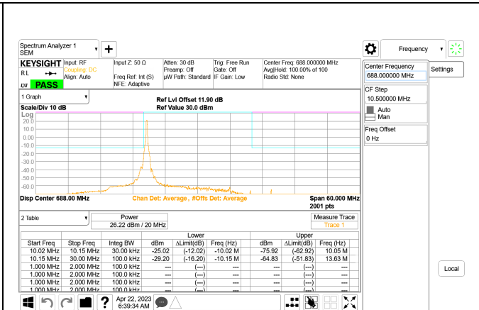
5G NR n71 20MHz BPSK High Channel RB1-0, ID:28568
