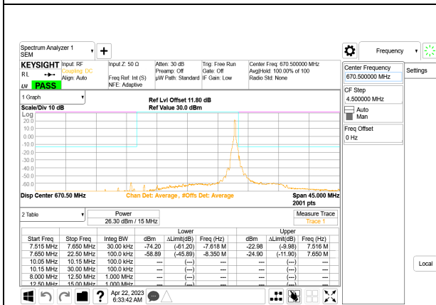
5G NR n71 15MHz BPSK Low Channel RB1-78, ID:28568
