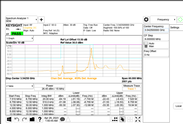
5G NR n77 15MHz BPSK High Channel RB1-37, ID:28568
