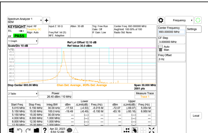
5G NR n71 10MHz BPSK High Channel RB1-0, ID:28568
