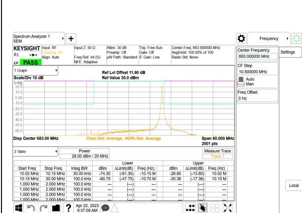
5G NR n71 20MHz BPSK Middle Channel RB1-105, ID:28568
