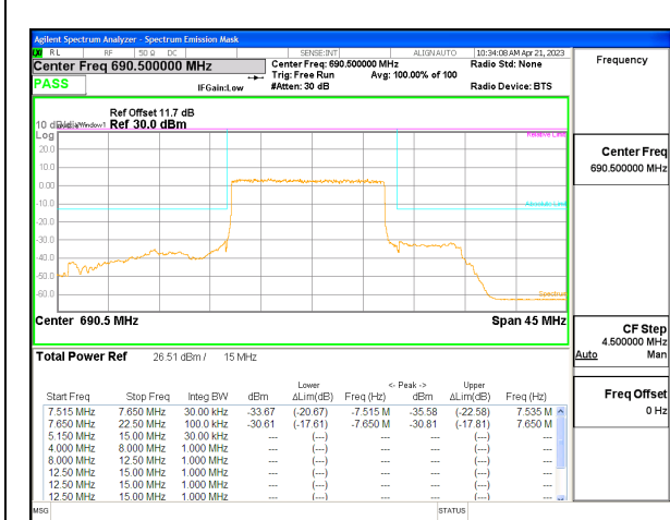
5G NR n71 15MHz BPSK High Channel RB75-0, ID:28568
