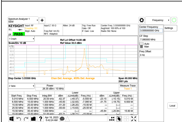
5G NR n48 10MHz BPSK Low Channel RB1-23, ID:28567
