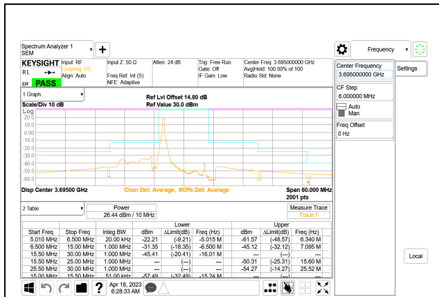
5G NR n48 10MHz BPSK High Channel RB1-0, ID:28567
