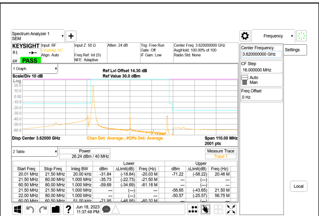
5G NR n48 40MHz BPSK Middle Channel RB1-0, ID:32586
