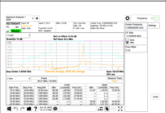
5G NR n48 30MHz BPSK Low Channel RB1-77, ID:32586
