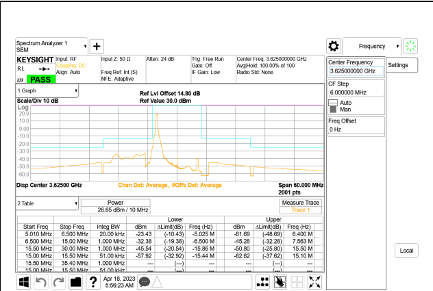
5G NR n48 10MHz BPSK Middle Channel RB1-0, ID:28567
