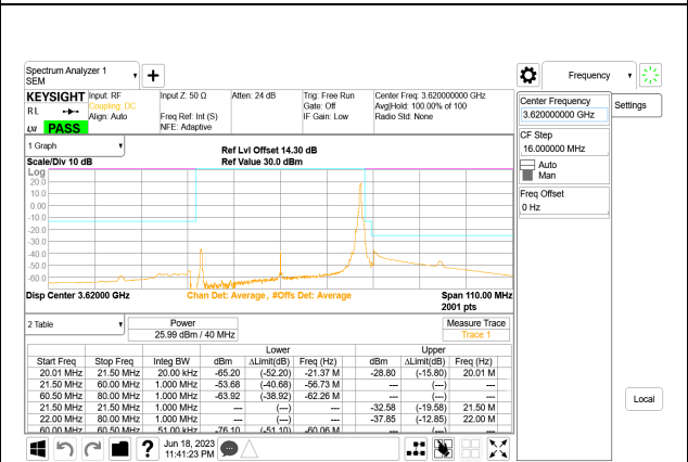
5G NR n48 40MHz BPSK Middle Channel RB1-105, ID:32586
