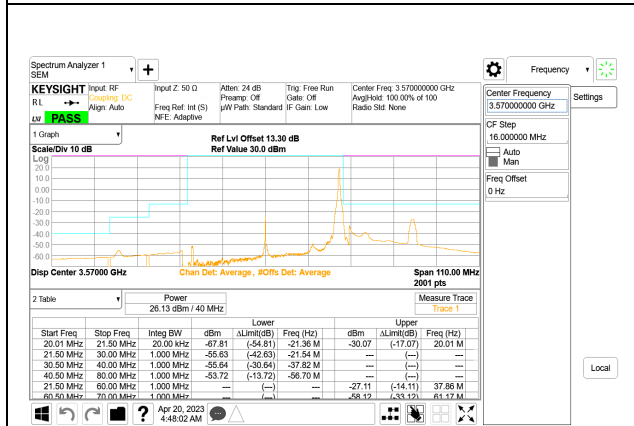
5G NR n48 40MHz BPSK Low Channel RB1-105, ID:28567
