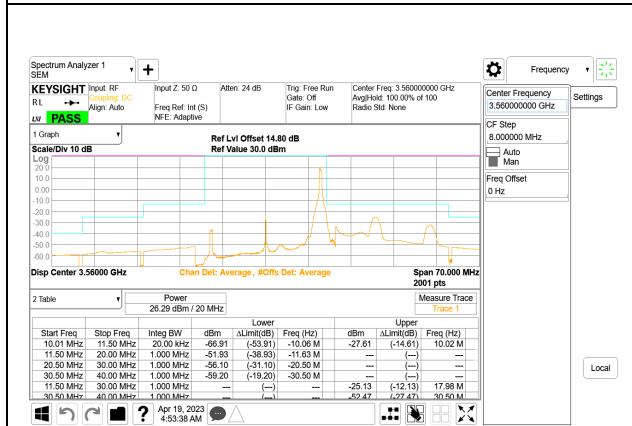
5G NR n48 20MHz BPSK Low Channel RB1-50, ID:28567
