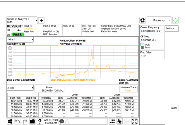
5G NR n48 20MHz BPSK Middle Channel RB1-50, ID:28567
