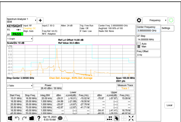
5G NR n48 30MHz BPSK Low Channel RB1-0, ID:28567
