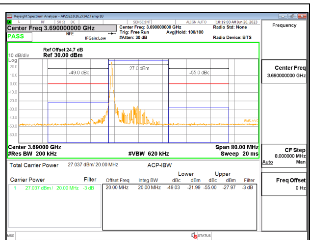
LTE B48 20MHz QPSK High Channel RB1-0
