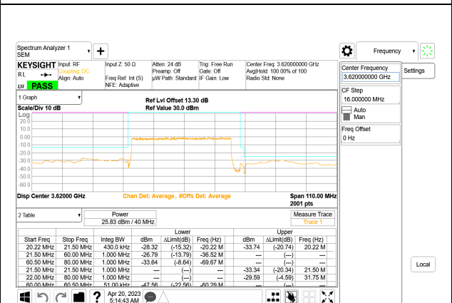
5G NR n48 40MHz BPSK Middle Channel RB100-0, ID:28567
