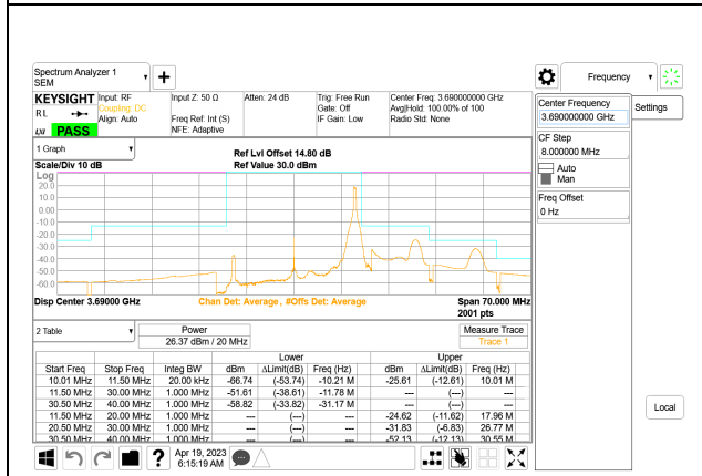
5G NR n48 20MHz BPSK High Channel RB1-50, ID:28567
