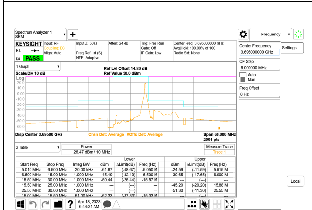
5G NR n48 10MHz BPSK High Channel RB1-23, ID:28567
