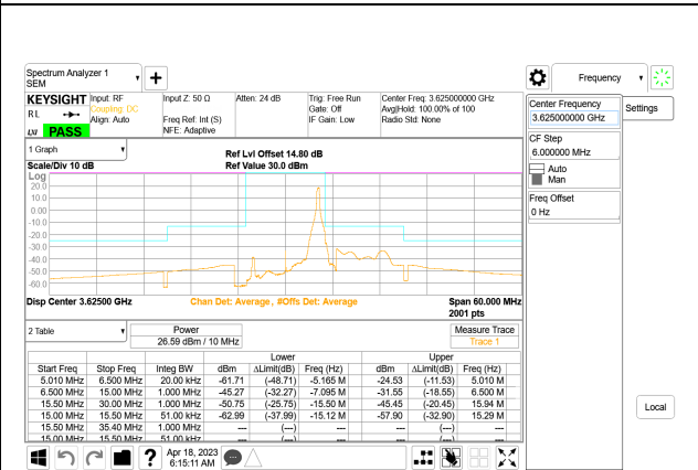
5G NR n48 10MHz BPSK Middle Channel RB1-23, ID:28567
