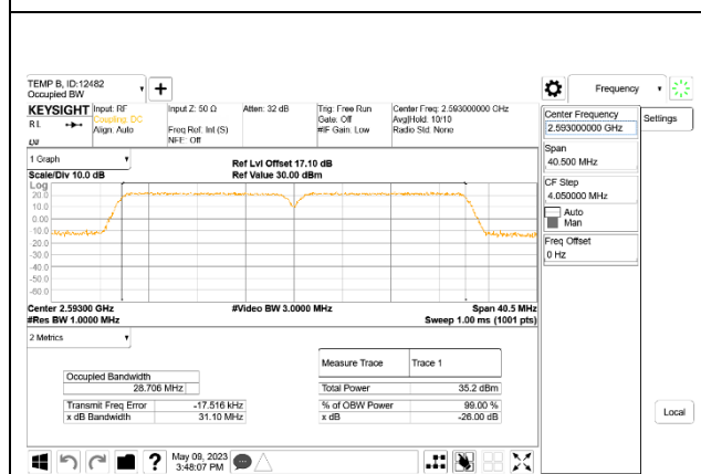
LTE B41 15MHz + 15MHz QPSK RB75-0 + RB75-0
