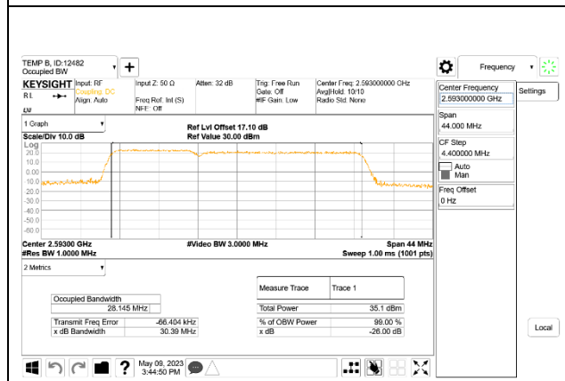
LTE B41 10MHz + 20MHz QPSK RB50-0 + RB100-0
