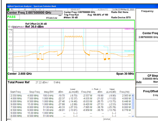
LTE B41 5MHz QPSK High Channel RB25-0, ID:25780
