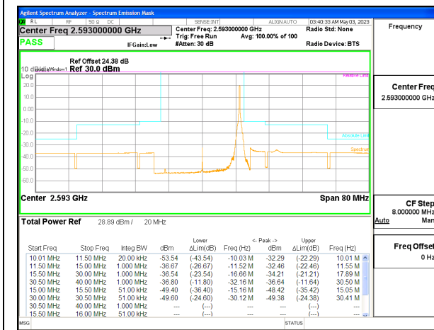
LTE B41 20MHz QPSK Middle Channel RB1-99, ID:25780
