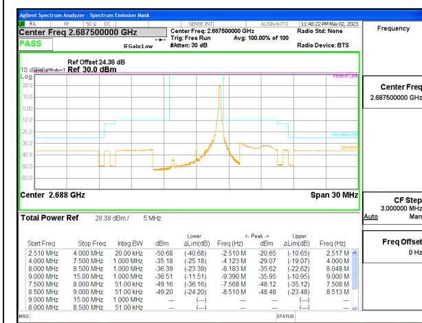
LTE B41 5MHz QPSK High Channel RB1-24, ID:25780
