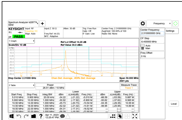
LTE B30 10MHz QPSK Middle Channel RB1-0
