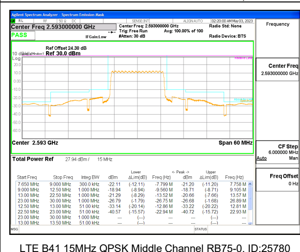
LTE B41 15MHz QPSK Middle Channel RB75-0, ID:25780
