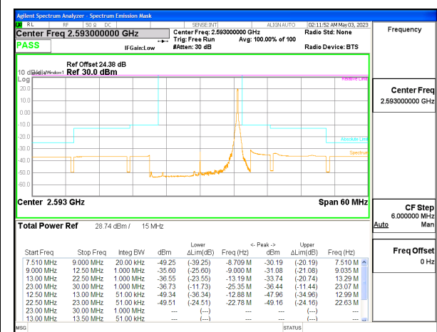
LTE B41 15MHz QPSK Middle Channel RB1-74, ID:25780
