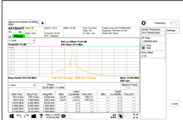
LTE B26 1.4MHz QPSK Low Channel RB1-0
