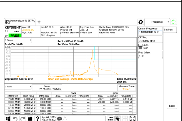
LTE B25 15MHz QPSK High Channel RB1-74
