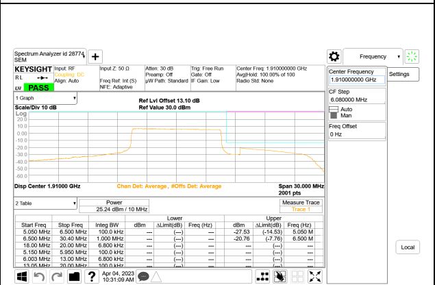
LTE B25 10MHz QPSK High Channel RB50-0
