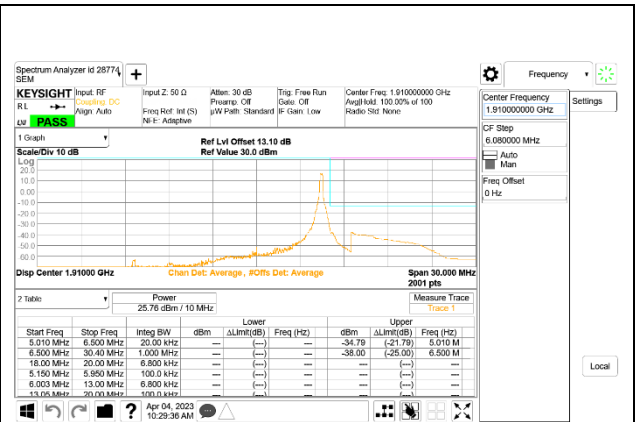
LTE B25 10MHz QPSK High Channel RB1-49
