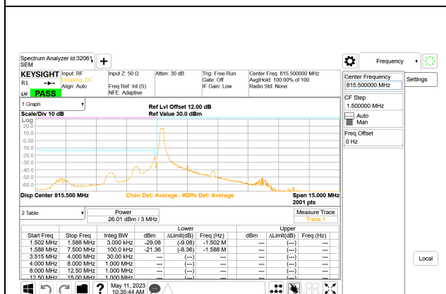
LTE B26 3MHz QPSK Low Channel RB1-0
