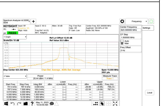
LTE B26 1.4MHz QPSK High Channel RB6-0
