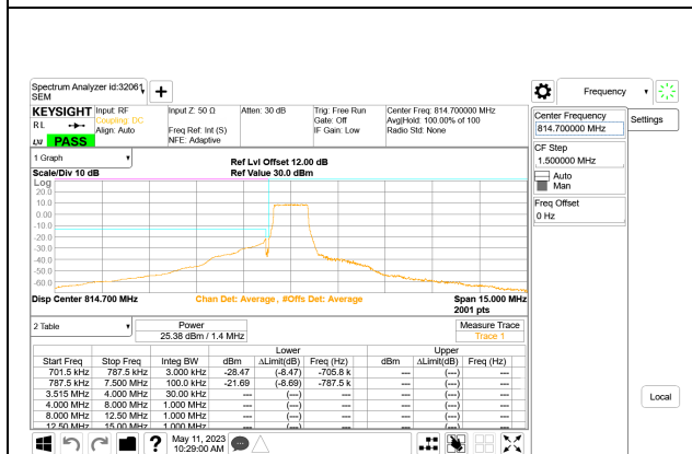
LTE B26 1.4MHz QPSK Low Channel RB6-0
