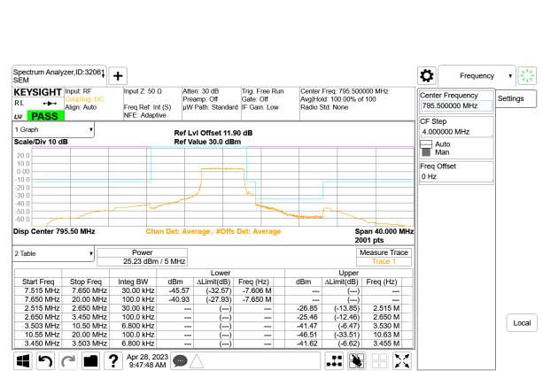
LTE B14 5MHz QPSK High Channel RB25-0
