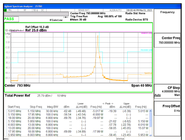
5G NR n14 10MHz BPSK Middle Channel RB1-51
