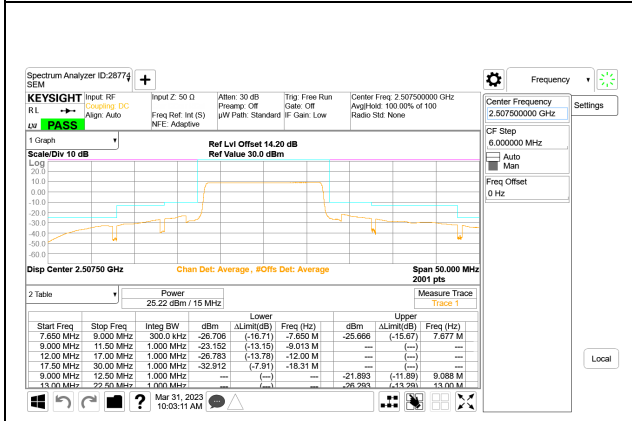
LTE B7 15MHz QPSK Low Channel RB75-0
