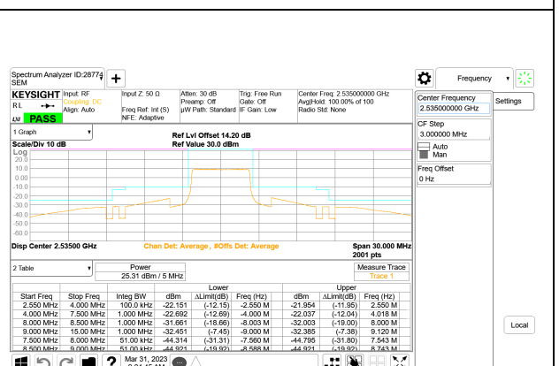
LTE B7 5MHz QPSK Middle Channel RB25-0
