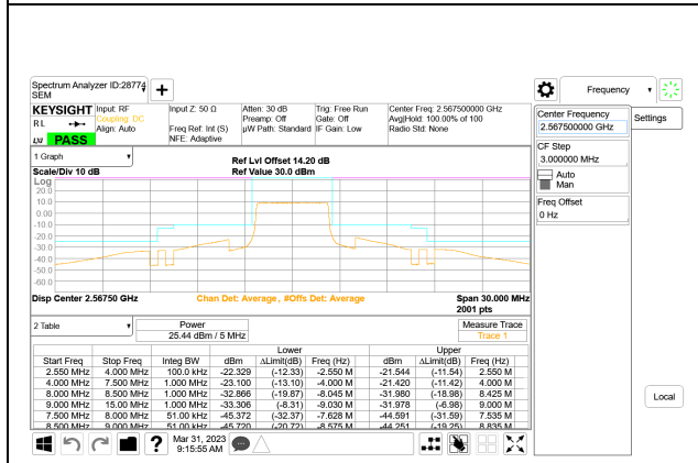
LTE B7 5MHz QPSK High Channel RB25-0
