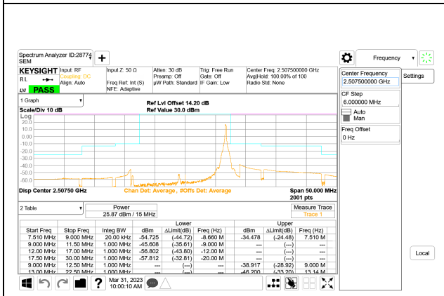
LTE B7 15MHz QPSK Low Channel RB1-74
