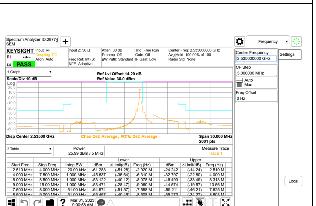
LTE B7 5MHz QPSK Middle Channel RB1-24
