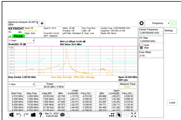
LTE B7 5MHz QPSK High Channel RB1-0
