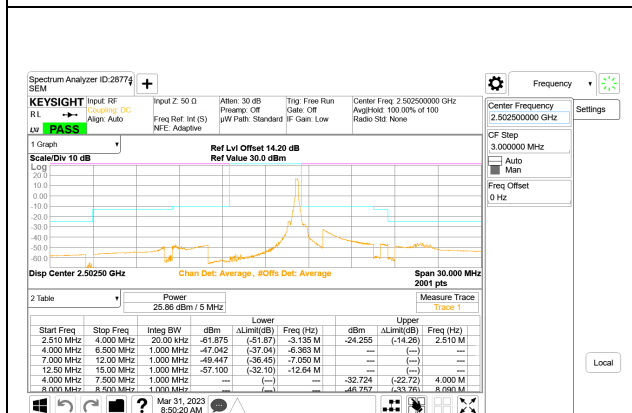
LTE B7 5MHz QPSK Low Channel RB1-24
