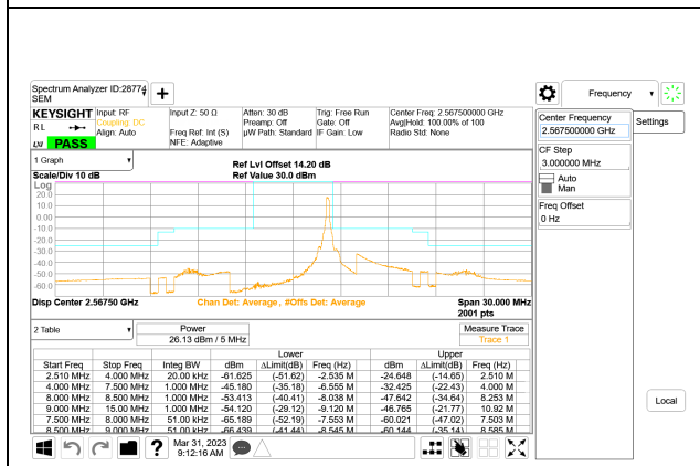
LTE B7 5MHz QPSK High Channel RB1-24
