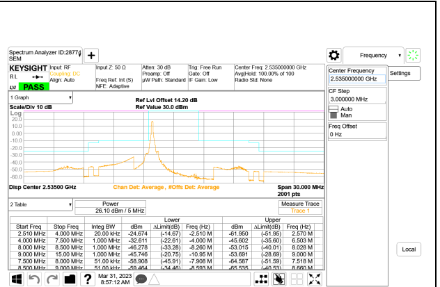
LTE B7 5MHz QPSK Middle Channel RB1-0
