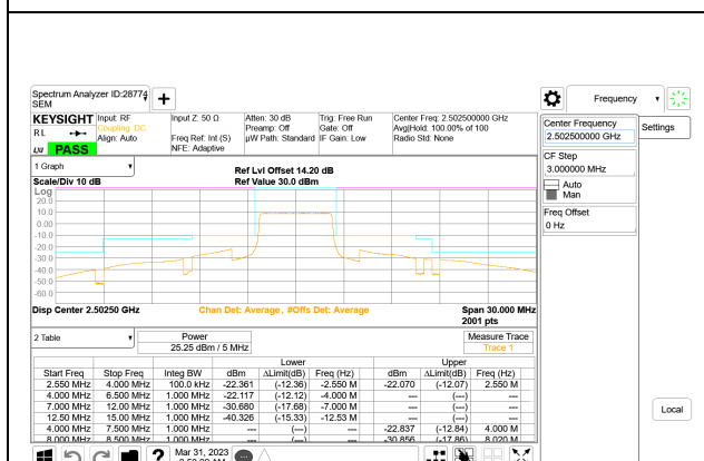
LTE B7 5MHz QPSK Low Channel RB25-0
