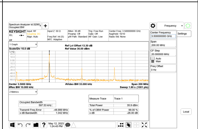
5G NR n77 100MHz BPSK Middle Channel RB1-0
