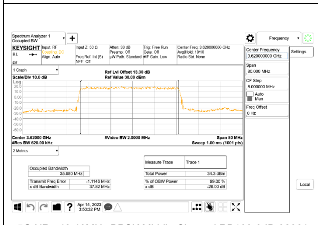
5G NR n48 40MHz BPSK Middle Channel RB100-0 ID:32061
