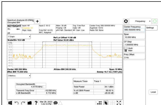
5G NR n71 5MHz BPSK Middle Channel RB25-0
