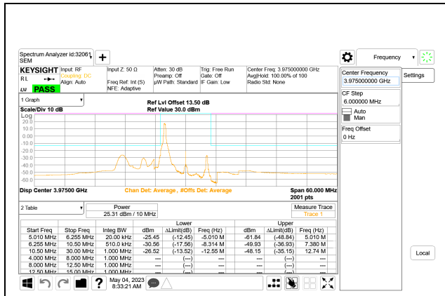
5G NR n77 10MHz BPSK High Channel RB1-0
