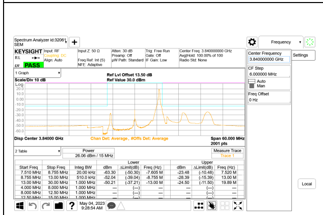
5G NR n77 15MHz BPSK Middle Channel RB1-37
