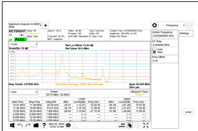
5G NR n77 20MHz BPSK High Channel RB1-0
