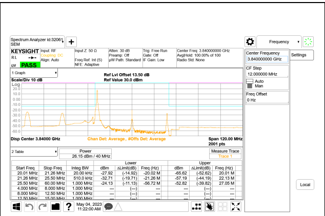
5G NR n77 40MHz BPSK Middle Channel RB1-0
