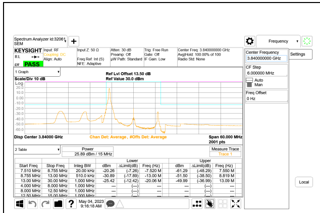
5G NR n77 15MHz BPSK Middle Channel RB1-0
