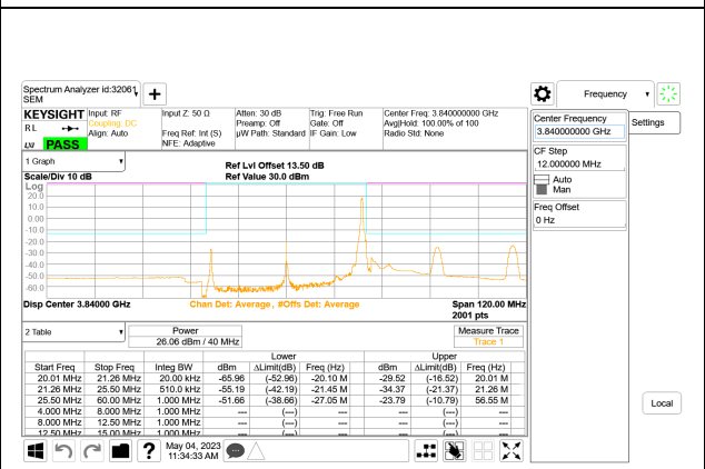
5G NR n77 40MHz BPSK Middle Channel RB1-105
