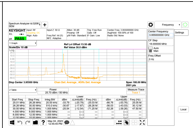
5G NR n77 50MHz BPSK High Channel RB1-0
