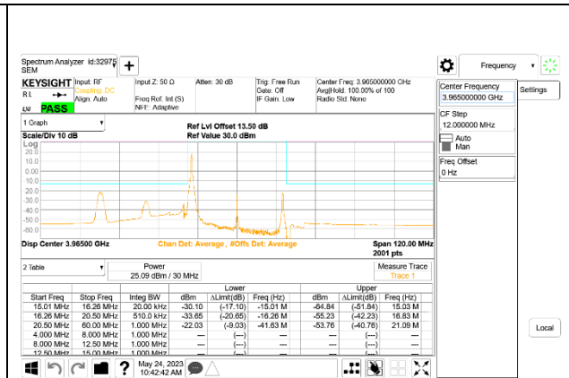
5G NR n77 30MHz BPSK High Channel RB1-0
