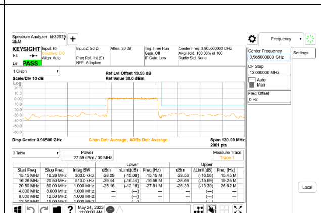
5G NR n77 30MHz BPSK High Channel RB75-0
