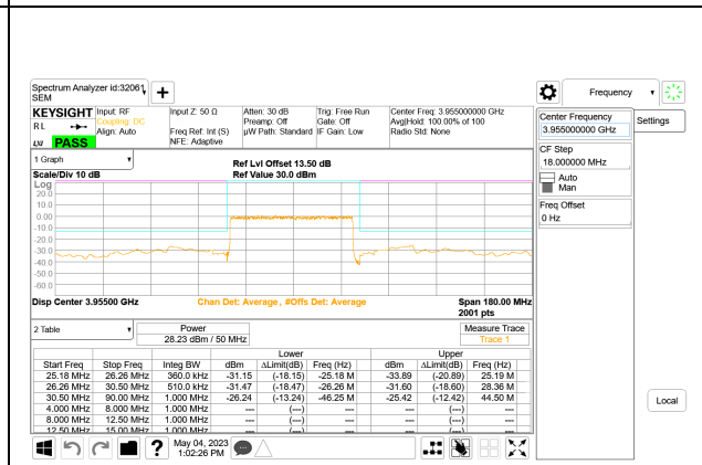
5G NR n77 50MHz BPSK High Channel RB128-0
