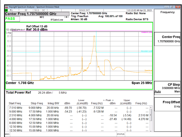
5G NR n70 5MHz BPSK High Channel (Upper Block) RB1-25, ID:50822
