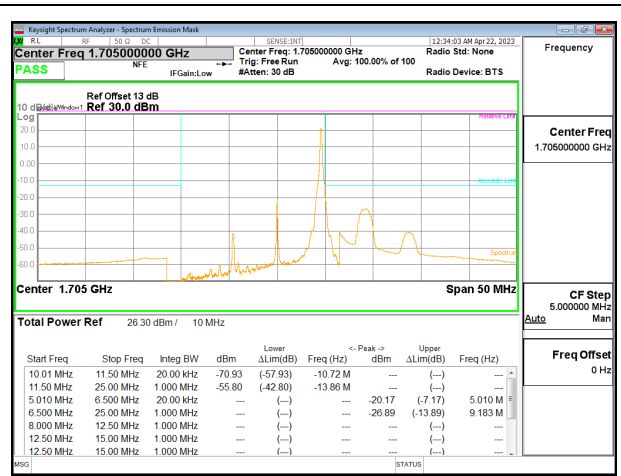
5G NR n70 10MHz BPSK High Channel (Full Block) RB1-51, ID:50822
