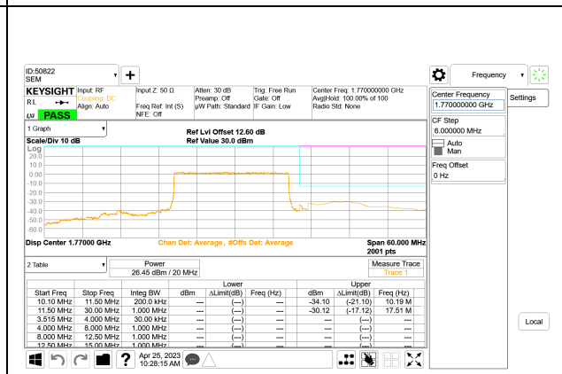
5G NR n66 20MHz BPSK High Channel RB100-0
