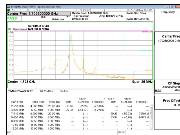
5G NR n70 5MHz BPSK Middle Channel (Upper Block) RB1-0, ID:50822
