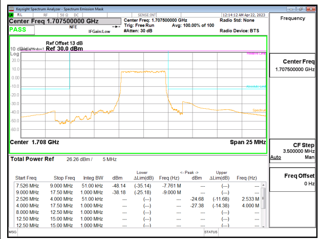
5G NR n70 5MHz BPSK High Channel (Upper Block) RB25-0, ID:50822
