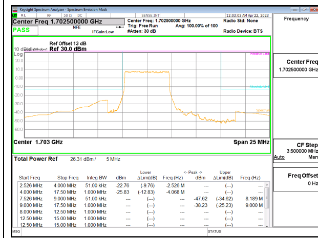
5G NR n70 5MHz BPSK Middle Channel (Upper Block) RB25-0, ID:50822
