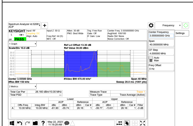
5G NR n48 10MHz BPSK Low Channel RB1-23
