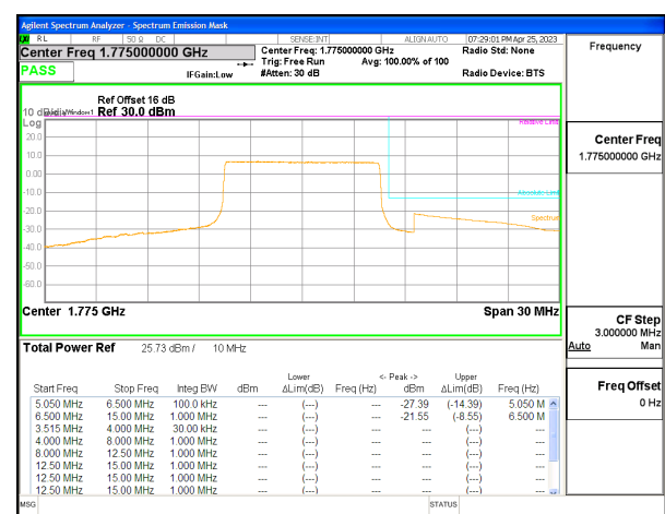
LTE B66 10MHz QPSK High Channel RB50-0, ID:25780
