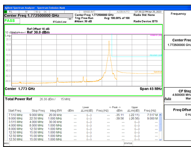
LTE B66 15MHz QPSK High Channel RB1-74, ID:25780
