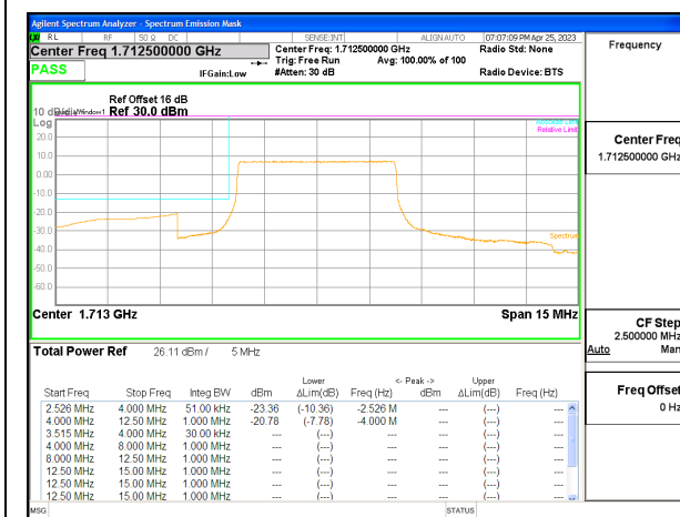
LTE B66 5MHz QPSK Low Channel RB25-0, ID:25780
