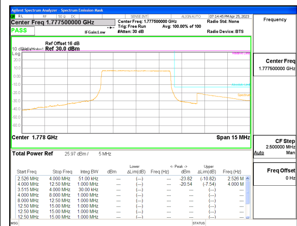
LTE B66 5MHz QPSK High Channel RB25-0, ID:25780
