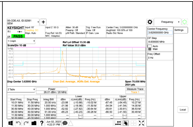
5G NR n48 20MHz BPSK Middle Channel RB1-0
