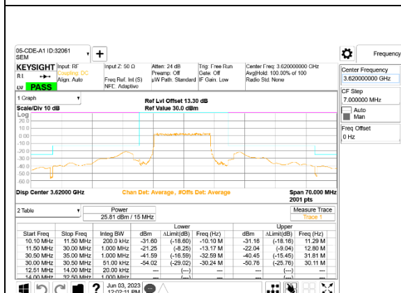
G NR n48 15MHz BPSK Middle Channel RB36-0
