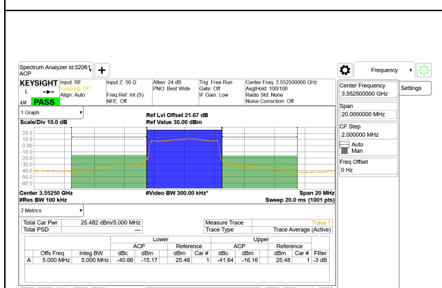
LTE B48 5MHz QPSK Low Channel RB25-0
