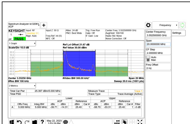
LTE B48 5MHz QPSK Low Channel RB1-0
