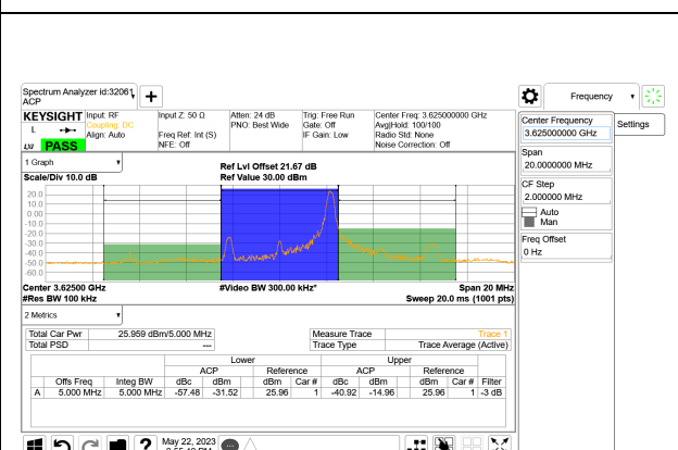
LTE B48 5MHz QPSK Middle Channel RB1-24
