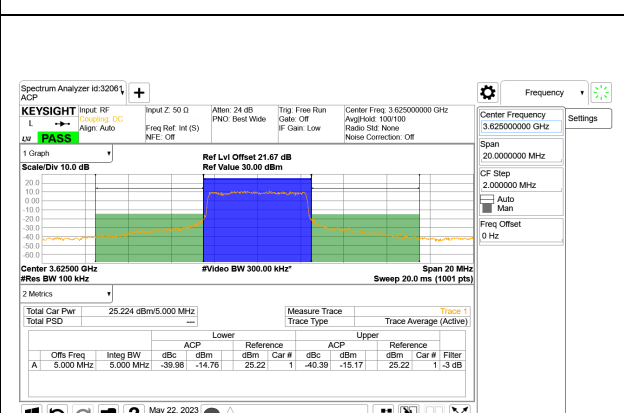
LTE B48 5MHz QPSK Middle Channel RB25-0
