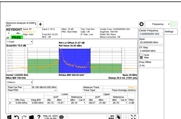
LTE B48 5MHz QPSK Middle Channel RB1-0
