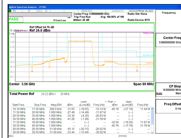
LTE B48 15MHz QPSK Low Channel RB75-0 ID:25780
