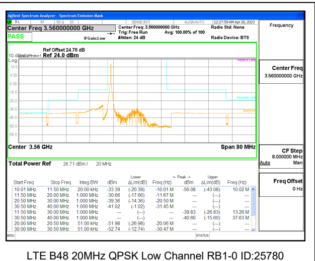
LTE B48 20MHz QPSK Low Channel RB1-0 ID:25780
