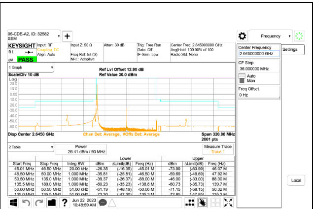
5G NR n41 90MHz BPSK High Channel RB1-0
