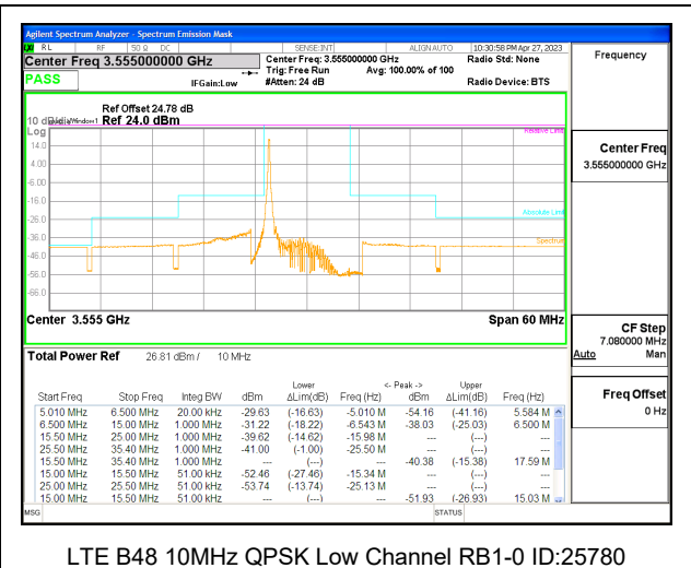
LTE B48 10MHz QPSK Low Channel RB1-0 ID:25780
