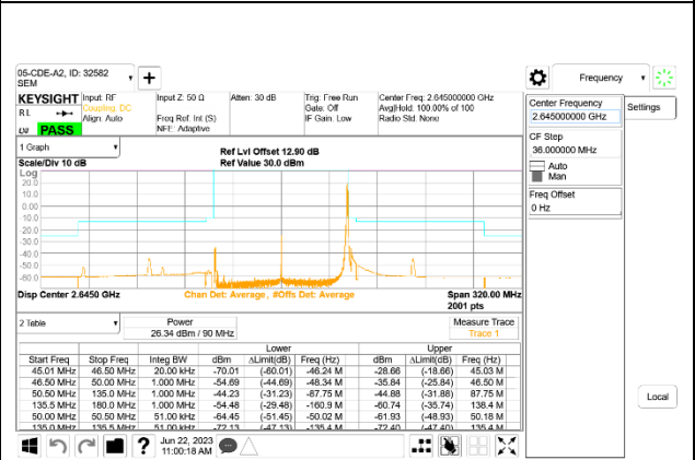
5G NR n41 90MHz BPSK High Channel RB1-244
