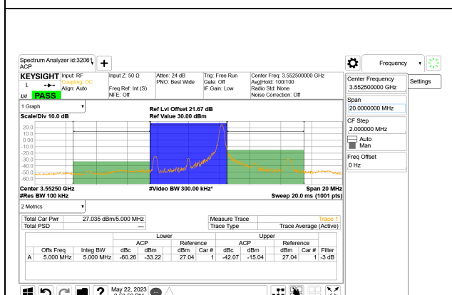
LTE B48 5MHz QPSK Low Channel RB1-24
