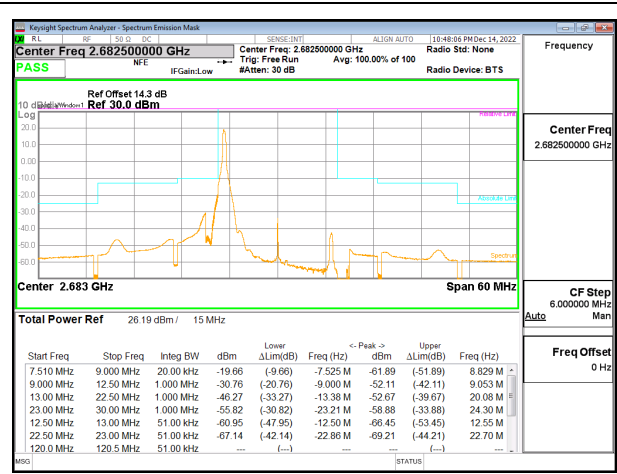
5G NR n41 15MHz BPSK High Channel RB1-0, ID:25780
