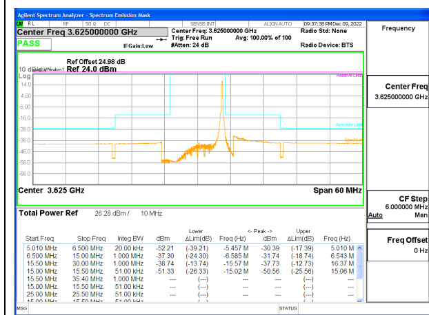
LTE B48 10MHz QPSK Middle Channel RB1-49, ID:25780
