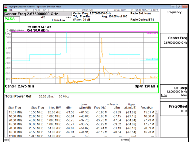
5G NR n41 30MHz BPSK High Channel RB1-77, ID:25780
