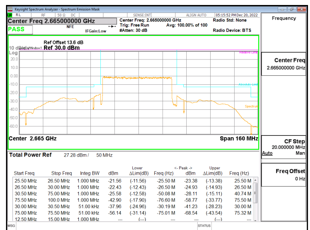
5G NR n41 50MHz BPSK High Channel RB128-0, ID:25780
