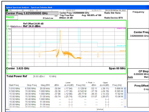
LTE B48 10MHz QPSK Middle Channel RB1-0, ID:25780
