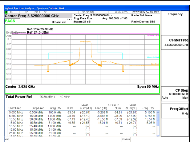
LTE B48 5MHz QPSK Middle Channel RB25-0, ID:25780
