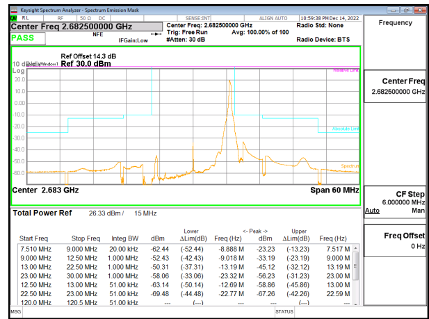
5G NR n41 15MHz BPSK High Channel RB1-37, ID:25780
