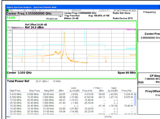
LTE B48 5MHz QPSK Low Channel RB1-0, ID:25780
