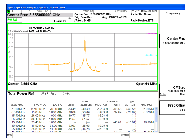
LTE B48 5MHz QPSK Low Channel RB1-24, ID:25780
