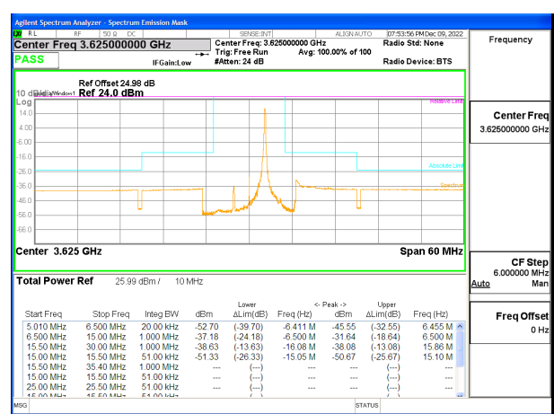
LTE B48 5MHz QPSK Middle Channel RB1-24, ID:25780
