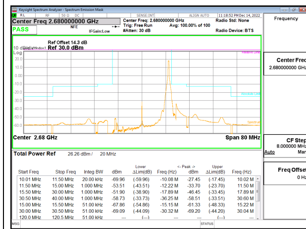
5G NR n41 20MHz BPSK High Channel RB1-50, ID:25780
