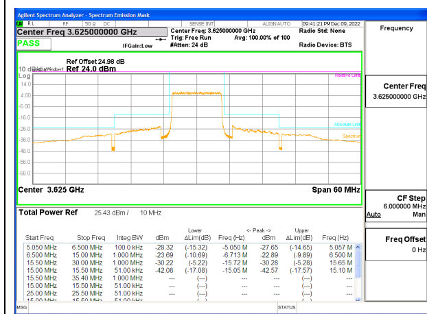
LTE B48 10MHz QPSK Middle Channel RB50-0, ID:25780
