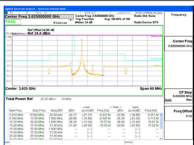
LTE B48 5MHz QPSK Middle Channel RB1-0, ID:25780
