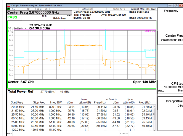
5G NR n41 40MHz BPSK High Channel RB100-0, ID:25780
