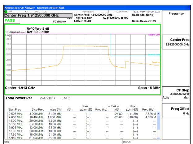
LTE B25 5MHz QPSK High Channel RB25-0, ID:25780
