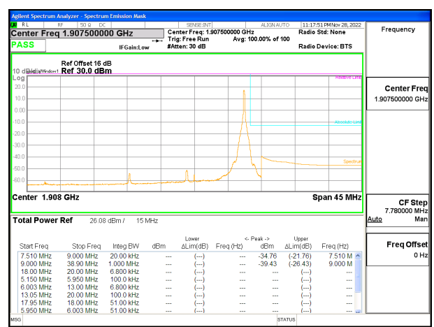
LTE B25 15MHz QPSK High Channel RB1-74, ID:25780
