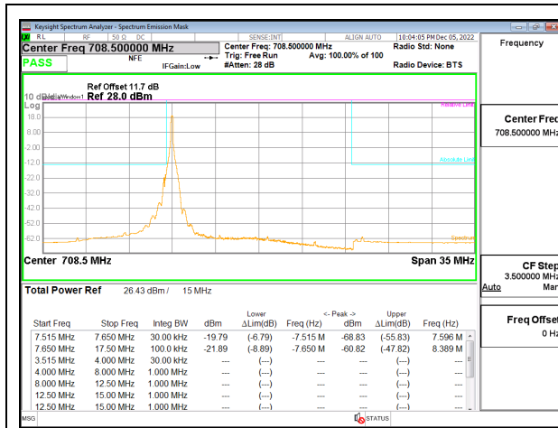
5G NR n12 15MHz BPSK High Channel RB1-0, ID:19146
