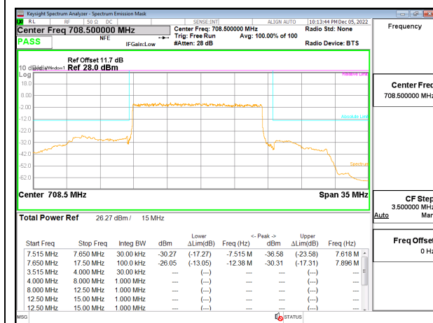
5G NR n12 15MHz BPSK High Channel RB75-0, ID:19146
