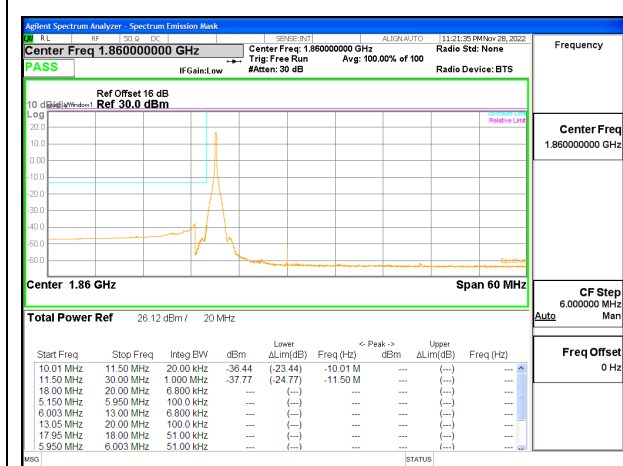
LTE B25 20MHz QPSK Low Channel RB1-0, ID:25780
