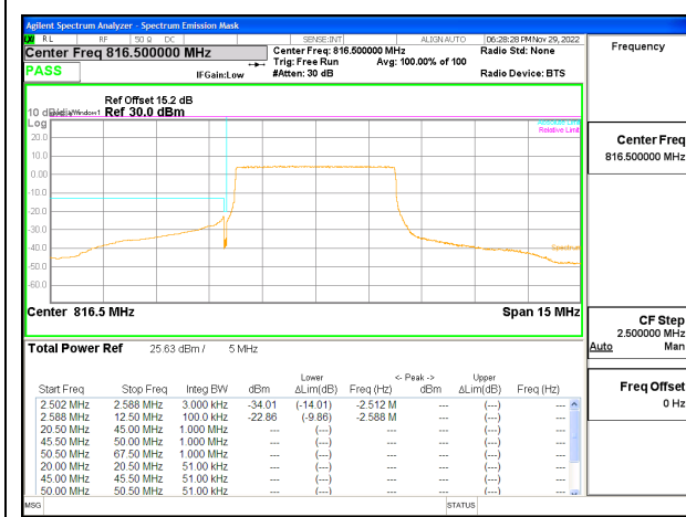
LTE B26 5MHz QPSK Low Channel RB25-0, ID:25780
