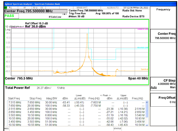
LTE B14 5MHz QPSK High Channel RB1-24, ID:25780
