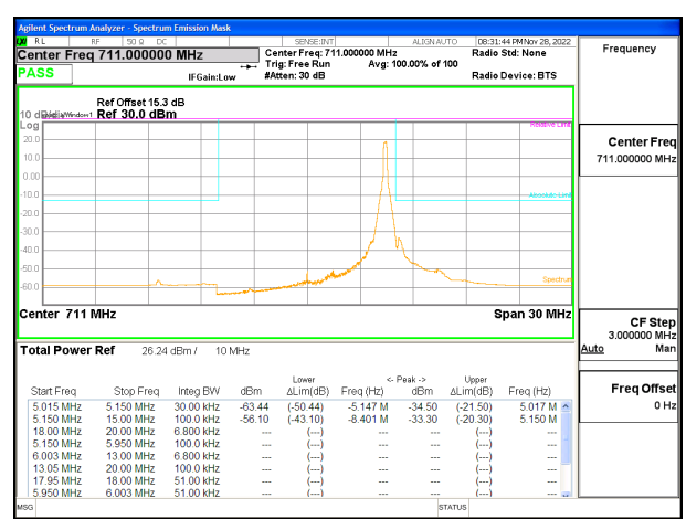
LTE B17 10MHz QPSK High Channel RB1-49, ID:25780
