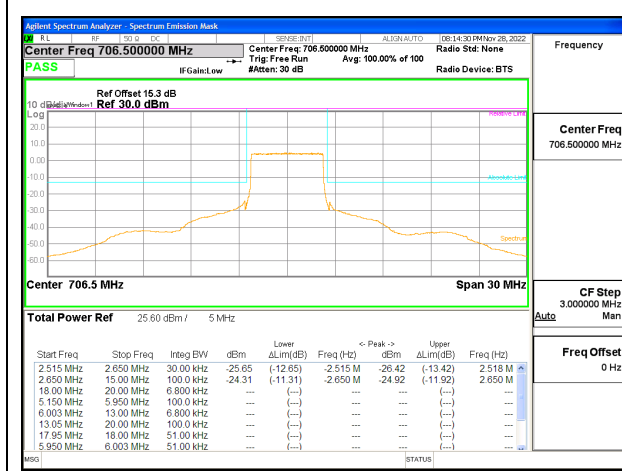
LTE B17 5MHz QPSK Low Channel RB25-0, ID:25780
