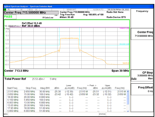
LTE B17 5MHz QPSK High Channel RB25-0, ID:25780
