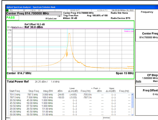
LTE B26 1.4MHz QPSK Low Channel RB1-0, ID:25780
