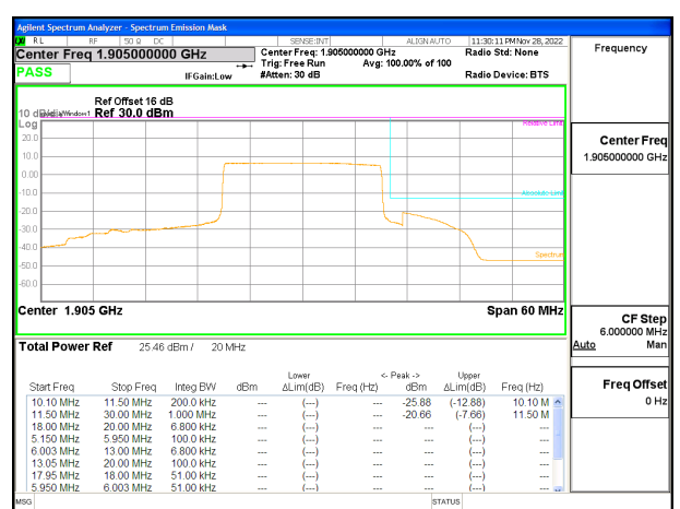
LTE B25 20MHz QPSK High Channel RB100-0, ID:25780
