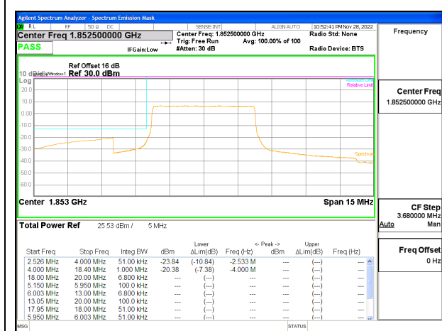
LTE B25 5MHz QPSK Low Channel RB25-0, ID:25780
