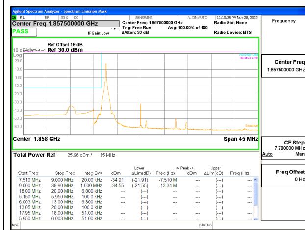
LTE B25 15MHz QPSK Low Channel RB1-0, ID:25780
