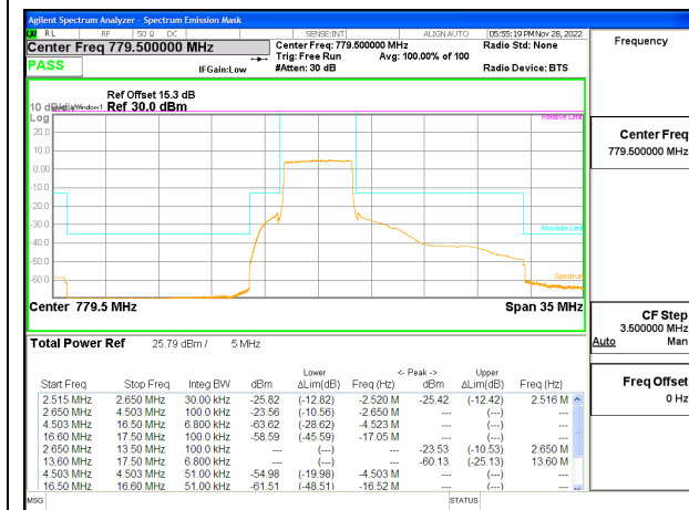
LTE B13 5MHz QPSK Low Channel RB25-0, ID:25780
