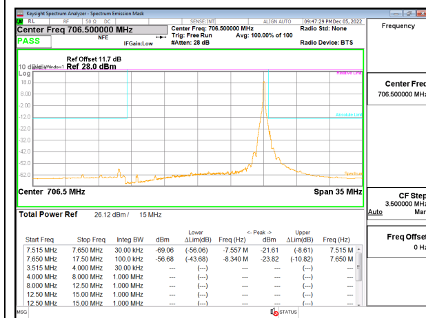
5G NR n12 15MHz BPSK Low Channel RB1-78, ID:19146
