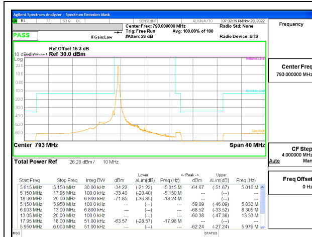
LTE B14 10MHz QPSK Middle Channel RB1-0, ID:25780
