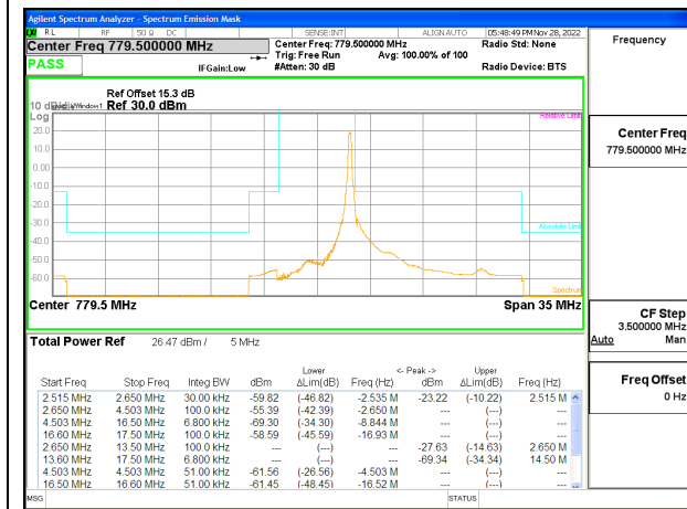
LTE B13 5MHz QPSK Low Channel RB1-24, ID:25780
