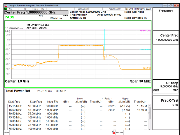
5G NR n25 30MHz BPSK High Channel RB160-0, ID:19146
