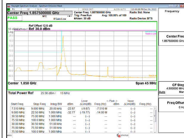
5G NR n25 15MHz BPSK Low Channel RB1-0, ID:19146
