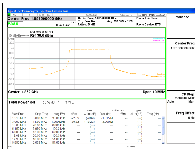
LTE B25 3MHz QPSK Low Channel RB15-0, ID:25780
