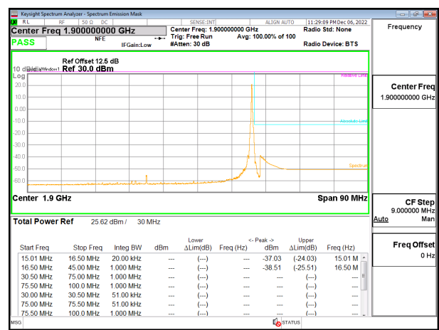
5G NR n25 30MHz BPSK High Channel RB1-159, ID:19146
