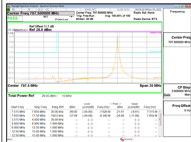
5G NR n12 15MHz BPSK Middle Channel RB1-78, ID:19146
