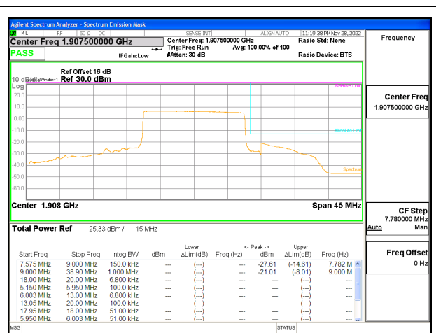
LTE B25 15MHz QPSK High Channel RB75-0, ID:25780
