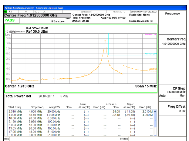
LTE B25 5MHz QPSK High Channel RB1-24, ID:25780
