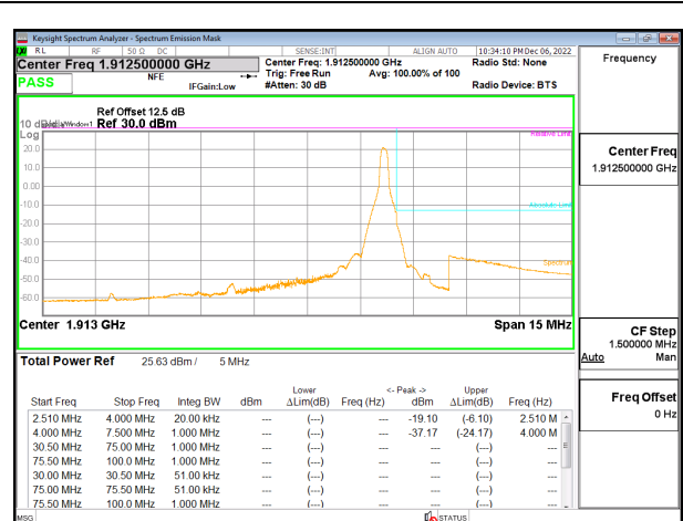
5G NR n25 5MHz BPSK High Channel RB1-24, ID:19146
