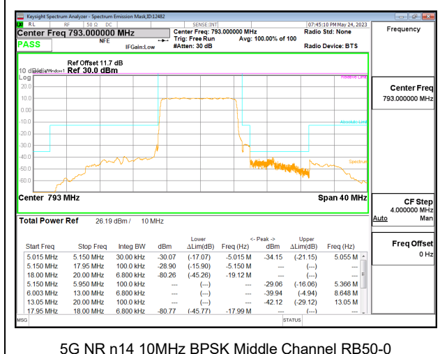
5G NR n14 10MHz BPSK Middle Channel RB50-0
