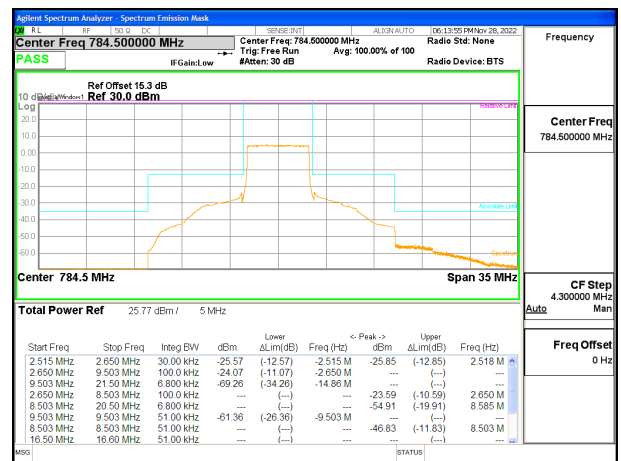
LTE B13 5MHz QPSK High Channel RB25-0, ID:25780
