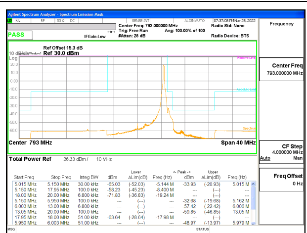
LTE B14 10MHz QPSK Middle Channel RB1-49, ID:25780
