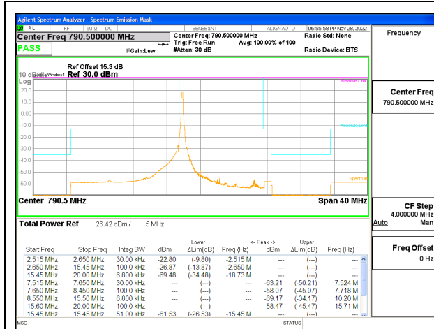
LTE B14 5MHz QPSK Low Channel RB1-0, ID:25780
