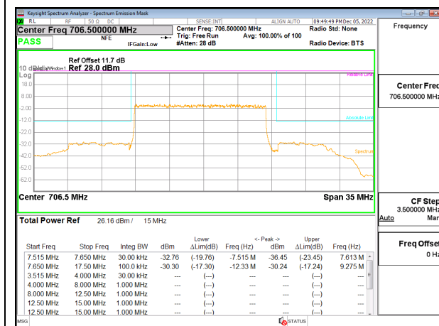
5G NR n12 15MHz BPSK Low Channel RB75-0, ID:19146
