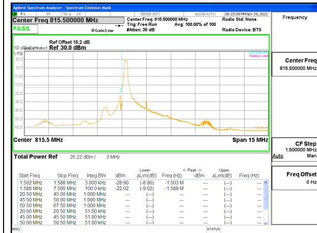
LTE B26 3MHz QPSK Low Channel RB1-0, ID:25780
