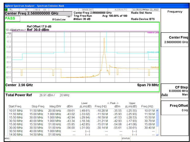
LTE B7 20MHz QPSK High Channel RB1-99, ID:25780
