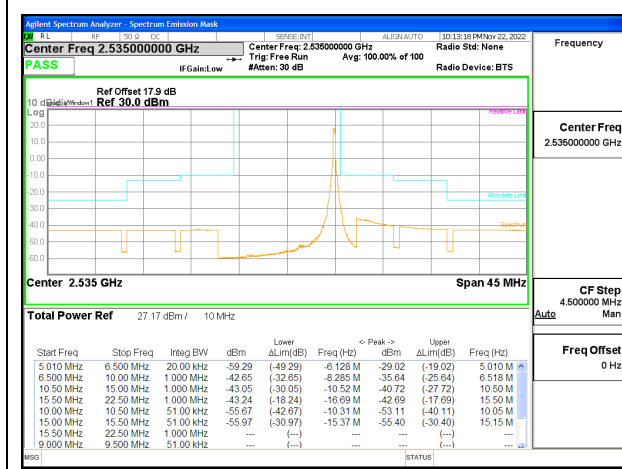
LTE B7 10MHz QPSK Middle Channel RB1-49, ID:25780
