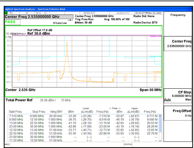
LTE B7 15MHz QPSK Middle Channel RB1-0, ID:25780
