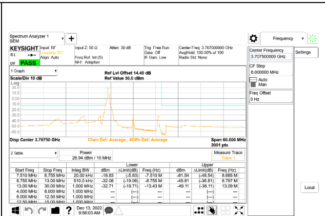
5G NR n77 15MHz BPSK Low Channel RB1-0, ID:50822
