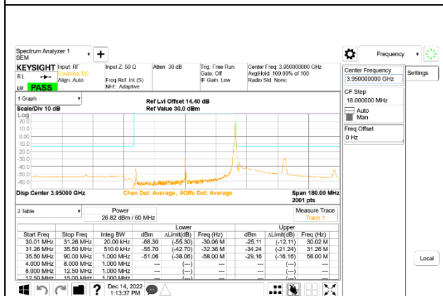
5G NR n77 60MHz BPSK High Channel RB1-161, ID:50822
