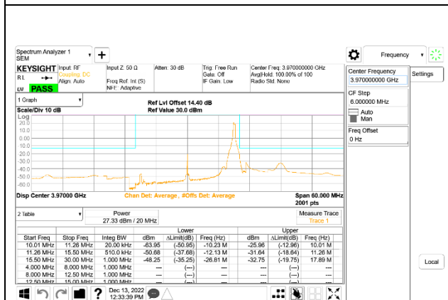
5G NR n77 20MHz BPSK High Channel RB1-50, ID:50822
