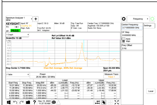
5G NR n77 20MHz BPSK Low Channel RB1-50, ID:50822
