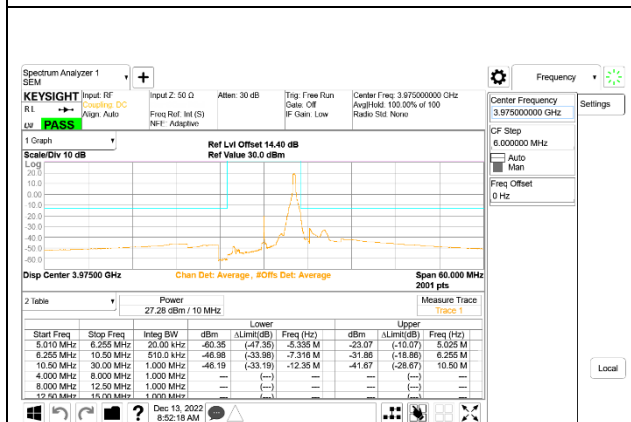
5G NR n77 10MHz BPSK High Channel RB1-23, ID:50822
