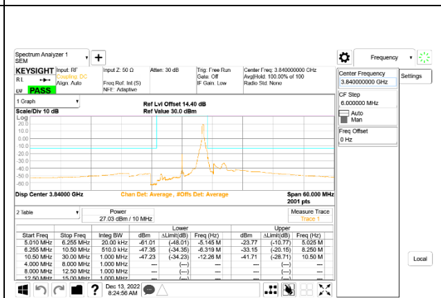
5G NR n77 10MHz BPSK Middle Channel RB1-23, ID:50822
