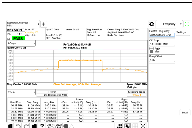
5G NR n77 60MHz BPSK High Channel RB162-0, ID:50822
