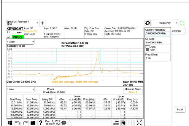
5G NR n77 20MHz BPSK Middle Channel RB1-50, ID:50822
