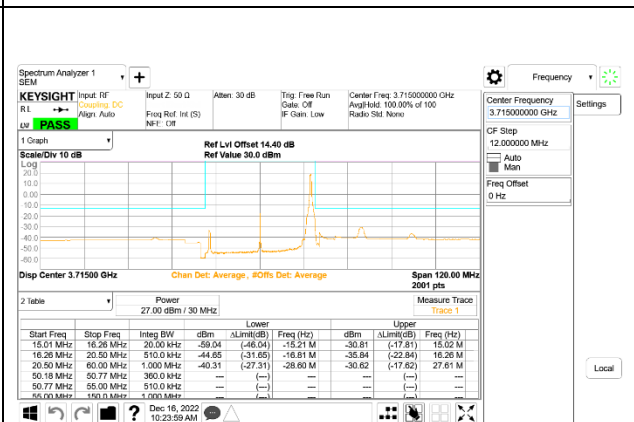
5G NR n77 30MHz BPSK Low Channel RB1-77, ID:50822
