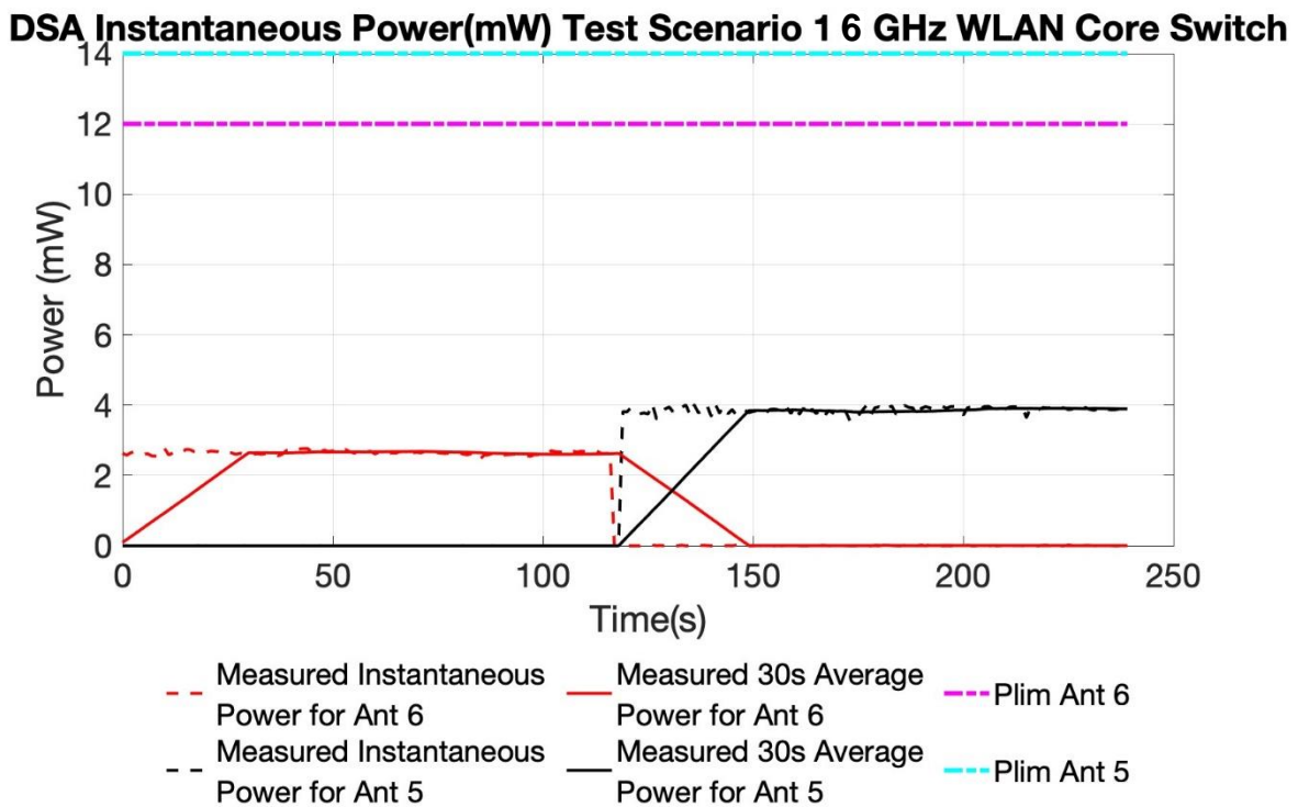
Figure 8: 30 second Average Power vs Time, 6GHz
