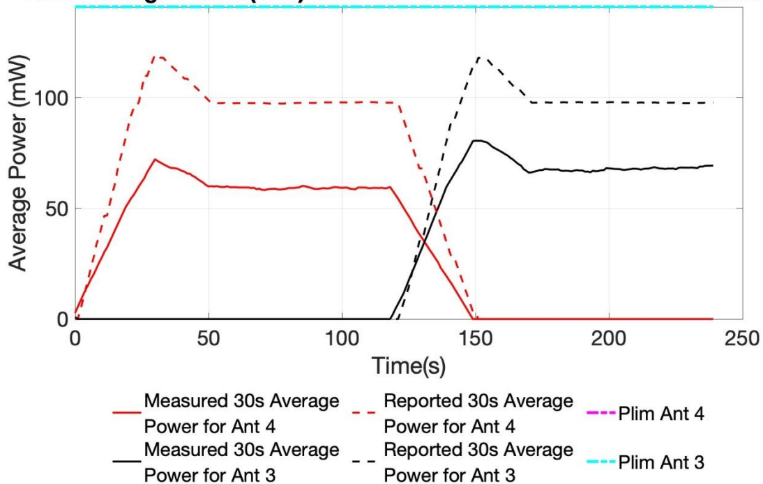
Figure 2: 30 second Average Power vs Time, 2.4GHz
