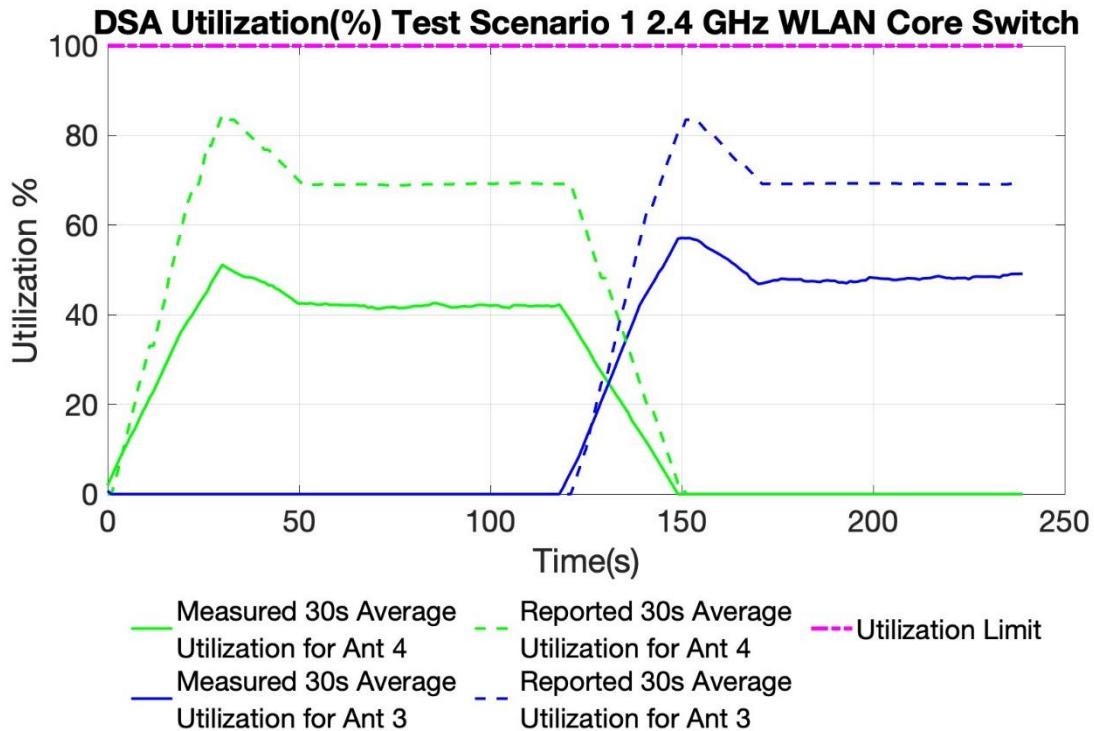
Figure 1: 30 second Aggregated SAR Utilization vs Time, 2.4GHz
