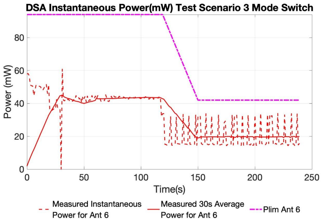
Figure 14: 30 second Average Power vs Time during Mode Switch
