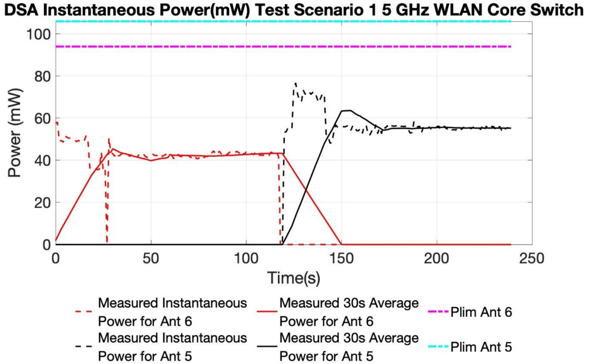
Figure 5: 30 second Average Power vs Time, 5GHz
