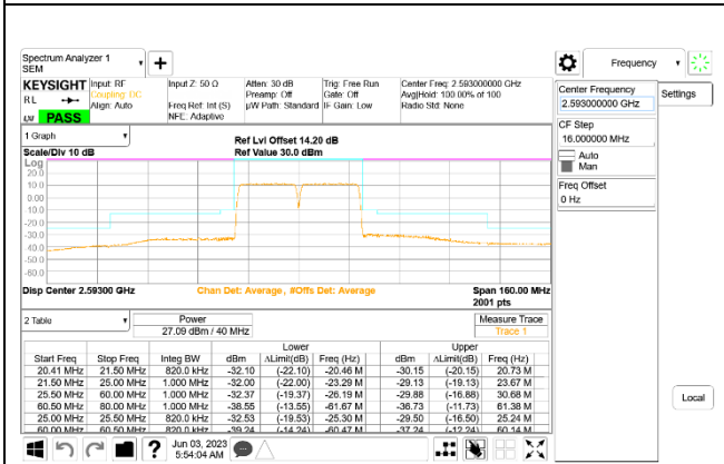
LTE B41 20MHz + 20MHz QPSK Mid Ch RB100-0 + RB100-0 ID:27342
