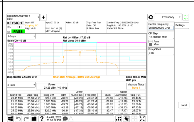
LTE B7 20MHz + 20MHz 16QAM High Ch RB100-0 + RB100-0 ID:27342
