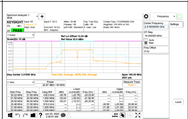
LTE B41 20MHz + 20MHz 16QAM Low Ch RB100-0 + RB100-0 ID:27342
