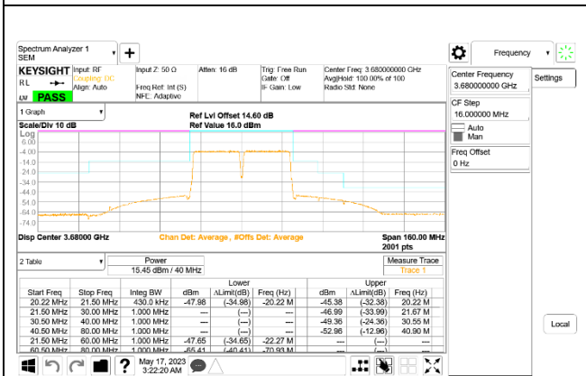
LTE B48 20MHz + 20MHz QPSK High Ch RB100-0 + RB100-0 ID:27342
