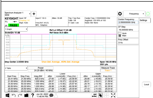
LTE B7 20MHz + 20MHz QPSK High Ch RB100-0 + RB100-0 ID:27342
