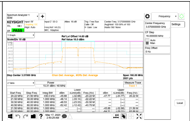
LTE B48 20MHz + 20MHz 16QAM Low Ch RB100-0 + RB100-0 ID:27342
