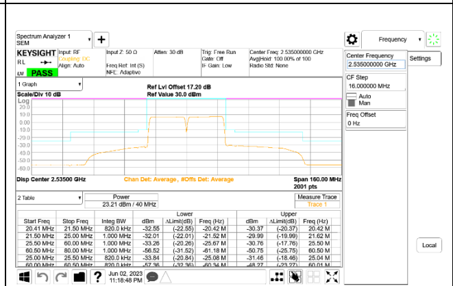
LTE B7 20MHz + 20MHz 16QAM Mid Ch RB100-0 + RB100-0 ID:27342
