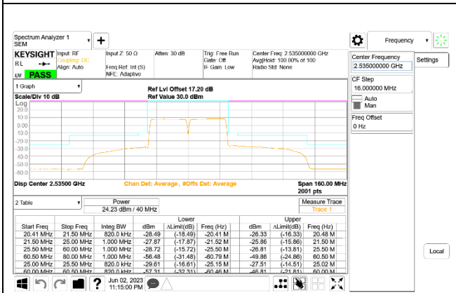
LTE B7 20MHz + 20MHz QPSK Mid Ch RB100-0 + RB100-0 ID:27342
