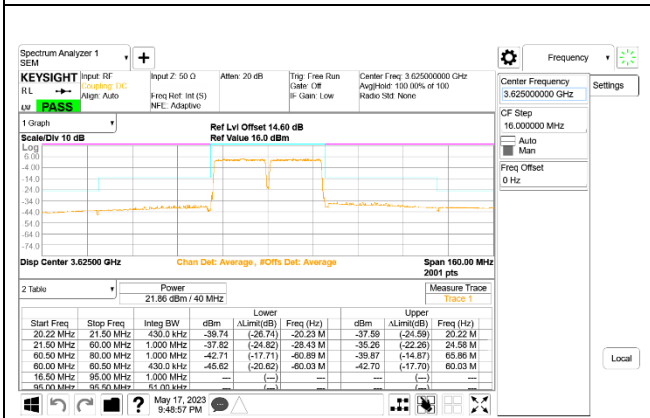
LTE B48 20MHz + 20MHz QPSK Mid Ch RB100-0 + RB100-0 ID:27342
