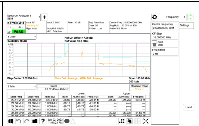
LTE B7 20MHz + 20MHz 16QAM Low Ch RB100-0 + RB100-0 ID:27342
