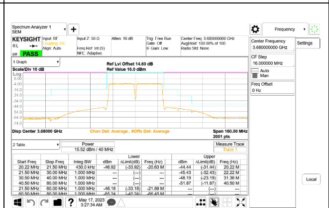
LTE B48 20MHz + 20MHz 16QAM High Ch RB100-0 + RB100-0 ID:27342
