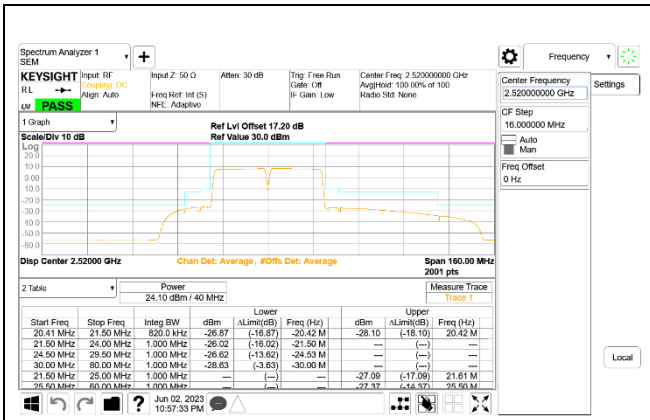
LTE B7 20MHz + 20MHz QPSK Low Ch RB100-0 + RB100-0 ID:27342
