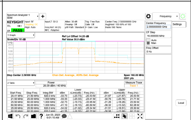
LTE B41 20MHz + 20MHz 16QAM Mid Ch RB100-0 + RB100-0 ID:27342
