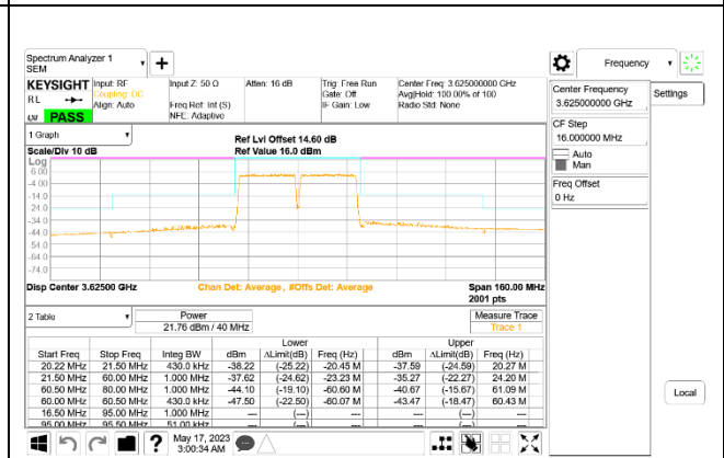
LTE B48 20MHz + 20MHz 16QAM Mid Ch RB100-0 + RB100-0 ID:27342
