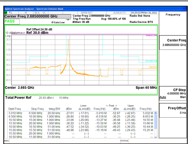
LTE B41 10MHz QPSK High Channel RB1-0 ID:19210
