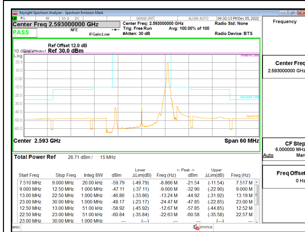
5G NR n41 15MHz BPSK Middle Channel RB1-37 ID:28498
