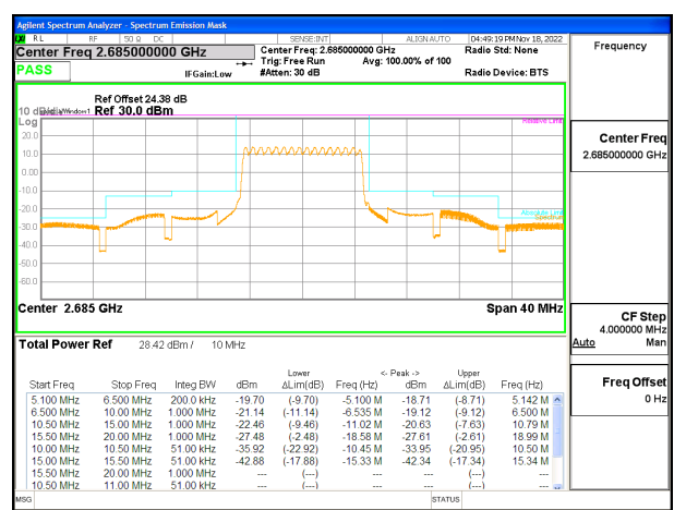
LTE B41 10MHz QPSK High Channel RB50-0 ID:19210
