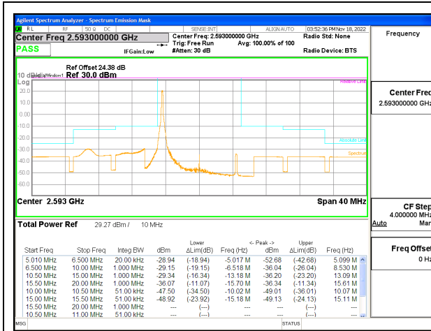
LTE B41 10MHz QPSK Middle Channel RB1-0 ID:19210
