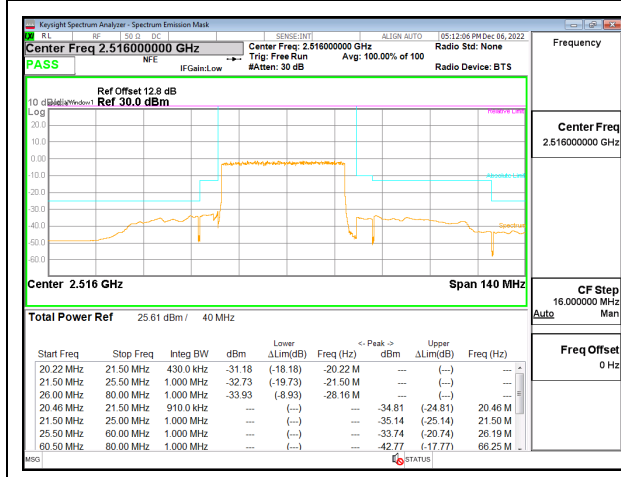
5G NR n41 40MHz BPSK Low Channel RB100-0 ID:28498
