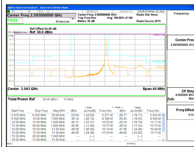
LTE B41 10MHz QPSK Middle Channel RB1-49 ID:19210
