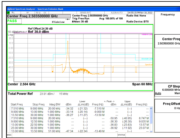
LTE B41 15MHz QPSK Low Channel RB1-0 ID:19210
