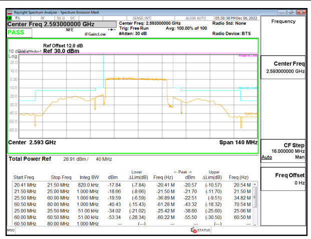
5G NR n41 40MHz BPSK Middle Channel RB100-0 ID:28498
