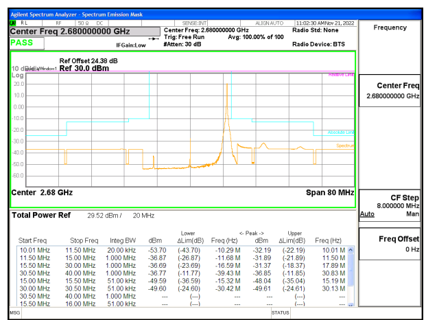
LTE B41 20MHz QPSK High Channel RB1-99 ID:19210
