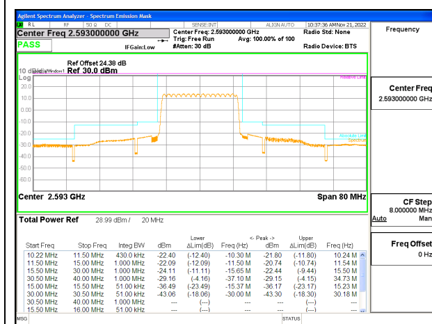
LTE B41 20MHz QPSK Middle Channel RB100-0 ID:19210
