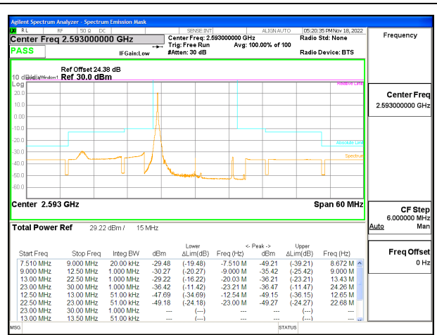
LTE B41 15MHz QPSK Middle Channel RB1-0 ID:19210
