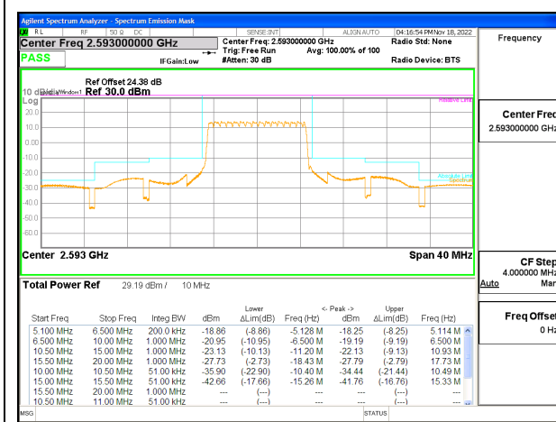
LTE B41 10MHz QPSK Middle Channel RB50-0 ID:19210
