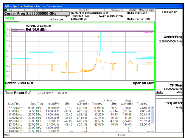
LTE B41 15MHz QPSK Middle Channel RB1-74 ID:19210
