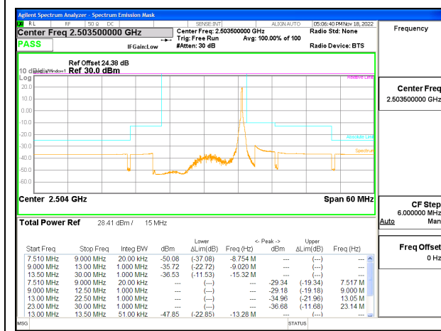
LTE B41 15MHz QPSK Low Channel RB1-74 ID:19210
