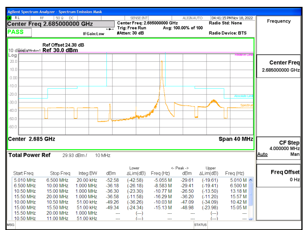
LTE B41 10MHz QPSK High Channel RB1-49 ID:19210
