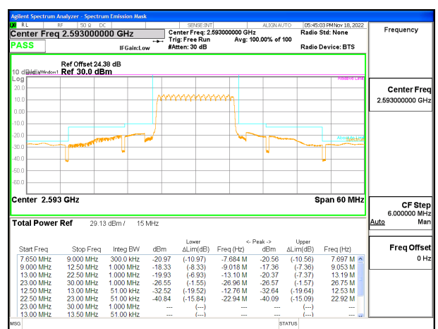
LTE B41 15MHz QPSK Middle Channel RB75-0 ID:19210
