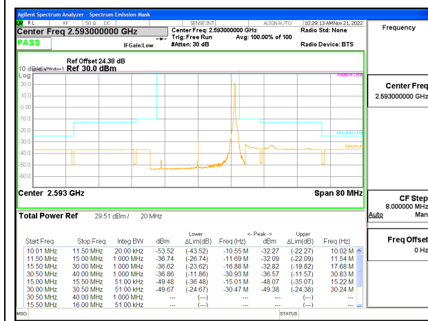
LTE B41 20MHz QPSK Middle Channel RB1-99 ID:19210
