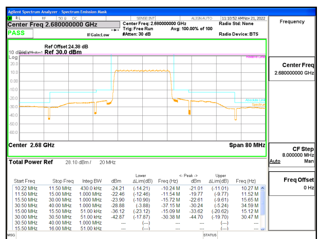
LTE B41 20MHz QPSK High Channel RB100-0 ID:19210
