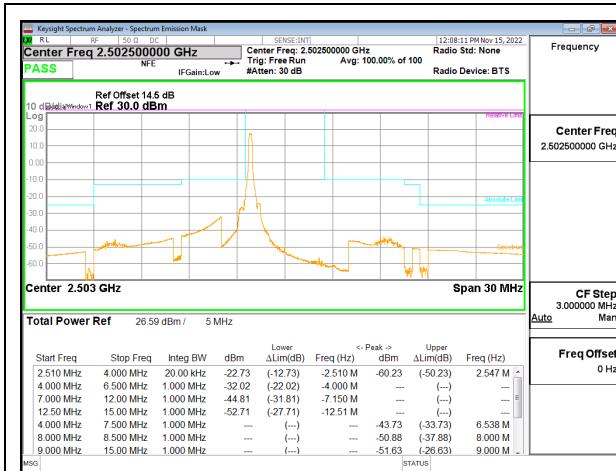
LTE B7 5MHz QPSK Low Channel RB1-0, ID:27342
