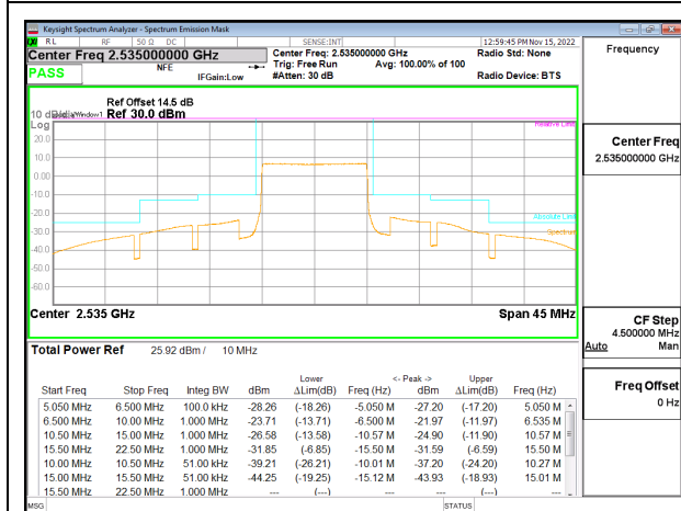
LTE B7 10MHz QPSK Middle Channel RB50-0, ID:27342
