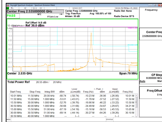
LTE B7 20MHz QPSK Middle Channel RB1-99, ID:27342
