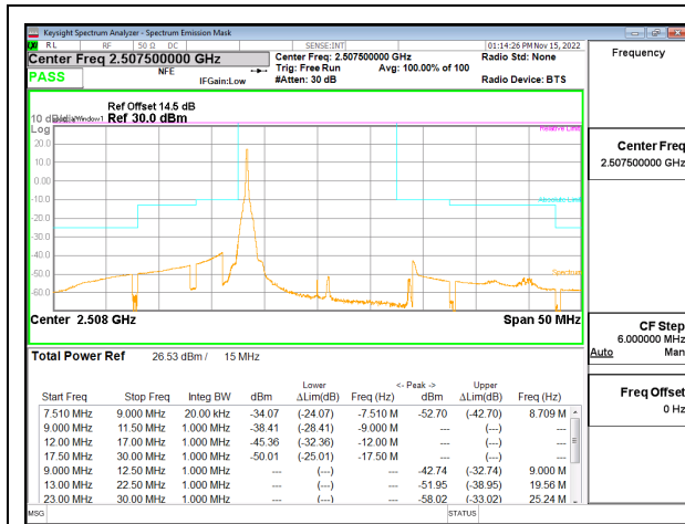
LTE B7 15MHz QPSK Low Channel RB1-0, ID:27342
