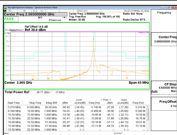
LTE B7 10MHz QPSK High Channel RB1-49, ID:27342
