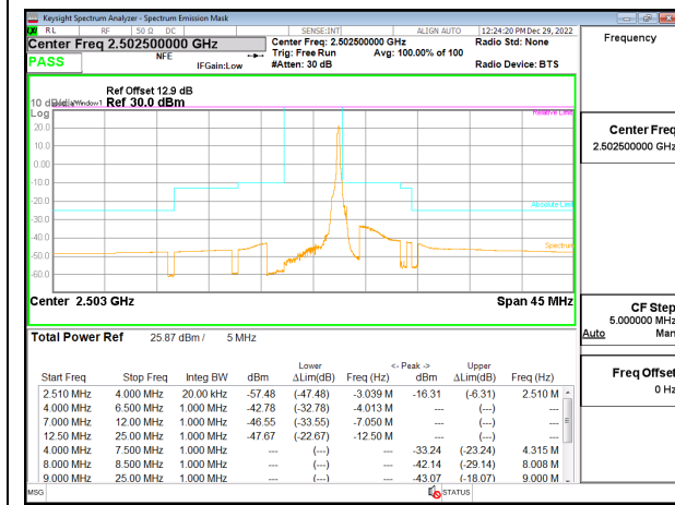
5G NR n7 5MHz BPSK Low Channel RB1-24, ID:28568
