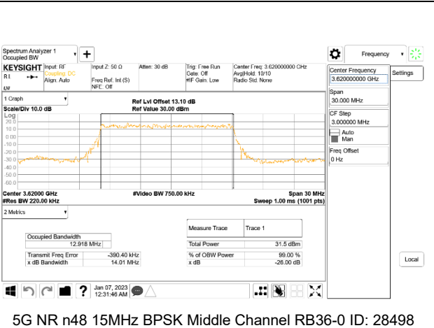
5G NR n48 15MHz BPSK Middle Channel RB36-0 ID: 28498
