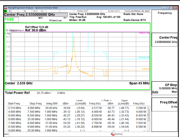
5G NR n7 5MHz BPSK Middle Channel RB1-0, ID:28568
