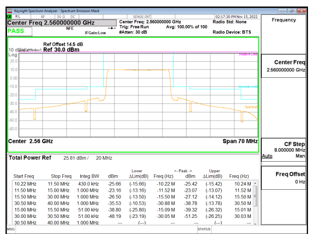
LTE B7 20MHz QPSK High Channel RB100-0, ID:27342
