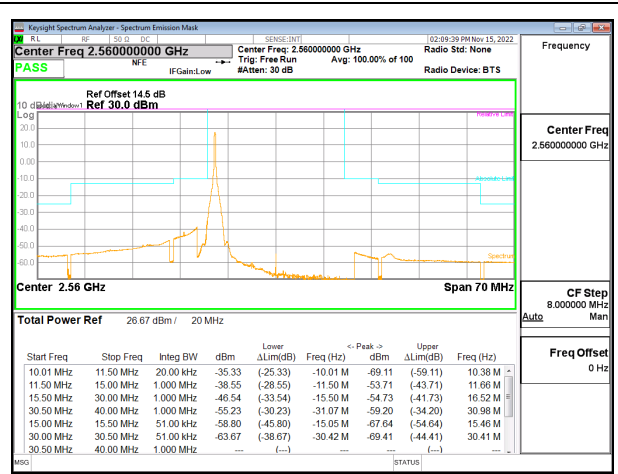
LTE B7 20MHz QPSK High Channel RB1-0, ID:27342
