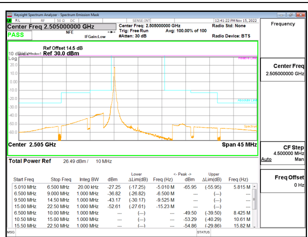
LTE B7 10MHz QPSK Low Channel RB1-0, ID:27342
