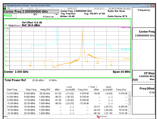
5G NR n7 10MHz BPSK Low Channel RB1-51, ID:28568
