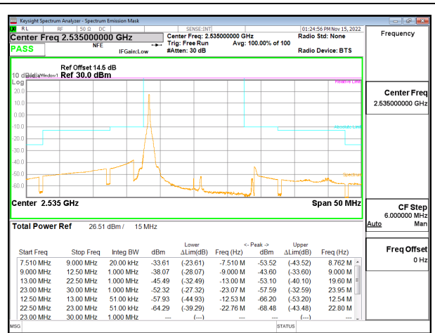
LTE B7 15MHz QPSK Middle Channel RB1-0, ID:27342
