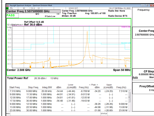
LTE B7 15MHz QPSK Low Channel RB1-74, ID:27342
