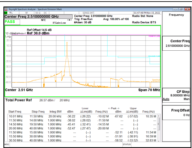
LTE B7 20MHz QPSK Low Channel RB1-0, ID:27342
