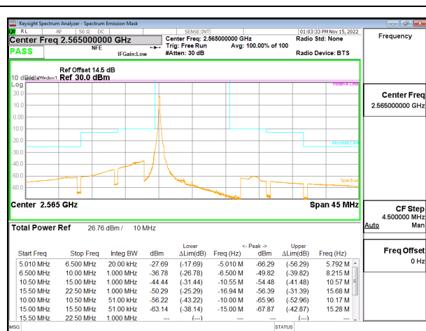
LTE B7 10MHz QPSK High Channel RB1-0, ID:27342
