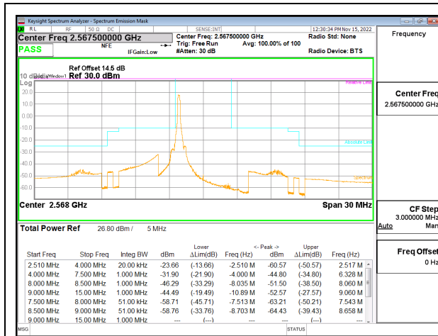
LTE B7 5MHz QPSK High Channel RB1-0, ID:27342
