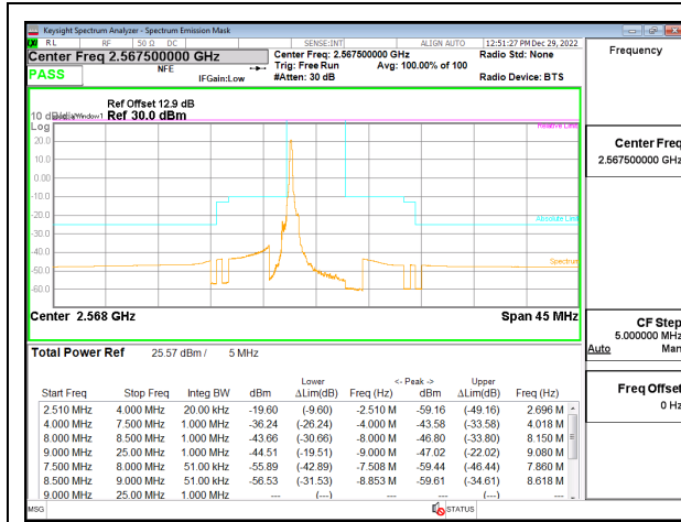
5G NR n7 5MHz BPSK High Channel RB1-0, ID:28568
