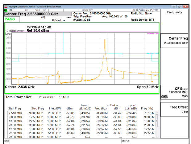
LTE B7 15MHz QPSK Middle Channel RB1-74, ID:27342
