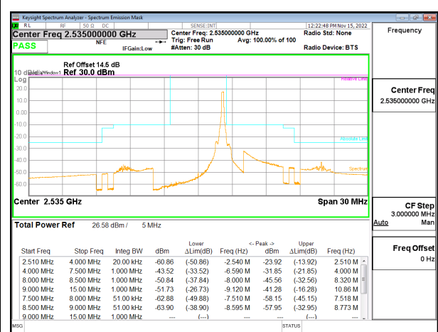
LTE B7 5MHz QPSK Middle Channel RB1-24, ID:27342
