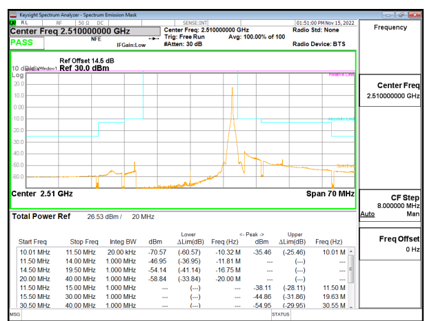
LTE B7 20MHz QPSK Low Channel RB1-99, ID:27342
