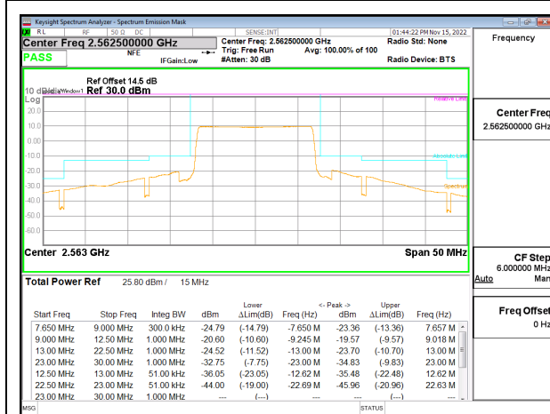
LTE B7 15MHz QPSK High Channel RB75-0, ID:27342
