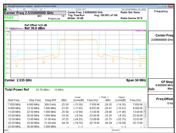
LTE B7 15MHz QPSK Middle Channel RB75-0, ID:27342
