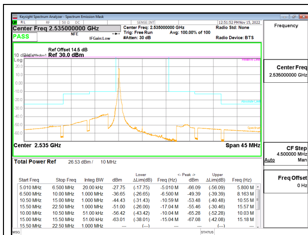
LTE B7 10MHz QPSK Middle Channel RB1-0, ID:27342
