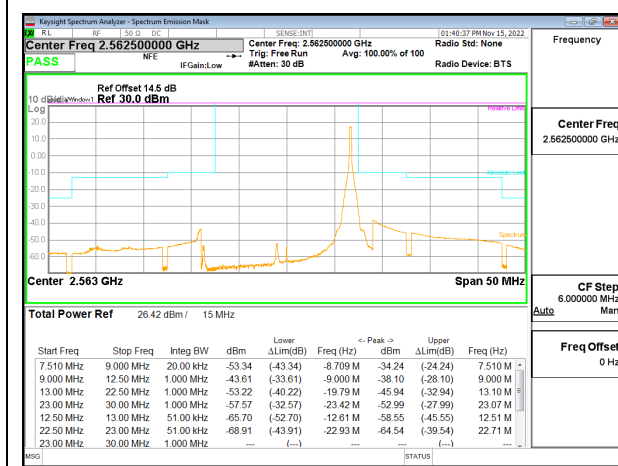
LTE B7 15MHz QPSK High Channel RB1-74, ID:27342
