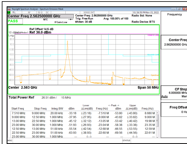
LTE B7 15MHz QPSK High Channel RB1-0, ID:27342
