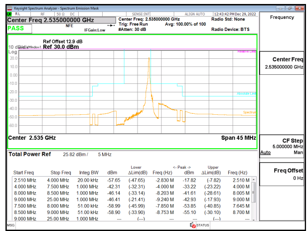
5G NR n7 5MHz BPSK Middle Channel RB1-24, ID:28568
