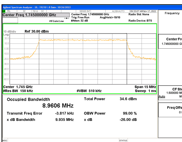
LTE B66 10MHz QPSK Middle Channel RB50-0
