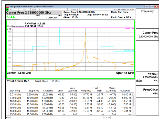
LTE B7 10MHz QPSK Middle Channel RB1-49, ID:27342
