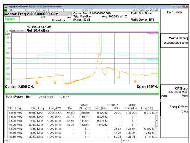
LTE B7 10MHz QPSK Low Channel RB1-49, ID:27342
