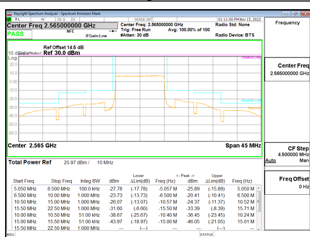
LTE B7 10MHz QPSK High Channel RB50-0, ID:27342
