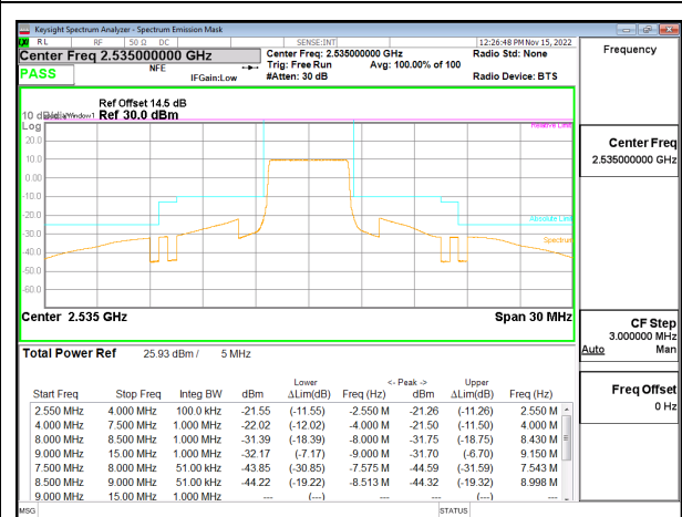
LTE B7 5MHz QPSK Middle Channel RB25-0, ID:27342
