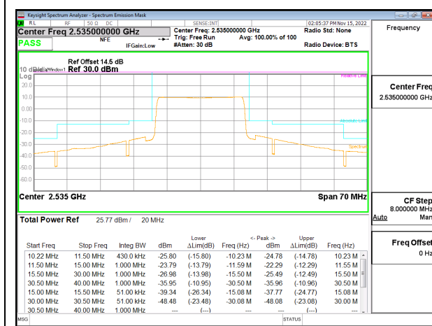
LTE B7 20MHz QPSK Middle Channel RB100-0, ID:27342
