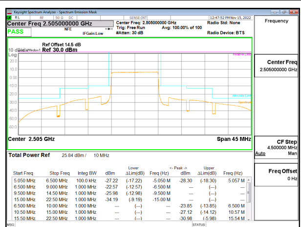
LTE B7 10MHz QPSK Low Channel RB50-0, ID:27342
