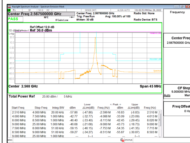
5G NR n7 5MHz BPSK High Channel RB1-24, ID:28568
