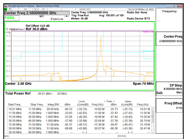
LTE B7 20MHz QPSK High Channel RB1-99, ID:27342
