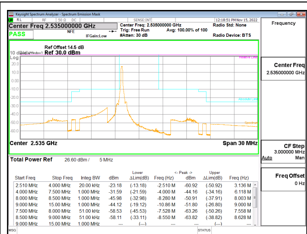
LTE B7 5MHz QPSK Middle Channel RB1-0, ID:27342
