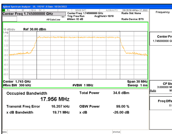
LTE B66 20MHz QPSK Middle Channel RB100-0
