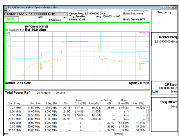
LTE B7 20MHz QPSK Low Channel RB100-0, ID:27342
