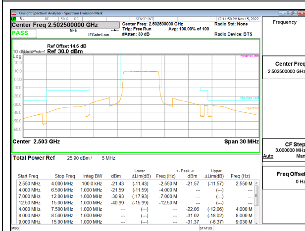
LTE B7 5MHz QPSK Low Channel RB25-0, ID:27342
