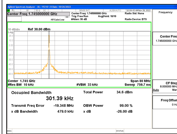
5G NR n66 40MHz BPSK Middle Channel RB1-0
