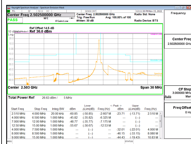
LTE B7 5MHz QPSK Low Channel RB1-24, ID:27342
