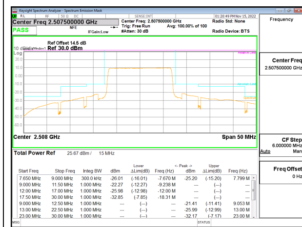
LTE B7 15MHz QPSK Low Channel RB75-0, ID:27342
