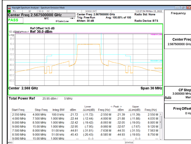
LTE B7 5MHz QPSK High Channel RB25-0, ID:27342
