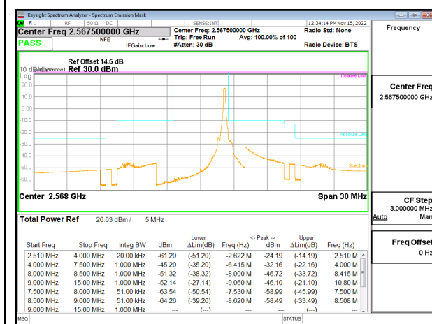
LTE B7 5MHz QPSK High Channel RB1-24, ID:27342
