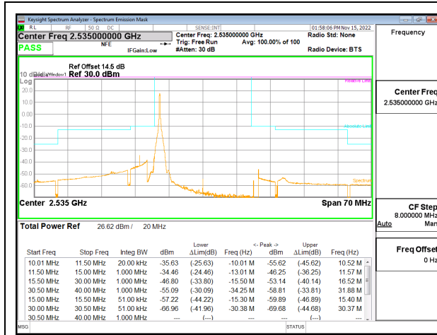
LTE B7 20MHz QPSK Middle Channel RB1-0, ID:27342
