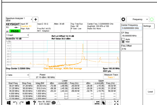
5G NR n77 60MHz BPSK High Channel RB1-161: ID 52275
