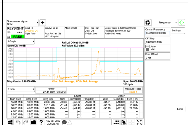
5G NR n77 30MHz BPSK Low Channel RB1-77: ID 52275
