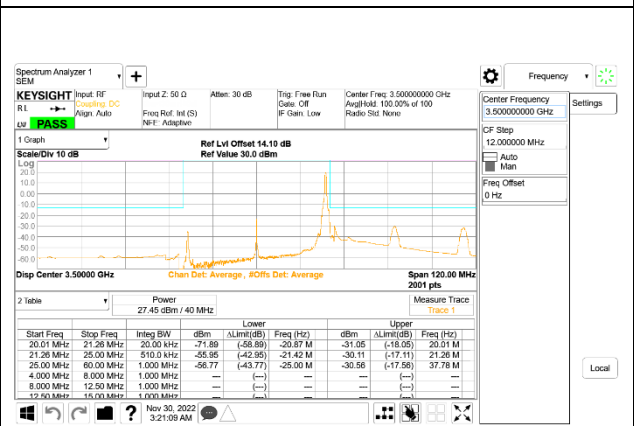
5G NR n77 40MHz BPSK Middle Channel RB1-105: ID 52275
