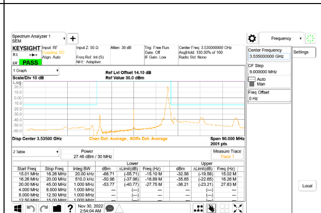
5G NR n77 30MHz BPSK High Channel RB1-77: ID 52275
