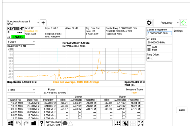
5G NR n77 30MHz BPSK Middle Channel RB1-77: ID 52275
