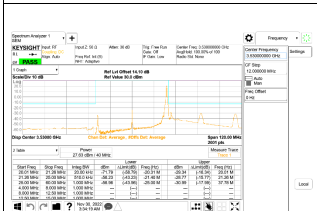
5G NR n77 40MHz BPSK High Channel RB1-105: ID 52275
