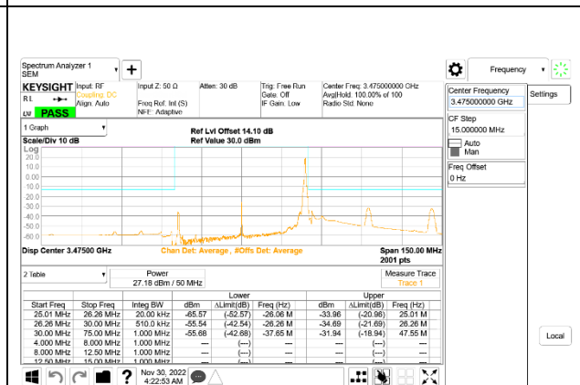
5G NR n77 50MHz BPSK Low Channel RB1-132: ID 52275
