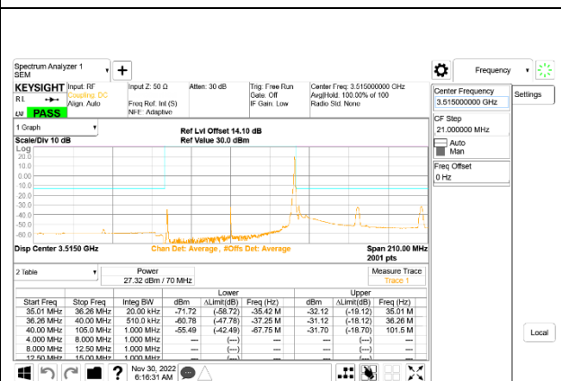
5G NR n77 70MHz BPSK High Channel RB1-188: ID 52275
