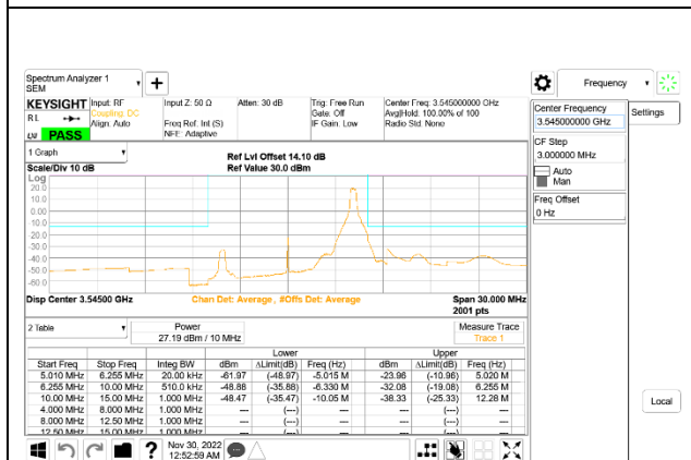
5G NR n77 10MHz BPSK High Channel RB1-23: ID 52275
