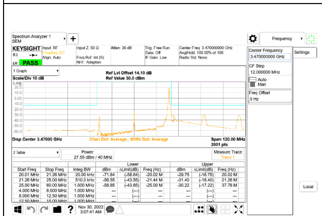
5G NR n77 40MHz BPSK Low Channel RB1-105: ID 52275
