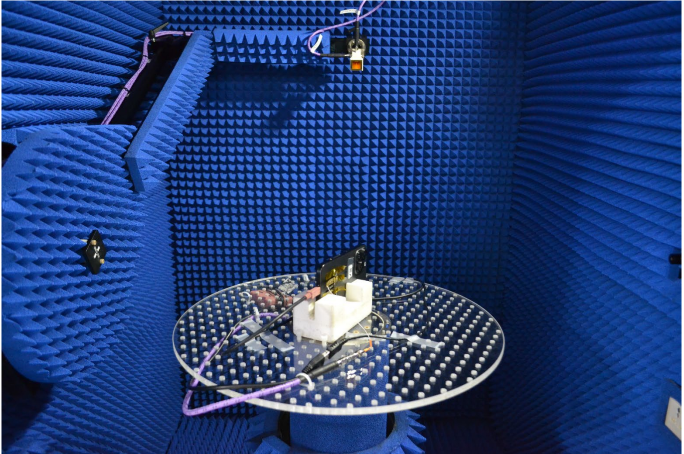
Figure C-6 Conducted Radiated power mmW test measurement setup
