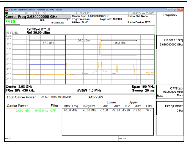
5G NR n48 40MHz BPSK High Channel RB1-05
