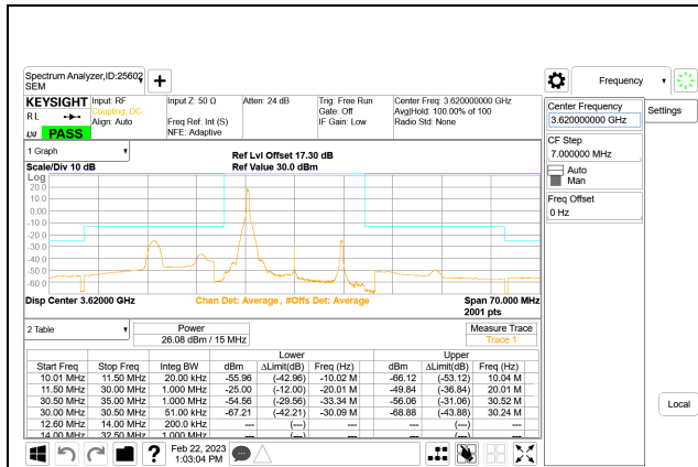
5G NR n48 15MHz BPSK Middle Channel RB1-0
