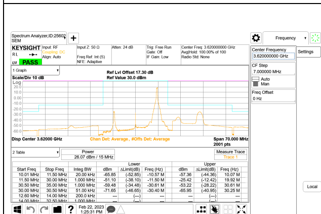
5G NR n48 15MHz BPSK Middle Channel RB1-37
