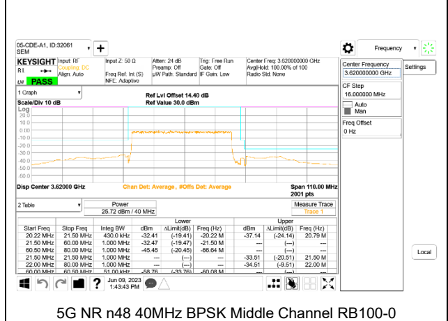
5G NR n48 40MHz BPSK Middle Channel RB100-0
