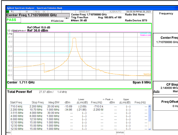
LTE B66 1.4MHz QPSK Low Channel RB1-0, ID:25780
