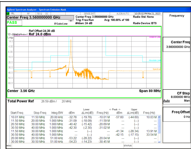
LTE B48 20MHz QPSK Low Channel RB1-0, ID:25780
