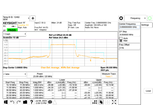
LTE B48 20MHz QPSK High Channel RB100-0, ID:25780
