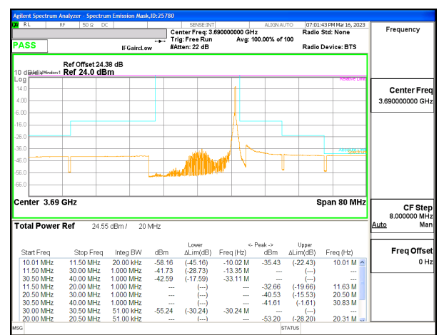
LTE B48 20MHz QPSK High Channel RB1-99, ID:25780
