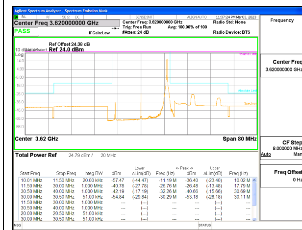
LTE B48 20MHz QPSK Middle Channel RB1-99, ID:25780
