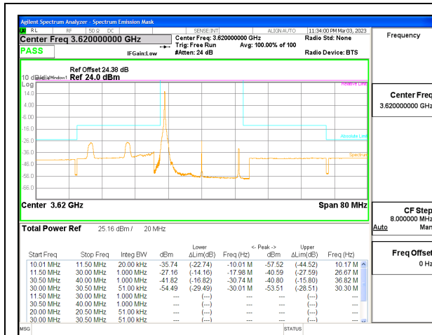
LTE B48 20MHz QPSK Middle Channel RB1-0, ID:25780
