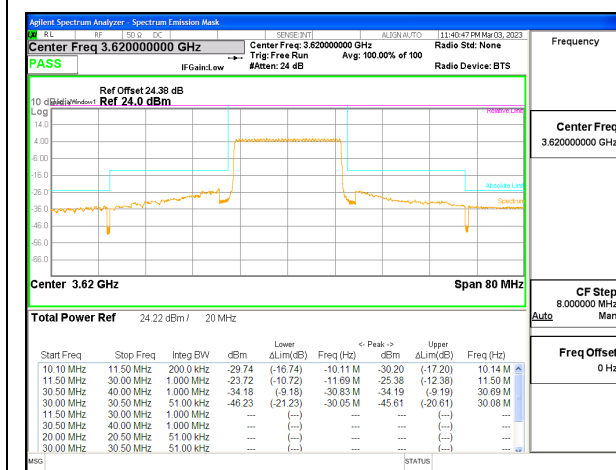
LTE B48 20MHz QPSK Middle Channel RB100-0, ID:25780
