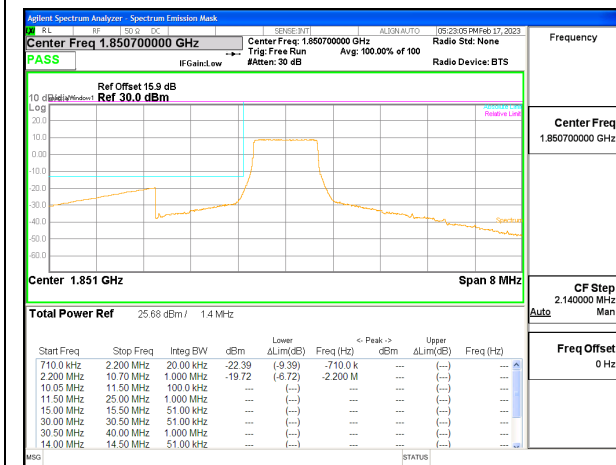
LTE B25 1.4MHz QPSK Low Channel RB6-0 ID:25780
