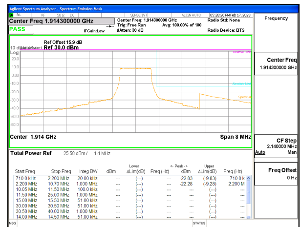
LTE B25 1.4MHz QPSK High Channel RB6-0 ID:25780
