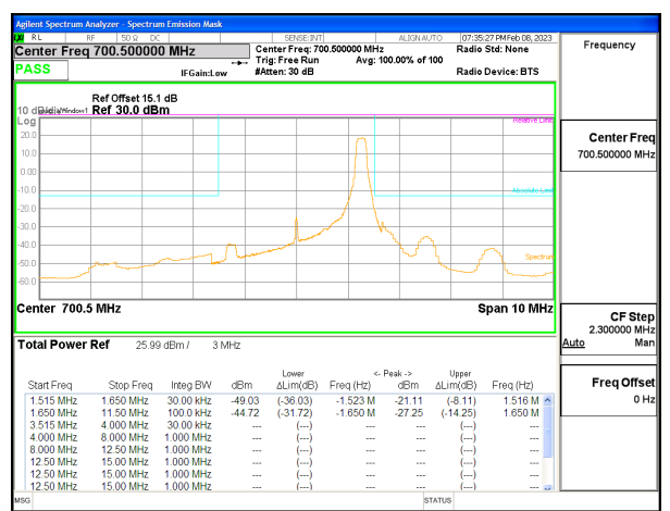
LTE B12 3MHz QPSK Low Channel RB1-14, ID:25780
