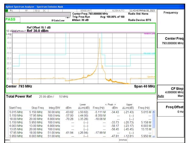
LTE B14 10MHz QPSK Middle Channel RB1-49, ID:25780
