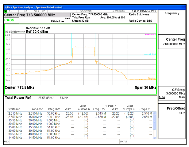
LTE B17 5MHz QPSK High Channel RB25-0 ID:25780
