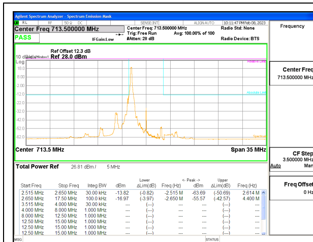
5G NR n12 5MHz BPSK High Channel RB1-0, ID:12482
