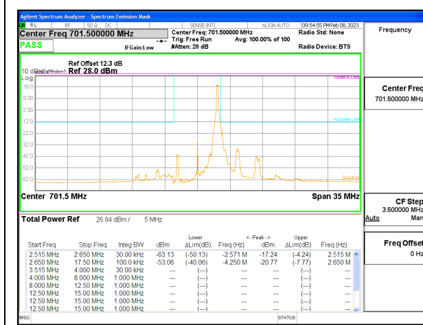
5G NR n12 5MHz BPSK Low Channel RB1-24, ID:12482
