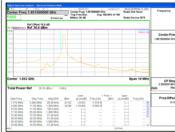
LTE B25 3MHz QPSK Low Channel RB1-0, ID:25780
