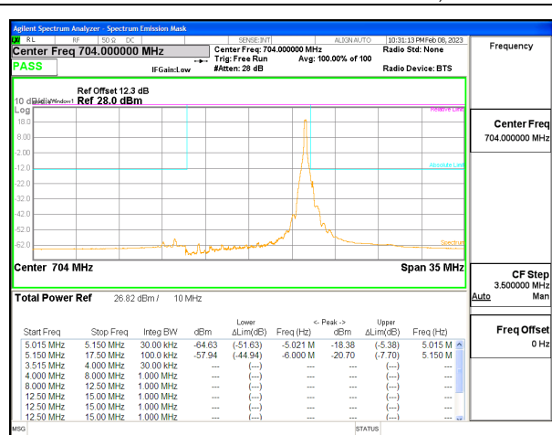
5G NR n12 10MHz BPSK Low Channel RB1-51, ID:12482
