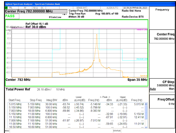
LTE B13 10MHz QPSK Middle Channel RB1-49 ID:25780
