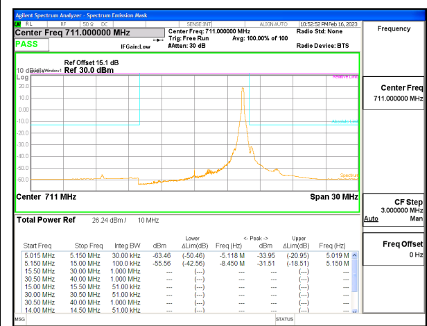
LTE B17 10MHz QPSK High Channel RB1-49 ID:25780
