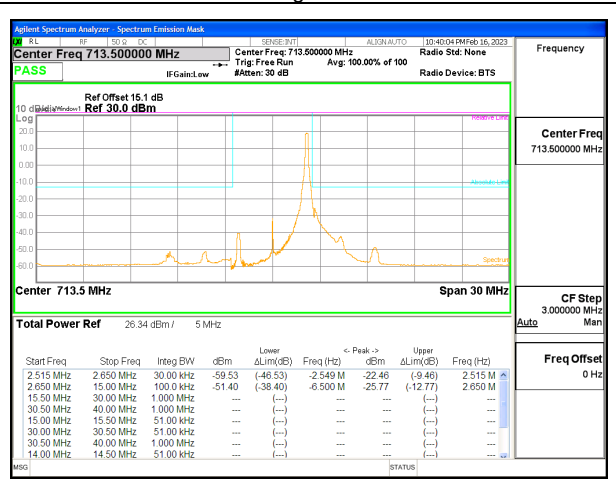
LTE B17 5MHz QPSK High Channel RB1-24 ID:25780
