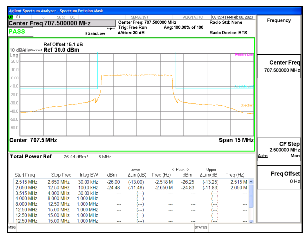
LTE B12 5MHz QPSK Middle Channel RB25-0, ID:25780
