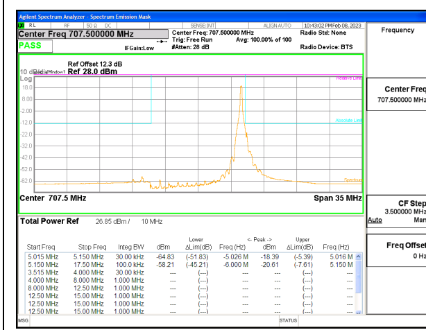
5G NR n12 10MHz BPSK Middle Channel RB1-51, ID:12482
