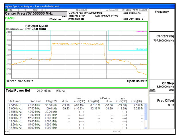
5G NR n12 15MHz BPSK Middle Channel RB75-0, ID:12482
