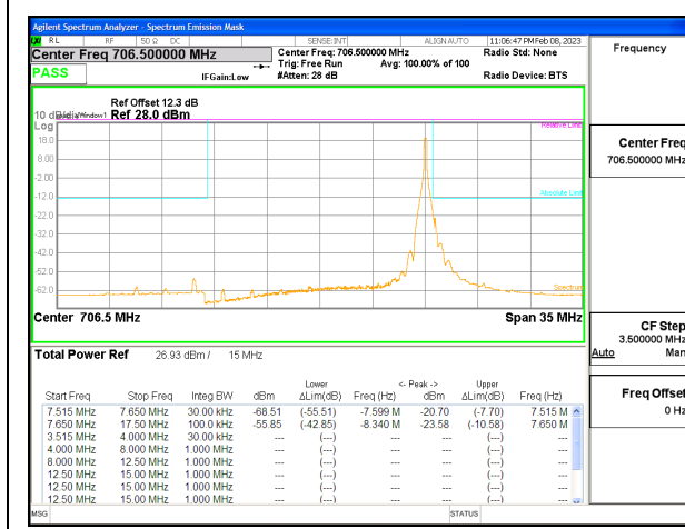
5G NR n12 15MHz BPSK Low Channel RB1-78, ID:12482
