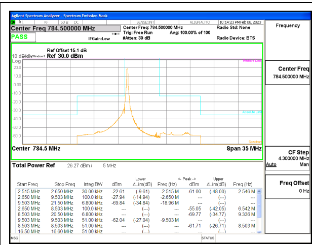
LTE B13 5MHz QPSK High Channel RB1-0, ID:25780
