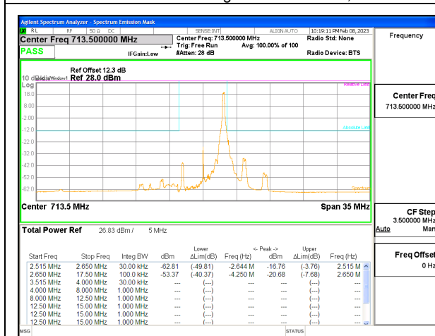
5G NR n12 5MHz BPSK High Channel RB1-24, ID:12482
