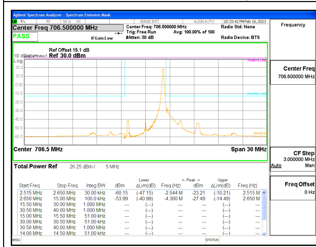
LTE B17 5MHz QPSK Low Channel RB1-24 ID:25780
