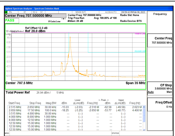
5G NR n12 5MHz BPSK Middle Channel RB1-0, ID:12482
