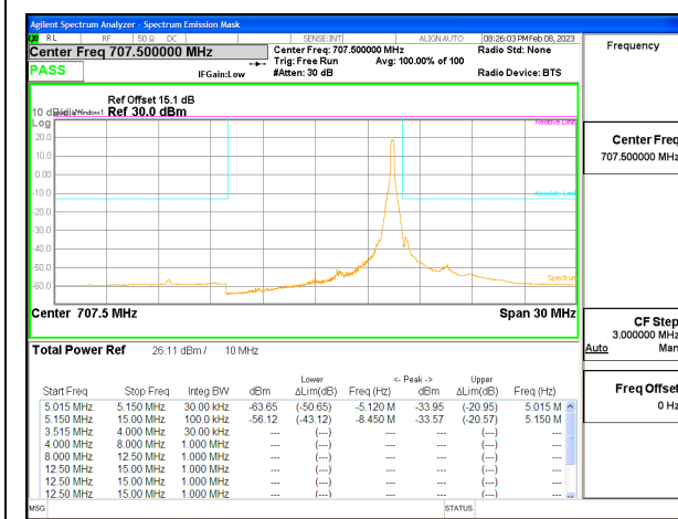
LTE B12 10MHz QPSK Middle Channel RB1-49, ID:25780
