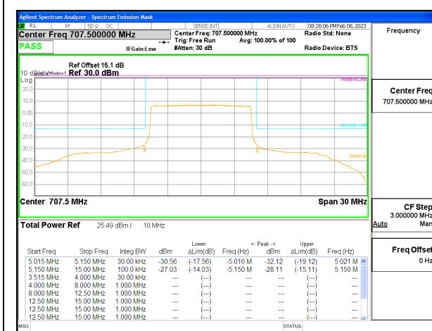
LTE B12 10MHz QPSK Middle Channel RB50-0, ID:25780
