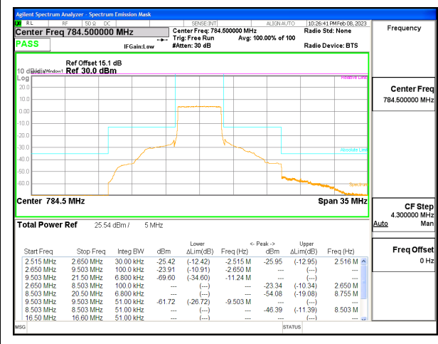
LTE B13 5MHz QPSK High Channel RB25-0, ID:25780
