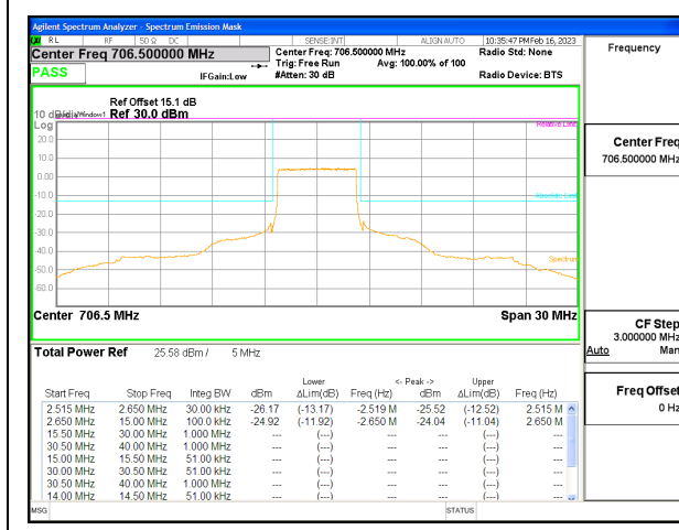
LTE B17 5MHz QPSK Low Channel RB25-0 ID:25780
