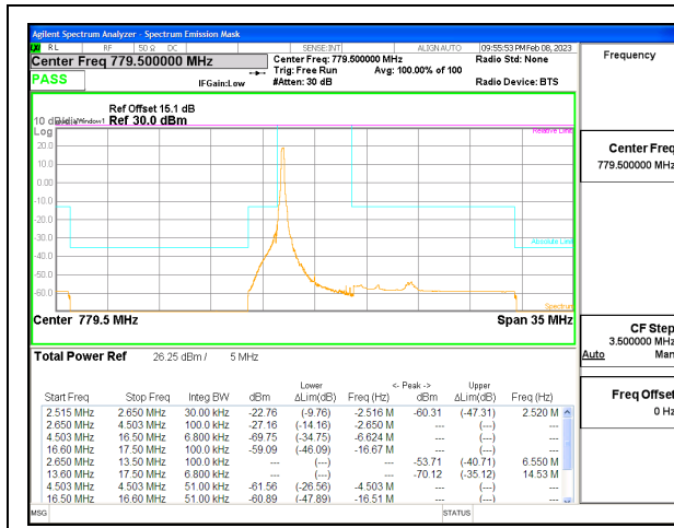
LTE B13 5MHz QPSK Low Channel RB1-0, ID:25780
