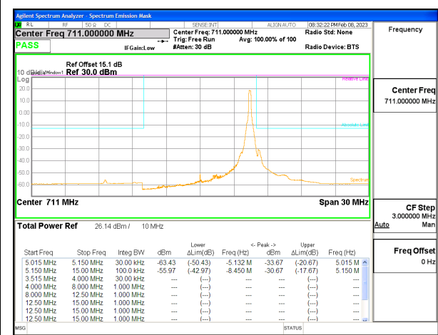
LTE B12 10MHz QPSK High Channel RB1-49, ID:25780
