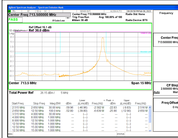
LTE B12 5MHz QPSK High Channel RB1-24, ID:25780
