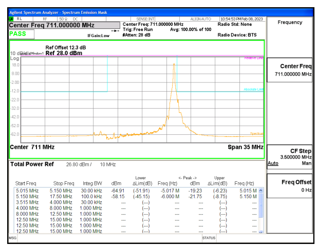
5G NR n12 10MHz BPSK High Channel RB1-51, ID:12482
