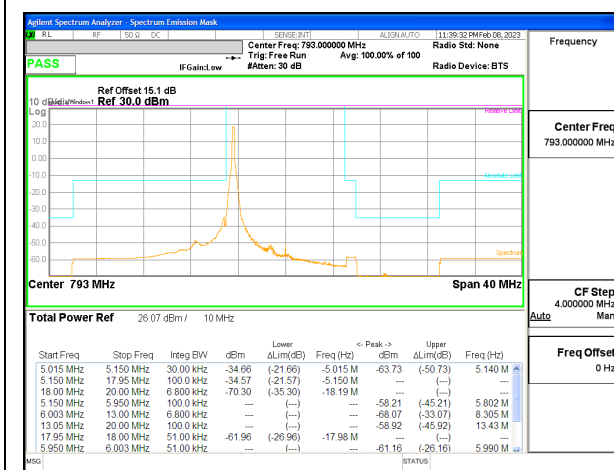
LTE B14 10MHz QPSK Middle Channel RB1-0, ID:25780
