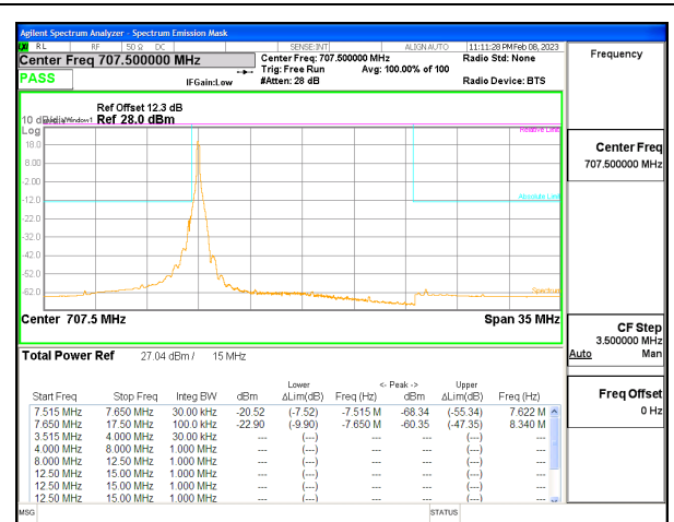
5G NR n12 15MHz BPSK Middle Channel RB1-0, ID:12482
