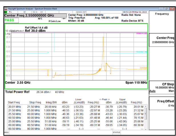
5G NR n7 40MHz BPSK High Channel RB1-215, ID:32061
