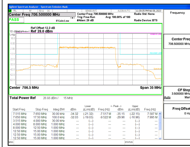
5G NR n12 15MHz BPSK Low Channel RB75-0, ID:12482
