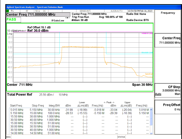
LTE B17 10MHz QPSK High Channel RB50-0 ID:25780
