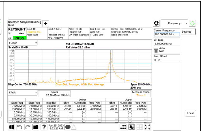
5G NR n12 15MHz BPSK High Channel RB1-78
