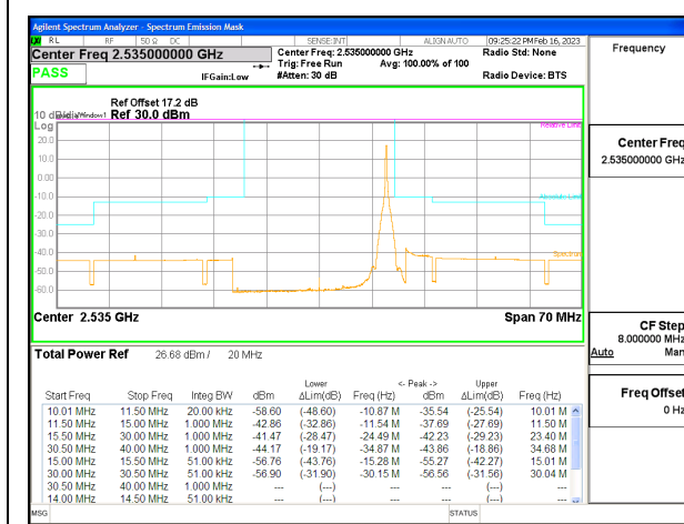
LTE B7 20MHz QPSK Middle Channel RB1-99, ID:25780
