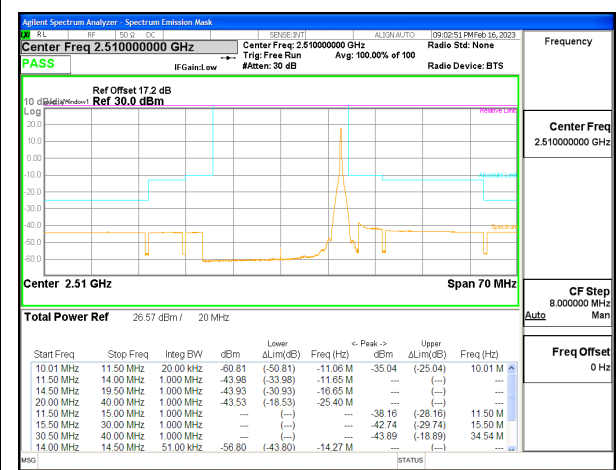
LTE B7 20MHz QPSK Low Channel RB1-99, ID:25780
