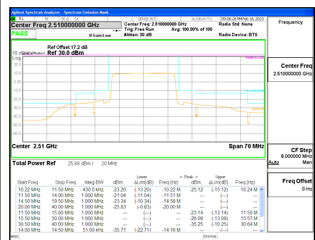
LTE B7 20MHz QPSK Low Channel RB100-0, ID:25780
