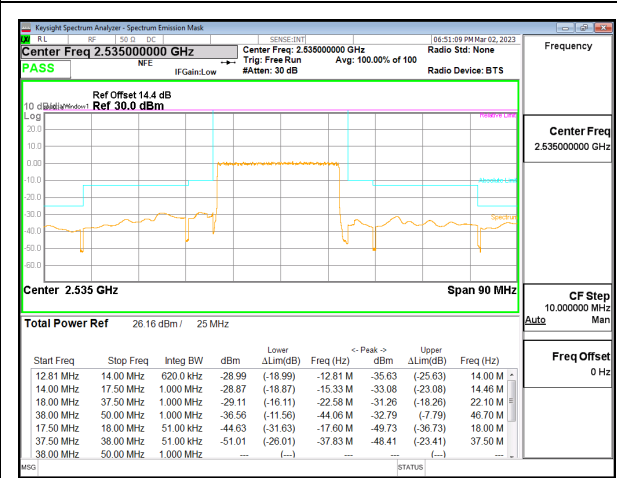
5G NR n7 25MHz BPSK Middle Channel RB128-0, ID:32061
