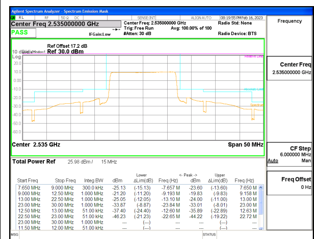
LTE B7 15MHz QPSK Middle Channel RB75-0, ID:25780
