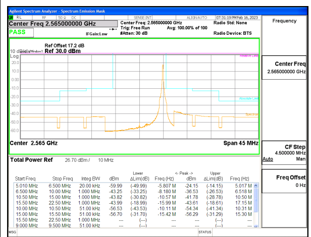
LTE B7 10MHz QPSK High Channel RB1-49, ID:25780
