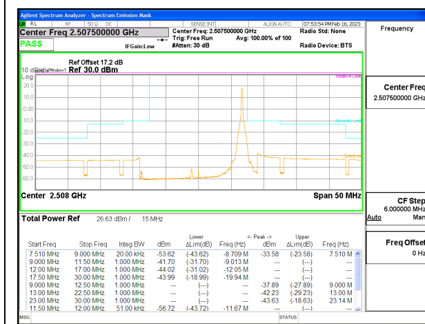
LTE B7 15MHz QPSK Low Channel RB1-74, ID:25780
