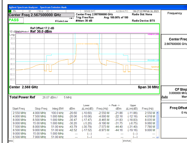
LTE B7 5MHz QPSK High Channel RB25-0, ID:25780
