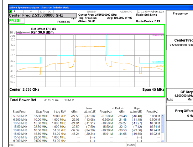
LTE B7 10MHz QPSK Middle Channel RB50-0, ID:25780
