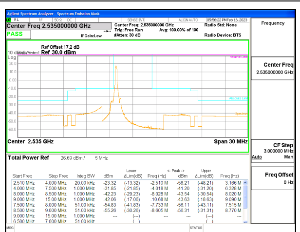
LTE B7 5MHz QPSK Middle Channel RB1-0, ID:25780
