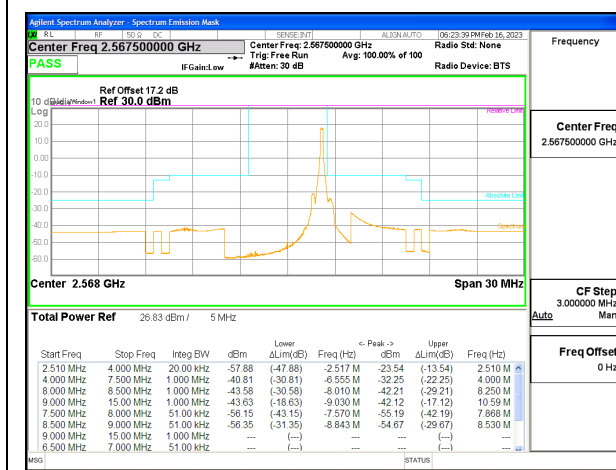
LTE B7 5MHz QPSK High Channel RB1-24, ID:25780
