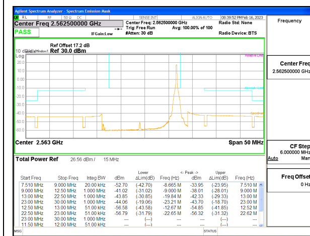
LTE B7 15MHz QPSK High Channel RB1-74, ID:25780
