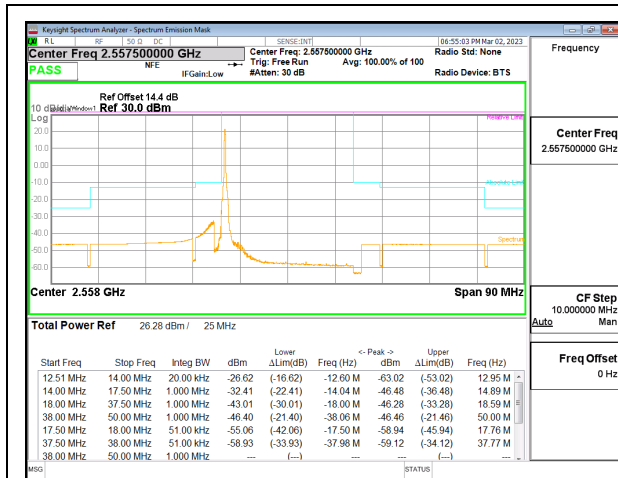
5G NR n7 25MHz BPSK High Channel RB1-0, ID:32061
