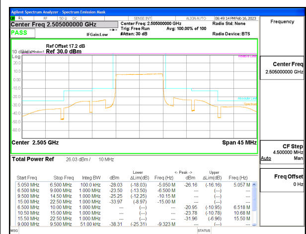
LTE B7 10MHz QPSK Low Channel RB50-0, ID:25780
