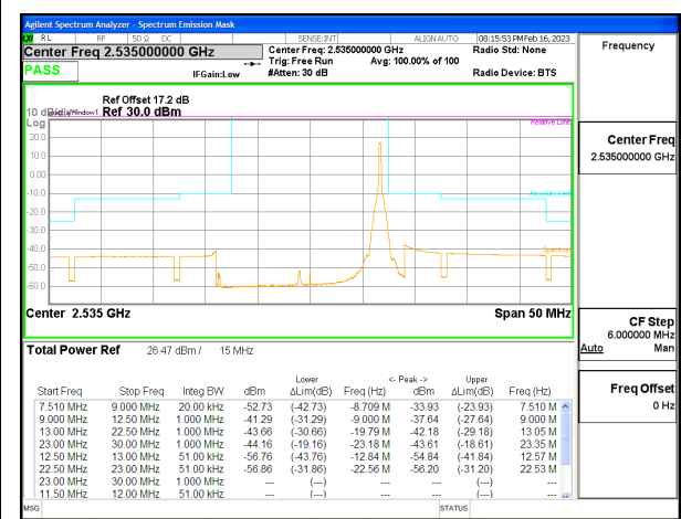
LTE B7 15MHz QPSK Middle Channel RB1-74, ID:25780
