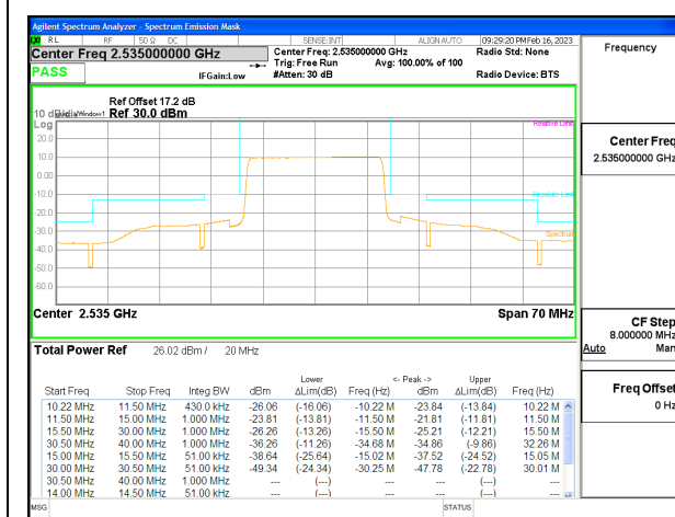
LTE B7 20MHz QPSK Middle Channel RB100-0, ID:25780
