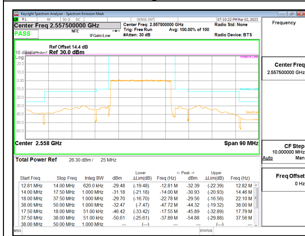
5G NR n7 25MHz BPSK High Channel RB128-0, ID:32061
