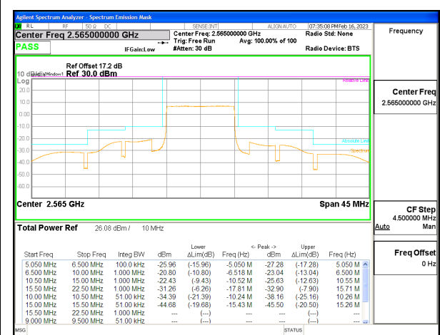
LTE B7 10MHz QPSK High Channel RB50-0, ID:25780
