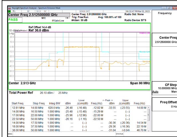
5G NR n7 25MHz BPSK Low Channel RB128-0, ID:32061
