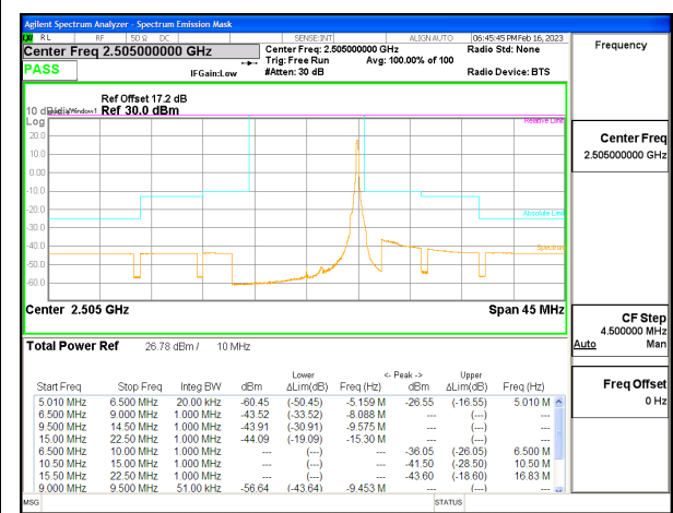
LTE B7 10MHz QPSK Low Channel RB1-49, ID:25780
