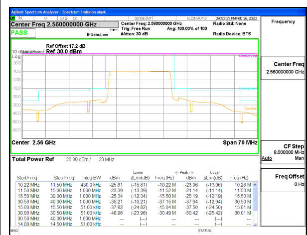
LTE B7 20MHz QPSK High Channel RB100-0, ID:25780
