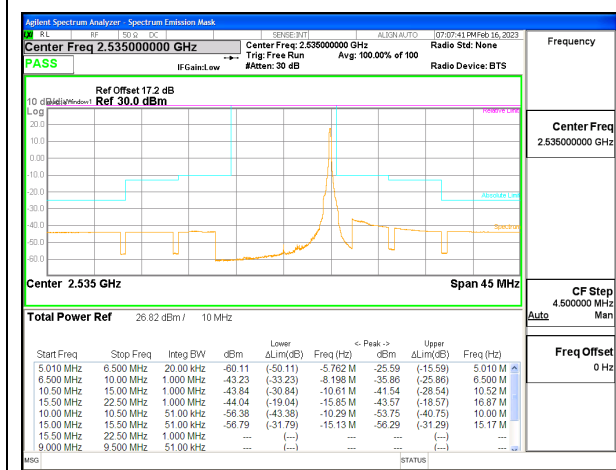
LTE B7 10MHz QPSK Middle Channel RB1-49, ID:25780
