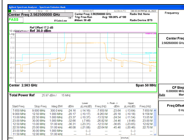
LTE B7 15MHz QPSK High Channel RB75-0, ID:25780
