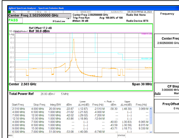
LTE B7 5MHz QPSK Low Channel RB1-0, ID:25780
