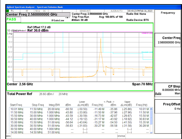
LTE B7 20MHz QPSK High Channel RB1-99, ID:25780
