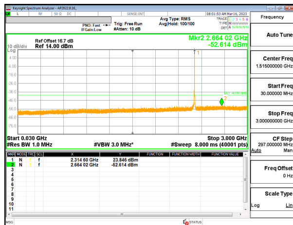
5G NR n30 5MHz QPSK High Channel RB1-0 (30MHz to 3GHz) ID:32061
