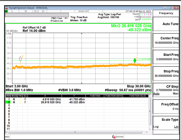
5G NR n30 5MHz QPSK Low Channel RB1-0 (3G to 26G), ID:32061
