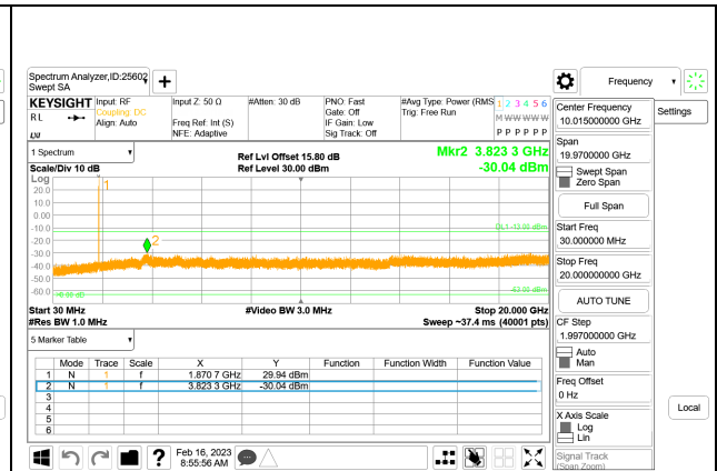
5G NR n25 25MHz BPSK Middle Channel RB1-1
