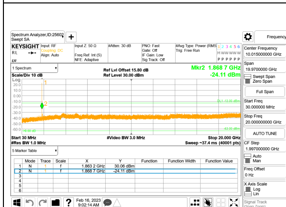
5G NR n25 40MHz BPSK Middle Channel RB1-1
