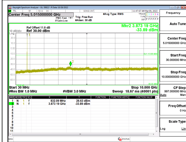
5G NR n26 10MHz BPSK Middle Channel RB1-1
