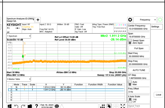
5G NR n25 20MHz BPSK High Channel RB1-105
