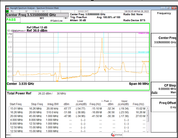
5G NR n77 30MHz BPSK High Channel RB1-77, ID:19146
