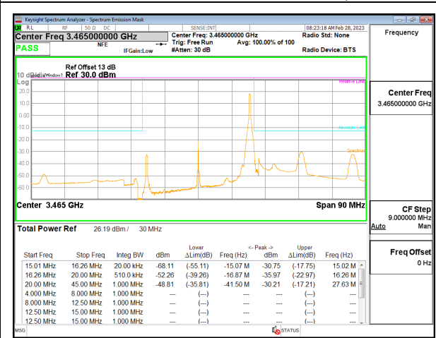
5G NR n77 30MHz BPSK Low Channel RB1-77, ID:19146
