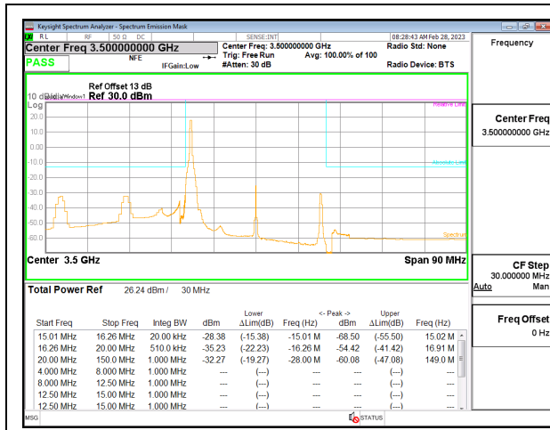
5G NR n77 30MHz BPSK Middle Channel RB1-0, ID:19146
