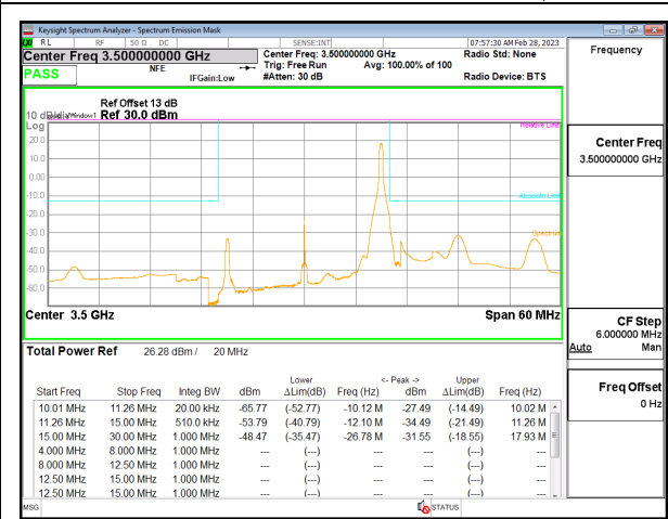
5G NR n77 20MHz BPSK Middle Channel RB1-50, ID:19146
