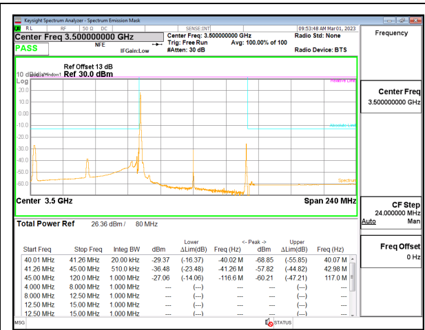
5G NR n77 80MHz BPSK Middle Channel RB1-0, ID:19146
