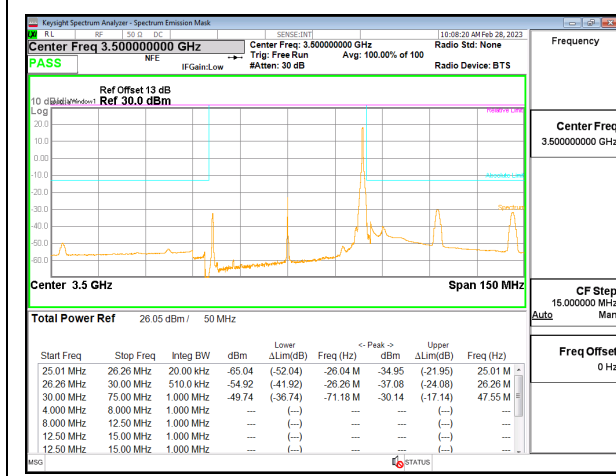
5G NR n77 50MHz BPSK Middle Channel RB1-132, ID:19146
