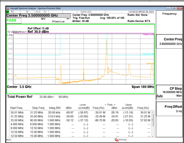
5G NR n77 60MHz BPSK Middle Channel RB1-161, ID:19146
