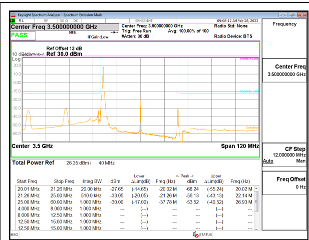
5G NR n77 40MHz BPSK Middle Channel RB1-0, ID:19146
