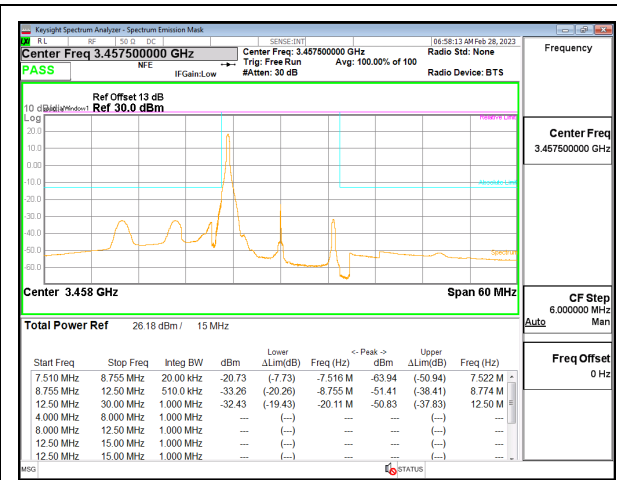
5G NR n77 15MHz BPSK Low Channel RB1-0, ID:19146
