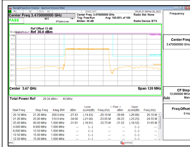
5G NR n77 40MHz BPSK Low Channel RB100-0, ID:19146
