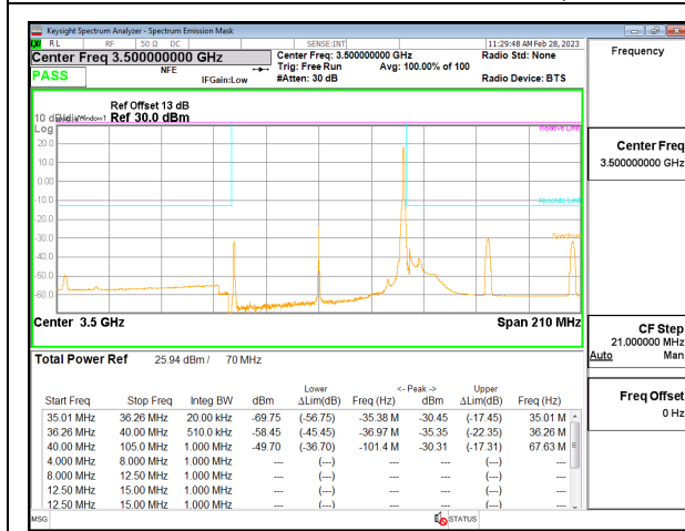
5G NR n77 70MHz BPSK Middle Channel RB1-188, ID:19146
