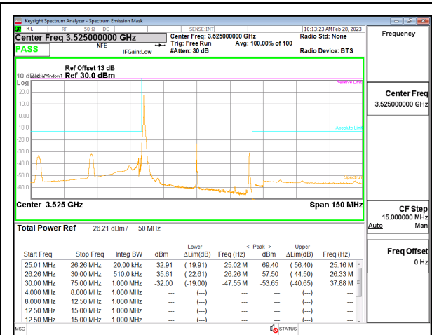
5G NR n77 50MHz BPSK High Channel RB1-0, ID:19146
