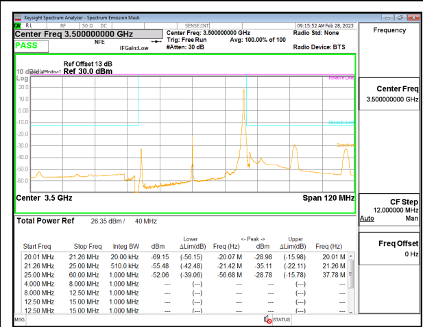
5G NR n77 40MHz BPSK Middle Channel RB1-105, ID:19146
