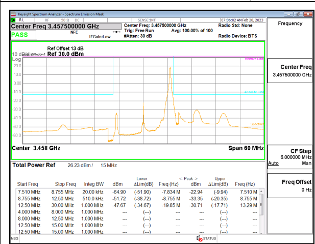
5G NR n77 15MHz BPSK Low Channel RB1-37, ID:19146
