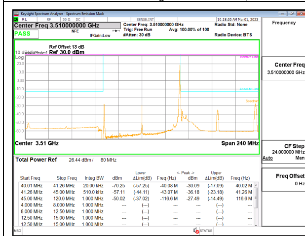
5G NR n77 80MHz BPSK High Channel RB1-216, ID:19146
