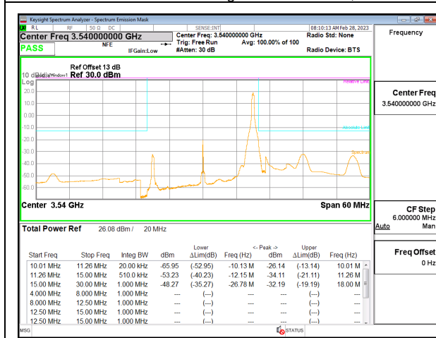
5G NR n77 20MHz BPSK High Channel RB1-50, ID:19146
