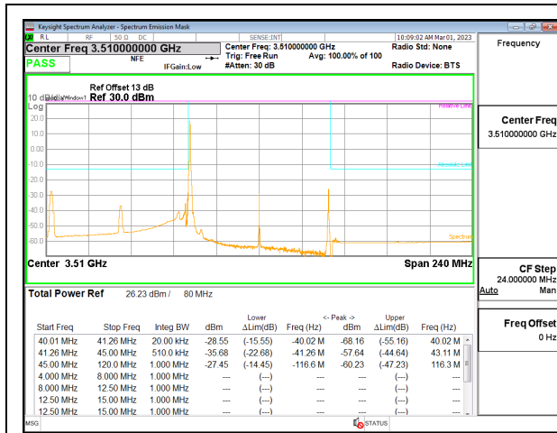
5G NR n77 80MHz BPSK High Channel RB1-0, ID:19146
