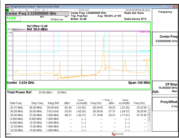
5G NR n77 50MHz BPSK High Channel RB1-132, ID:19146
