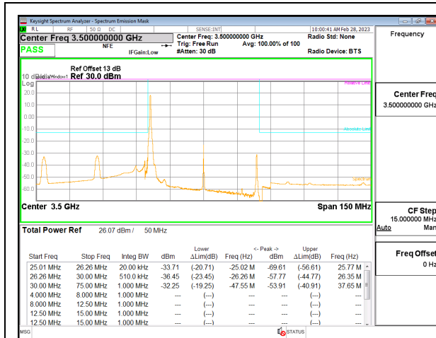
5G NR n77 50MHz BPSK Middle Channel RB1-0, ID:19146
