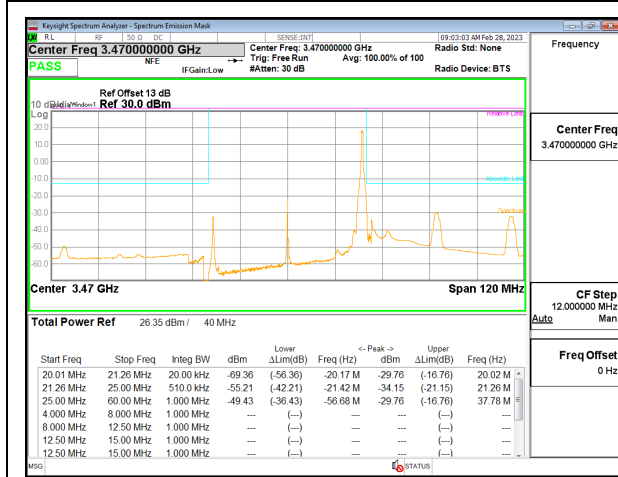
5G NR n77 40MHz BPSK Low Channel RB1-105, ID:19146
