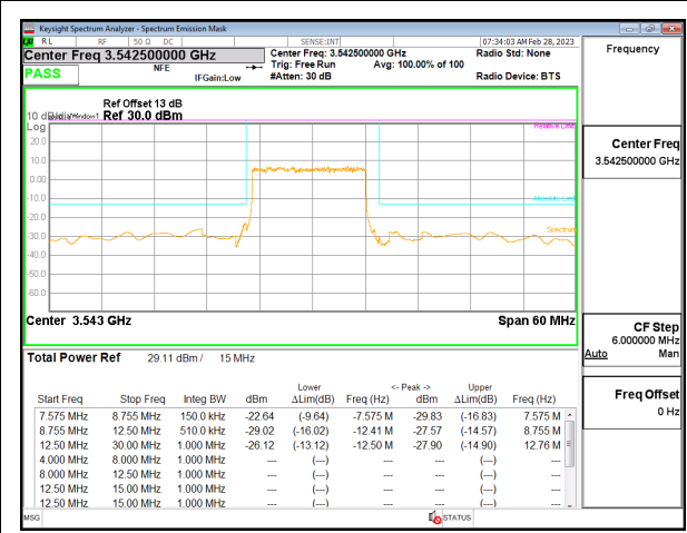
5G NR n77 15MHz BPSK High Channel RB36-0, ID:19146
