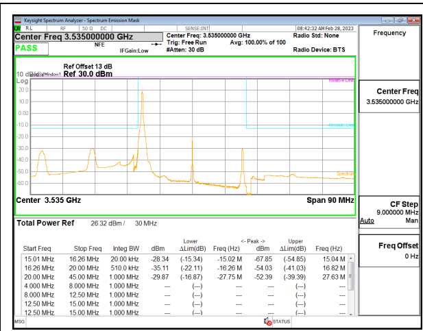
5G NR n77 30MHz BPSK High Channel RB1-0, ID:19146
