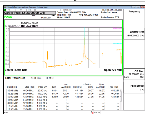
5G NR n77 90MHz BPSK High Channel RB1-244, ID:19146
