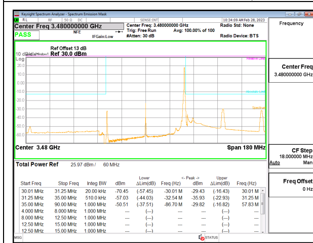
5G NR n77 60MHz BPSK Low Channel RB1-161, ID:19146
