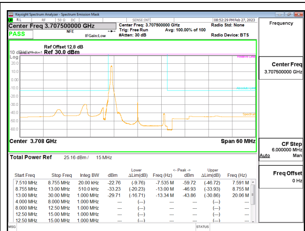
5G NR n77 15MHz BPSK Low Channel RB1-0, ID:50822
