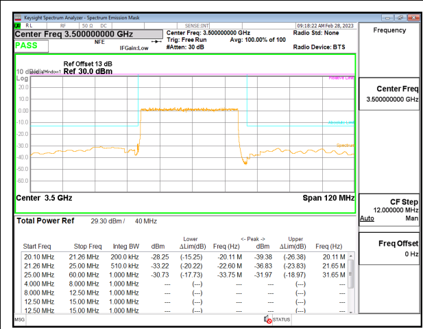
5G NR n77 40MHz BPSK Middle Channel RB100-0, ID:19146
