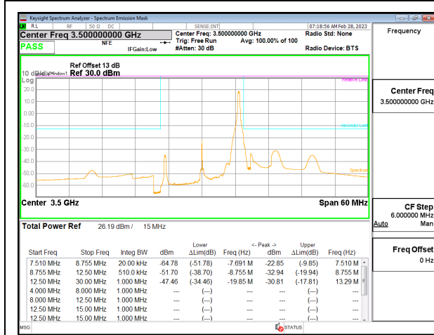
5G NR n77 15MHz BPSK Middle Channel RB1-37, ID:19146
