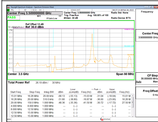
5G NR n77 30MHz BPSK Middle Channel RB1-77, ID:19146
