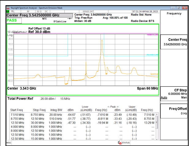
5G NR n77 15MHz BPSK High Channel RB1-37, ID:19146
