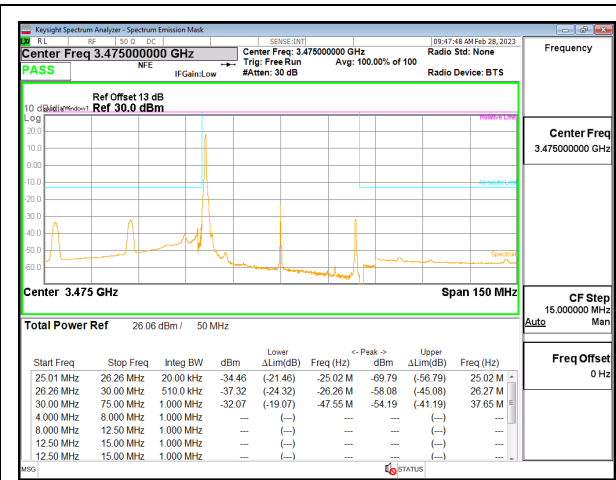
5G NR n77 50MHz BPSK Low Channel RB1-0, ID:19146
