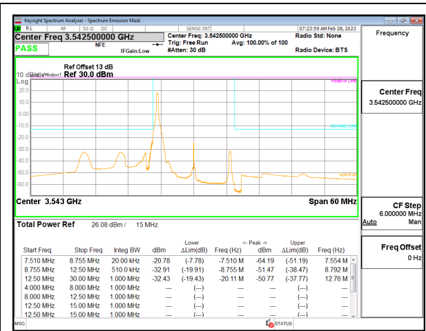
5G NR n77 15MHz BPSK High Channel RB1-0, ID:19146
