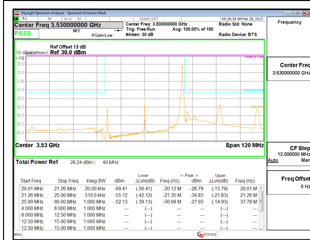
5G NR n77 40MHz BPSK High Channel RB1-105, ID:19146
