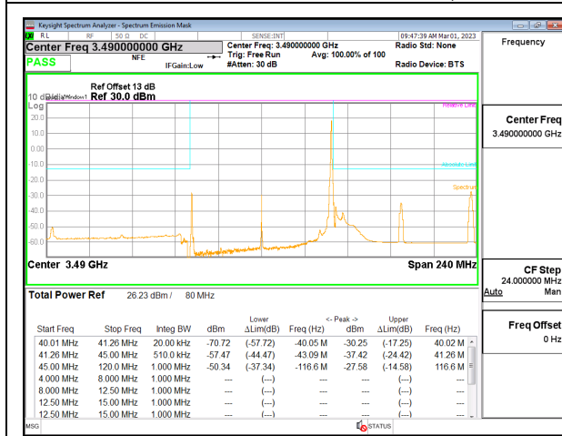
5G NR n77 80MHz BPSK Low Channel RB1-216, ID:19146
