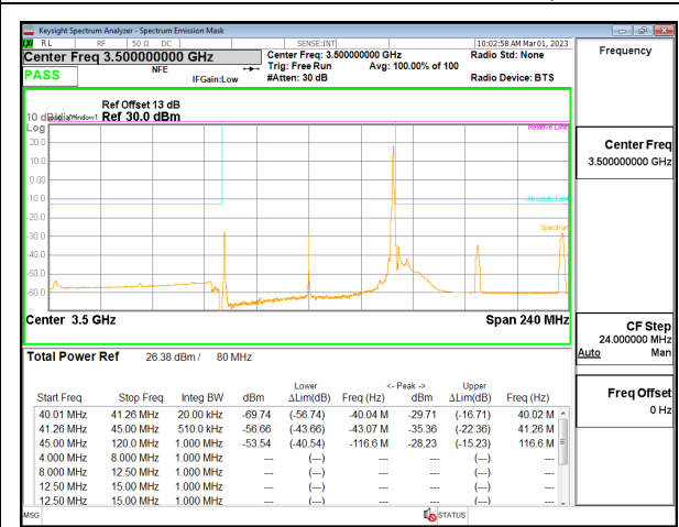
5G NR n77 80MHz BPSK Middle Channel RB1-216, ID:19146
