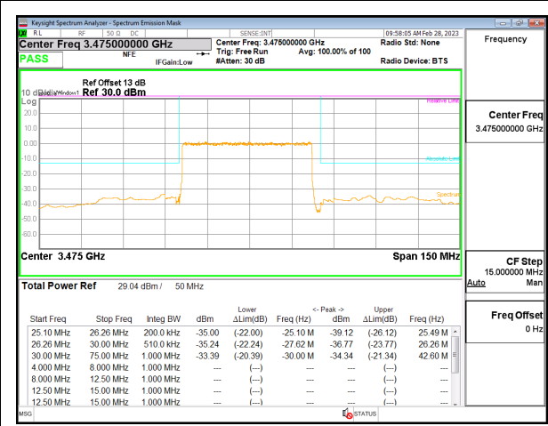
5G NR n77 50MHz BPSK Low Channel RB128-0, ID:19146
