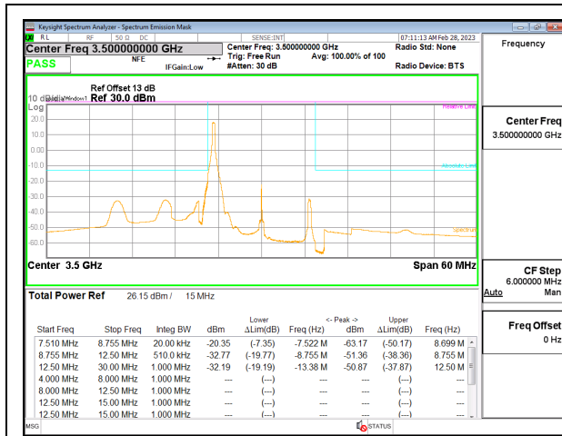
5G NR n77 15MHz BPSK Middle Channel RB1-0, ID:19146
