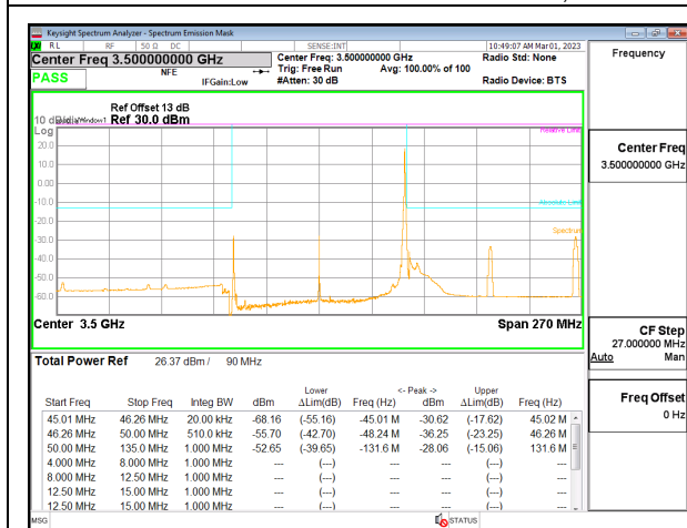
5G NR n77 90MHz BPSK Middle Channel RB1-244, ID:19146
