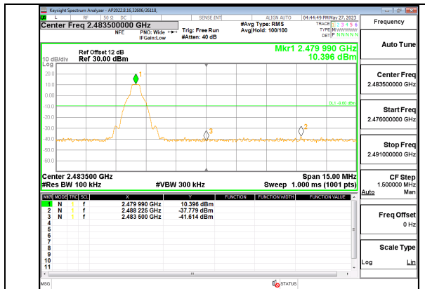
HIGH CHANNEL BANDEDGE ANT 4
