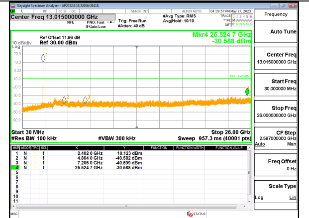
LOW CHANNEL OUT-OF-BAND ANT 4
