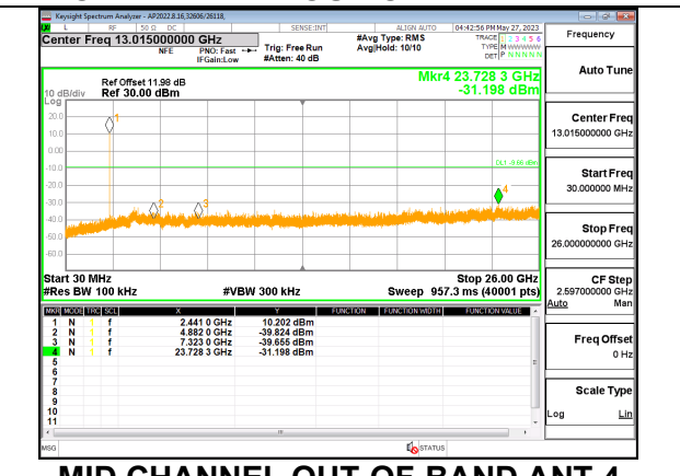
MID CHANNEL OUT-OF-BAND ANT 4
