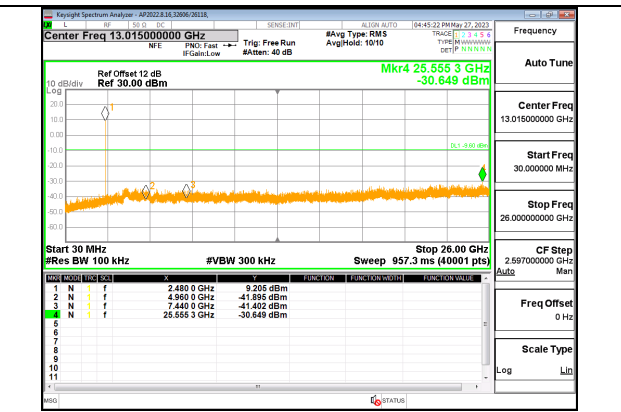
HIGH CHANNEL OUT-OF-BAND ANT 4
