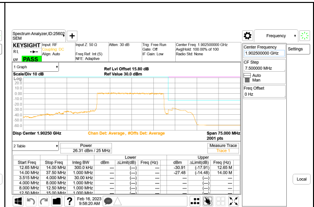
5G NR n25 25MHz BPSK High Channel RB128-0
