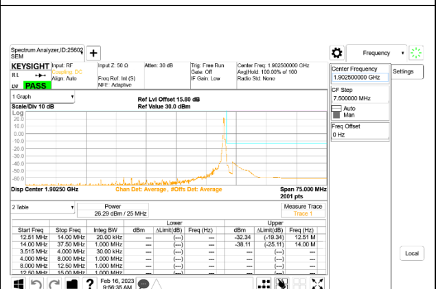
5G NR n25 25MHz BPSK High Channel RB1-132
