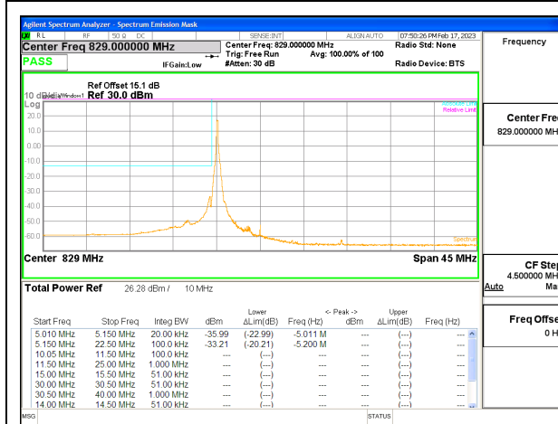
LTE B26 10MHz QPSK Low Channel RB1-0, ID:25780
