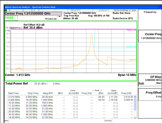
LTE B25 5MHz QPSK High Channel RB1-24, ID:25780
