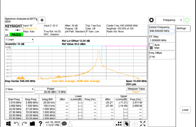
LTE B26 5MHz QPSK High Channel RB1-24
