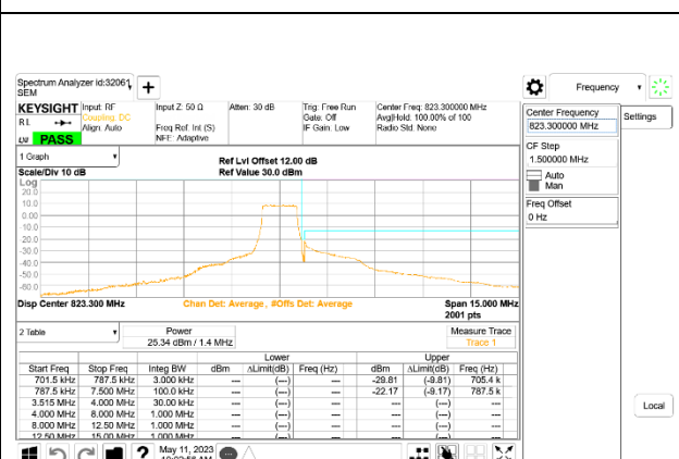
LTE B26 1.4MHz QPSK High Channel RB6-0
