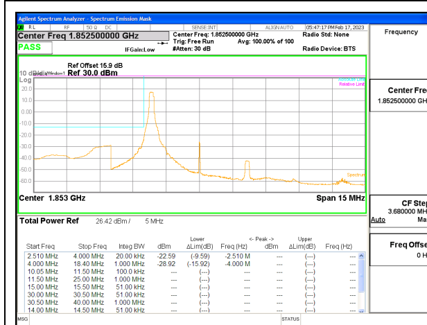
LTE B25 5MHz QPSK Low Channel RB1-0, ID:25780
