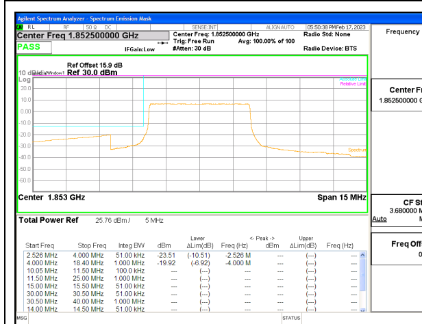
LTE B25 5MHz QPSK Low Channel RB25-0 ID:25780
