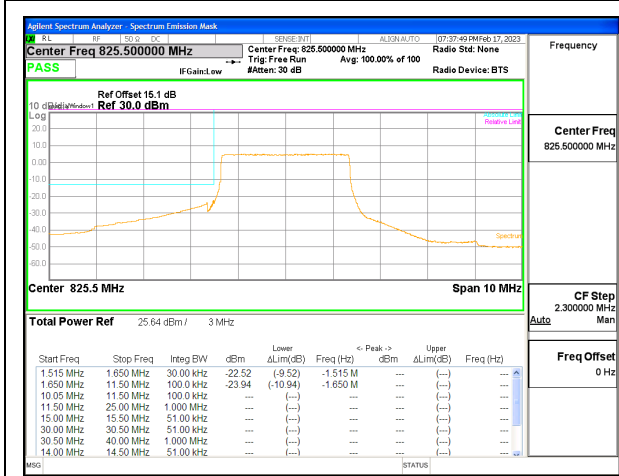
LTE B26 3MHz QPSK Low Channel RB15-0, ID:25780
