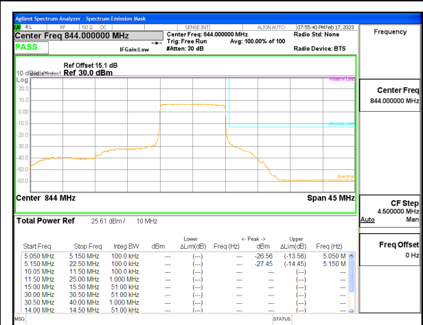
LTE B26 10MHz QPSK High Channel RB50-0, ID:25780
