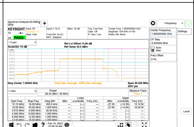
5G NR n25 30MHz BPSK High Channel RB160-0
