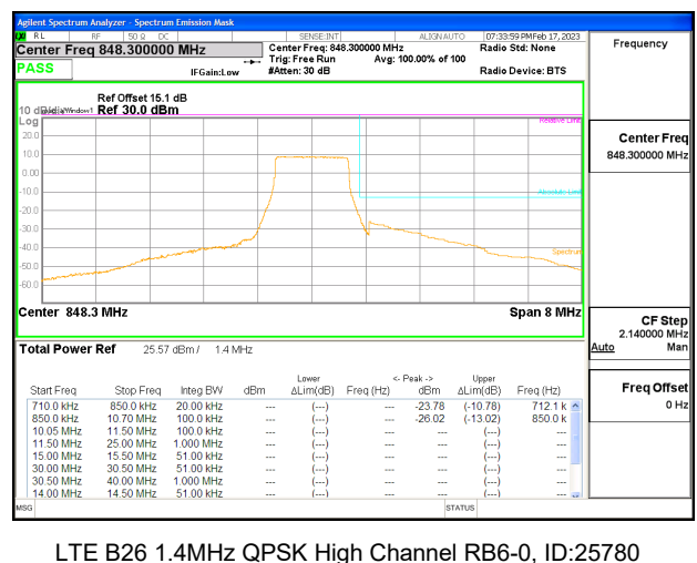
LTE B26 1.4MHz QPSK High Channel RB6-0, ID:25780
