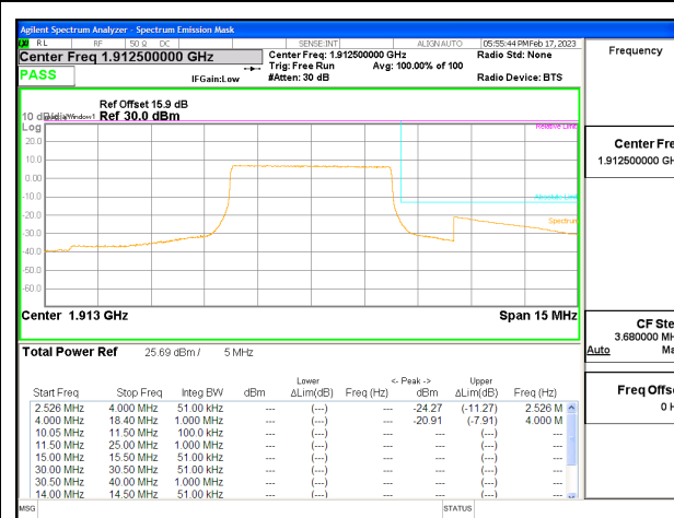
LTE B25 5MHz QPSK High Channel RB25-0 ID:25780
