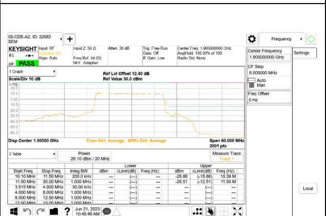
5G NR n25 20MHz BPSK High Channel RB100-0
