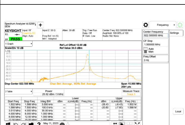
LTE B26 3MHz QPSK High Channel RB1-14
