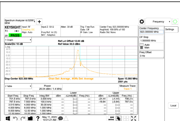
LTE B26 1.4MHz QPSK High Channel RB1-5
