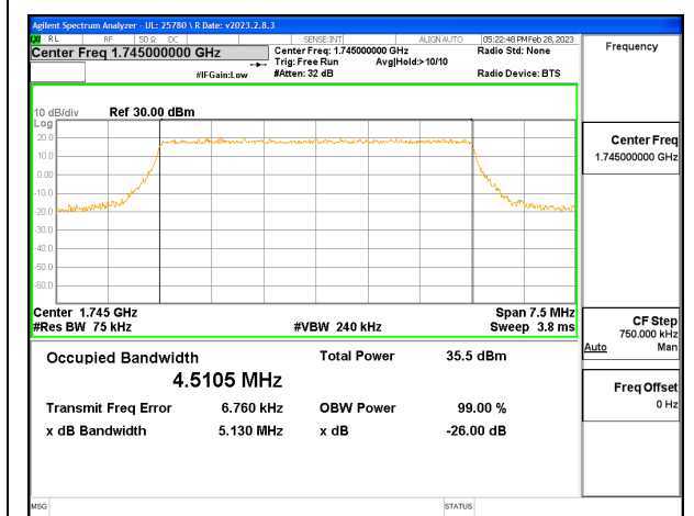
LTE B66 5MHz QPSK Middle Channel RB25-0
