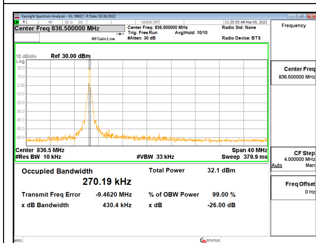
5G NR n26 20MHz Middle High Channel RB1-0
