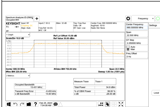
LTE B71 15MHz QPSK Middle Channel RB75-0
