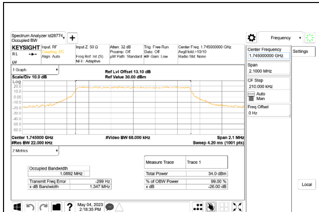
LTE B66 1.4MHz QPSK Middle Channel RB6-0
