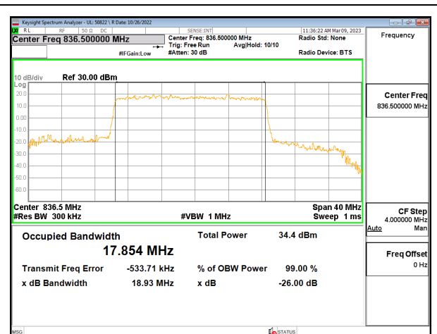
5G NR n26 20MHz BPSK Middle Channel RB100-0
