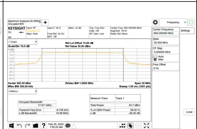
LTE B71 20MHz QPSK Middle Channel RB100-0
