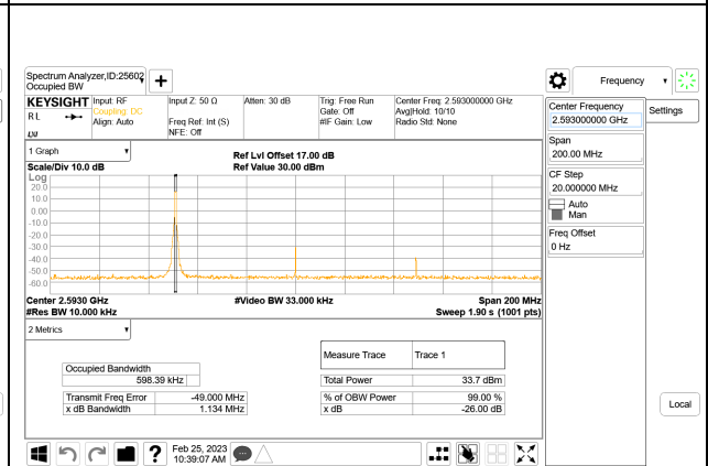
5G NR n41 100MHz BPSK Middle Channel RB1-0
