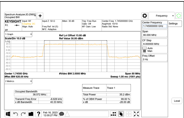
5G NR n66 40MHz BPSK Middle Channel RB216-0
