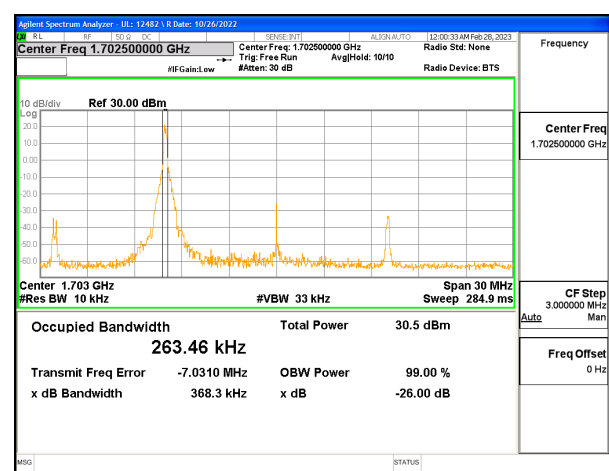
5G NR n70 10MHz BPSK Middle Channel RB1-0
