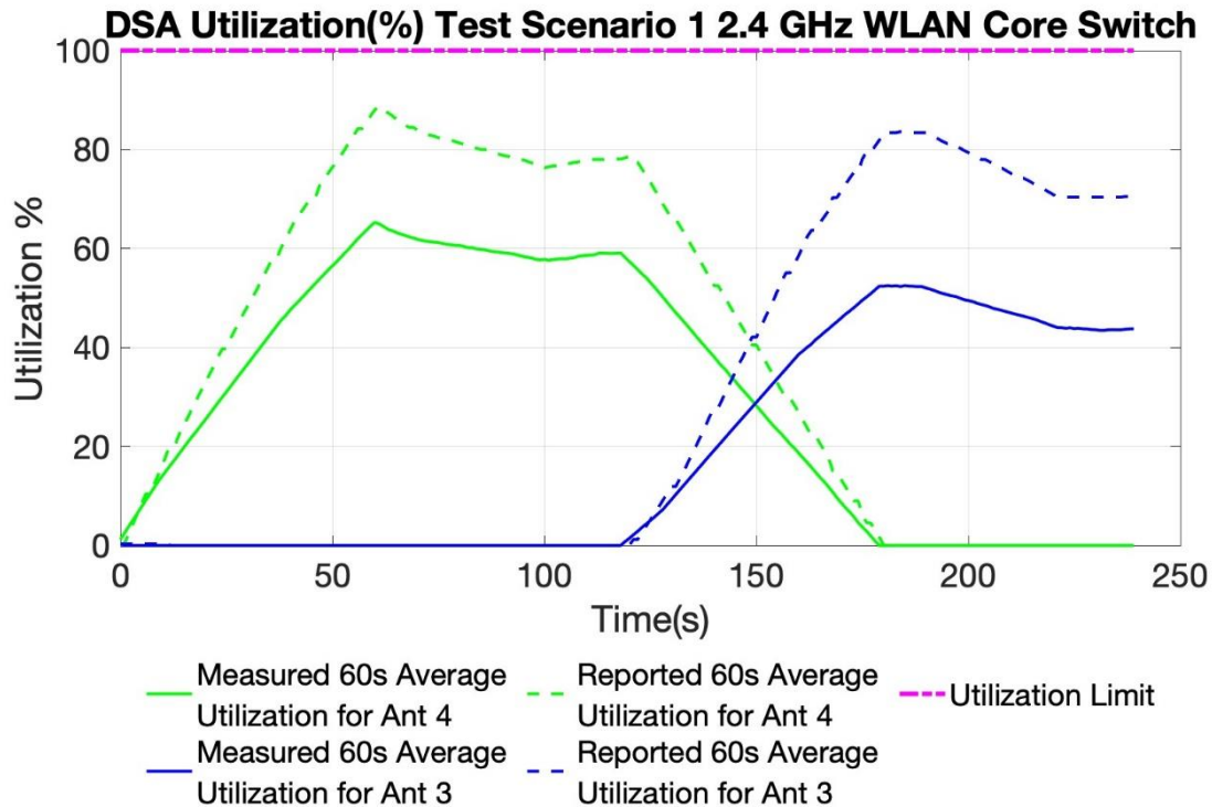
Figure 1: 60 Second Aggregated SAR Utilization vs Time, 2.4GHz
