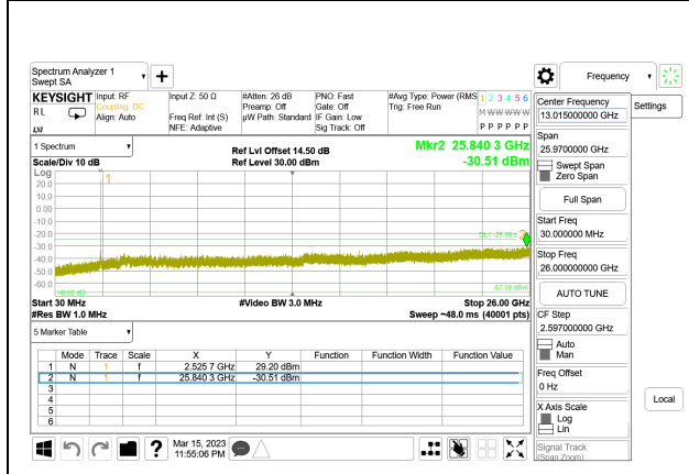
LTE B7 20MHz QPSK Middle Channel RB1-0, ID:19210
