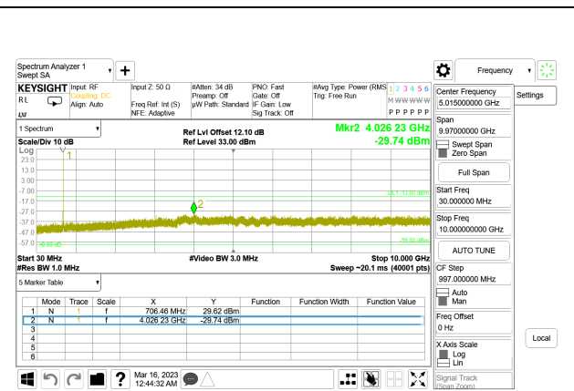
LTE B12 10MHz QPSK High Channel RB1-0, ID:28568
