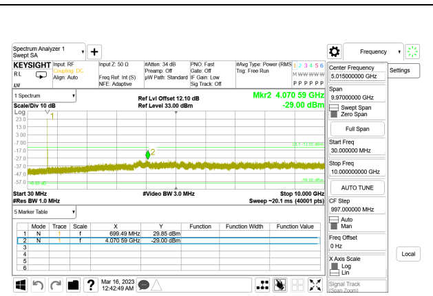
LTE B12 10MHz QPSK Low Channel RB1-0, ID:28568
