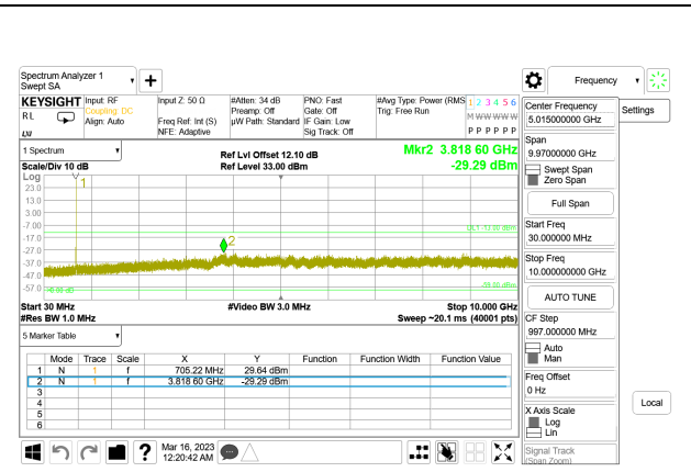
LTE B12 5MHz QPSK Middle Channel RB1-0, ID:28568
