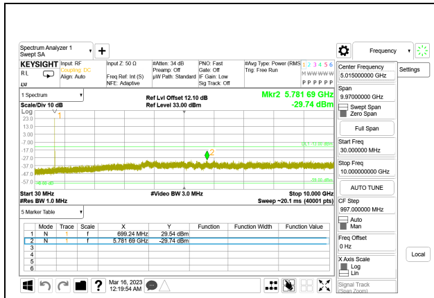
LTE B12 5MHz QPSK Low Channel RB1-0, ID:28568
