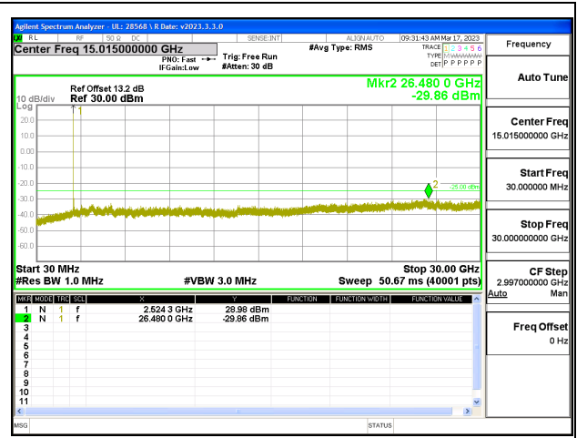
5G NR n7 25MHz BPSK Middle Channel RB1-1
