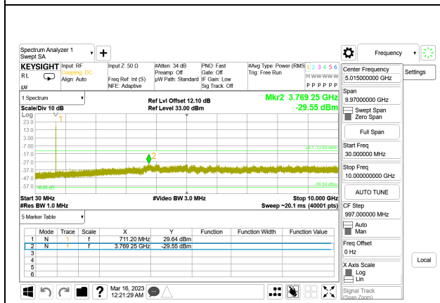
LTE B12 5MHz QPSK High Channel RB1-0, ID:28568
