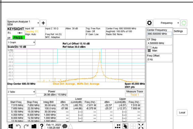
5G NR n71 15MHz BPSK Middle Channel RB1-78, ID:28567
