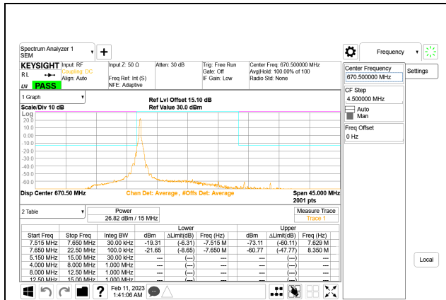
5G NR n71 15MHz BPSK Low Channel RB1-0, ID:28567
