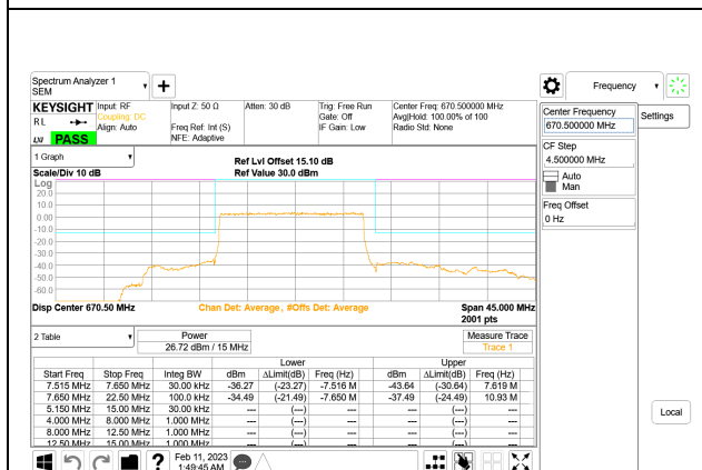
5G NR n71 15MHz BPSK Low Channel RB75-0, ID:28567
