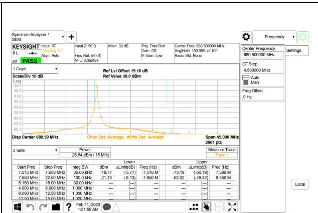
5G NR n71 15MHz BPSK Middle Channel RB1-0, ID:28567
