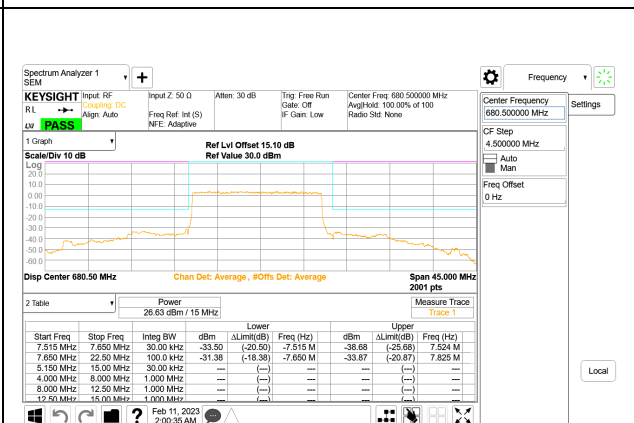
5G NR n71 15MHz BPSK Middle Channel RB75-0, ID:28567
