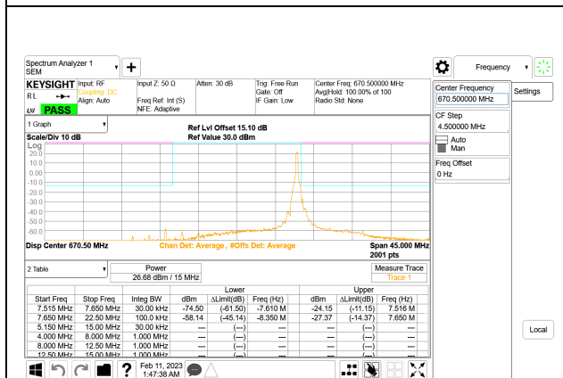
5G NR n71 15MHz BPSK Low Channel RB1-78, ID:28567
