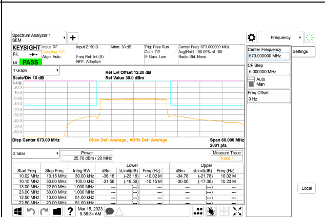
LTE B71 20MHz QPSK Low Channel RB100-0, ID:28567
