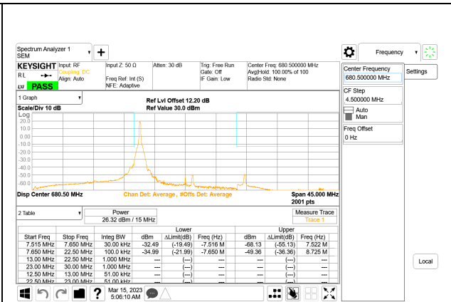
LTE B71 15MHz QPSK Middle Channel RB1-0, ID:28567
