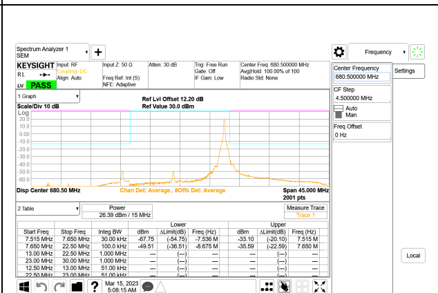
LTE B71 15MHz QPSK Middle Channel RB1-74, ID:28567
