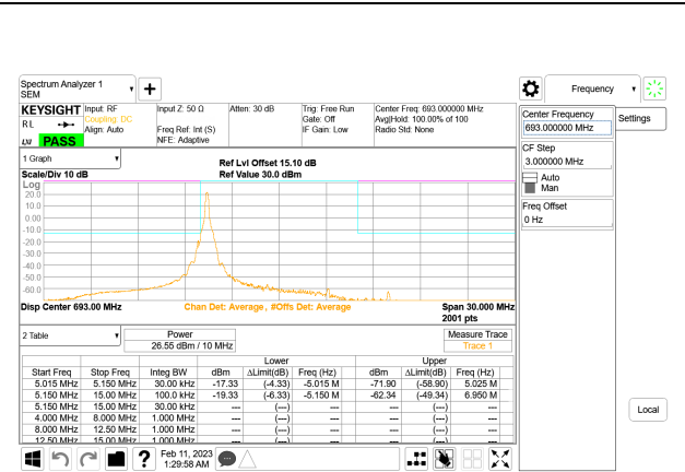
5G NR n71 10MHz BPSK High Channel RB1-0, ID:28567
