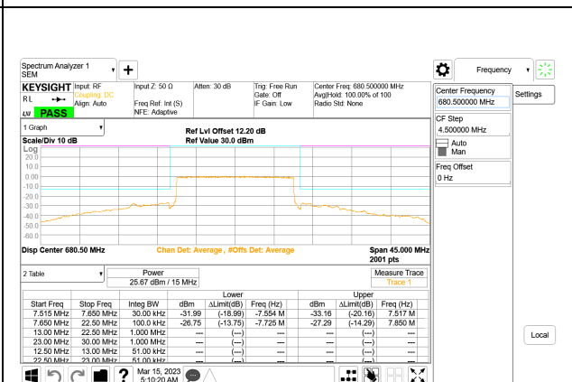
LTE B71 15MHz QPSK Middle Channel RB75-0, ID:28567
