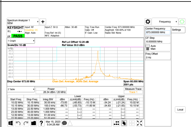
LTE B71 20MHz QPSK Low Channel RB1-99, ID:28567
