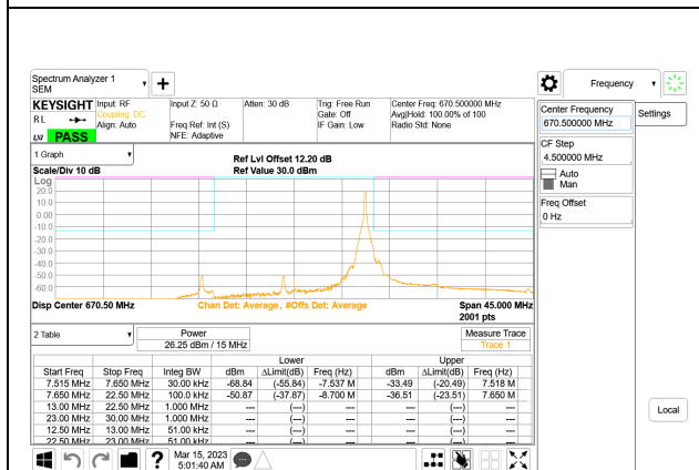
LTE B71 15MHz QPSK Low Channel RB1-74, ID:28567
