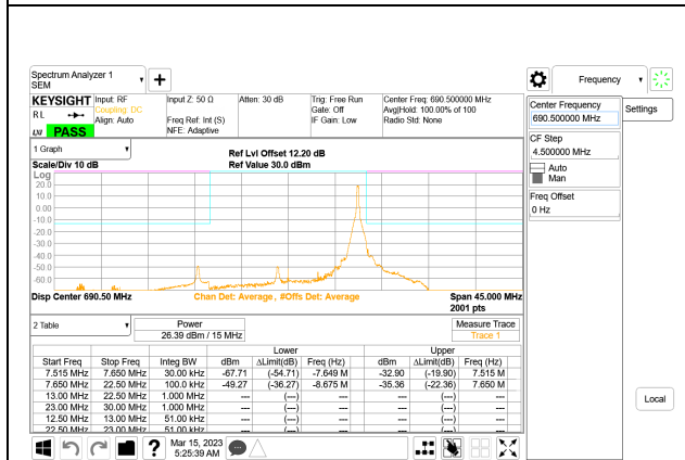
LTE B71 15MHz QPSK High Channel RB1-74, ID:28567
