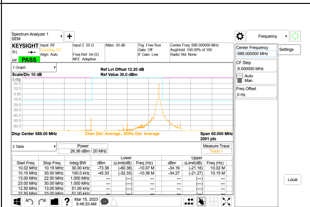
LTE B71 20MHz QPSK High Channel RB1-99, ID:28567
