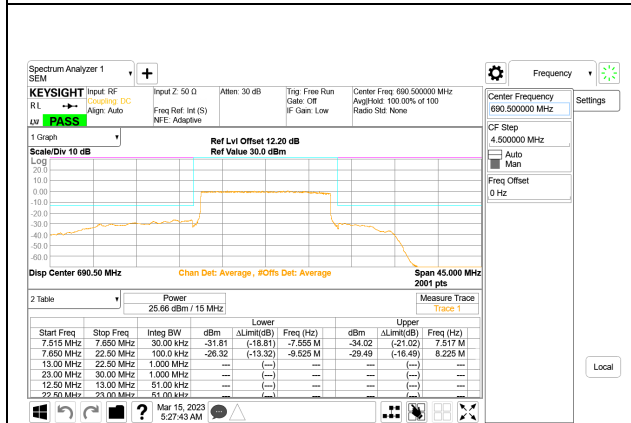
LTE B71 15MHz QPSK High Channel RB75-0, ID:28567
