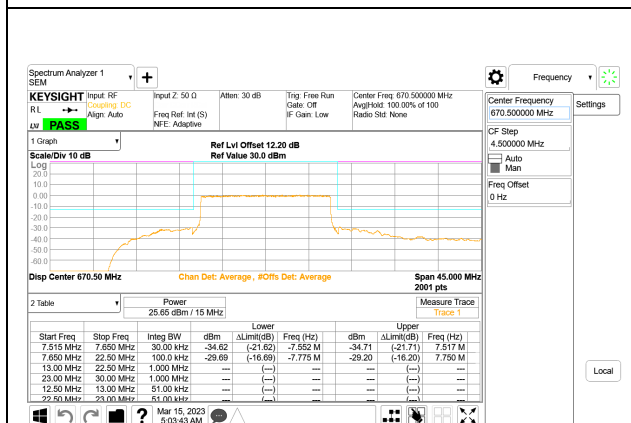
LTE B71 15MHz QPSK Low Channel RB75-0, ID:28567
