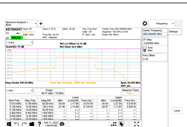
5G NR n71 10MHz BPSK High Channel RB50-0, ID:28567
