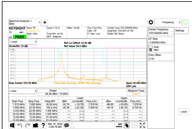
LTE B71 15MHz QPSK Low Channel RB1-0, ID:28567
