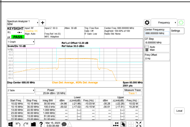
LTE B71 20MHz QPSK High Channel RB100-0, ID:28567
