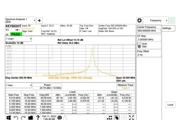
5G NR n71 10MHz BPSK High Channel RB1-51, ID:28567
