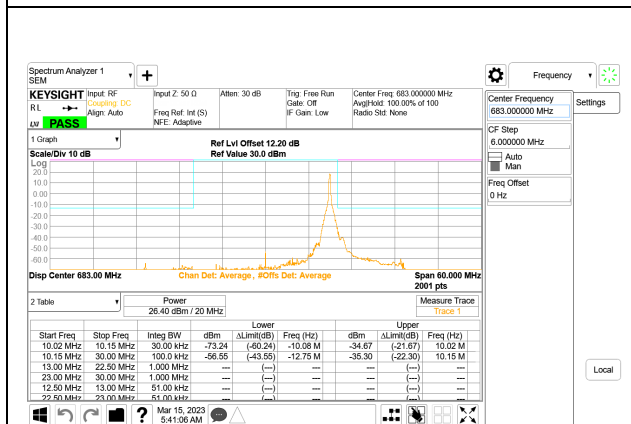
LTE B71 20MHz QPSK Middle Channel RB1-99, ID:28567
