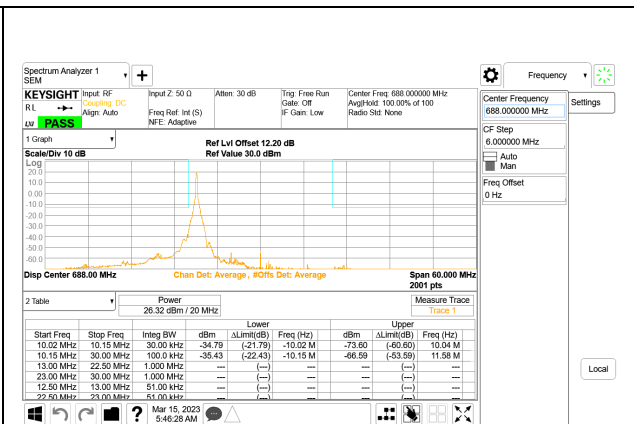
LTE B71 20MHz QPSK High Channel RB1-0, ID:28567
