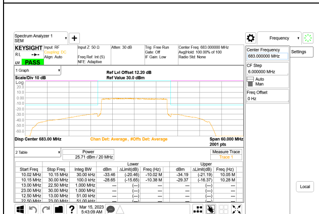
LTE B71 20MHz QPSK Middle Channel RB100-0, ID:28567
