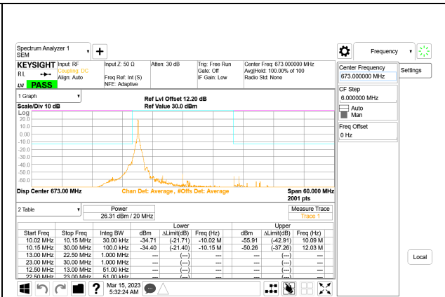
LTE B71 20MHz QPSK Low Channel RB1-0, ID:28567
