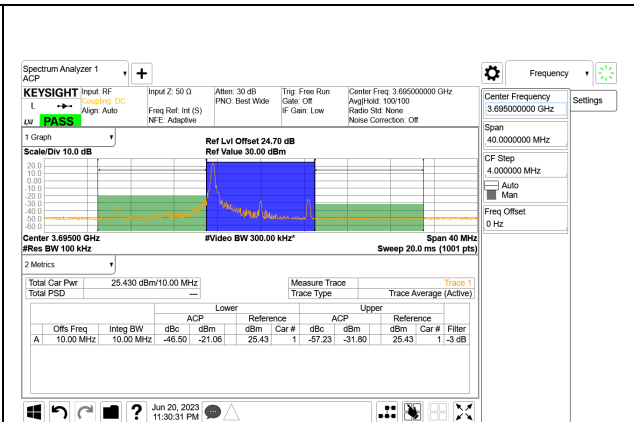
LTE B48 10MHz QPSK High Channel RB1-0, ID:39004
