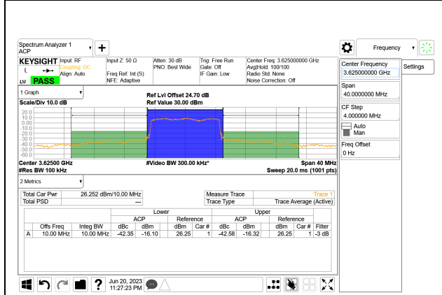
LTE B48 10MHz QPSK Middle Channel RB50-0, ID:39004
