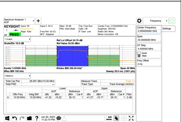
LTE B48 10MHz QPSK Low Channel RB50-0, ID:39004
