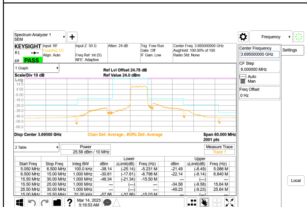
LTE B48 5MHz QPSK High Channel RB25-0, ID:39004
