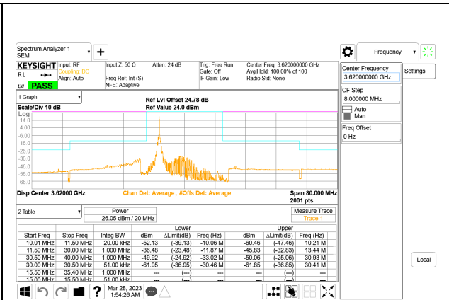
LTE B48 15MHz QPSK Middle Channel RB1-0, ID:39004
