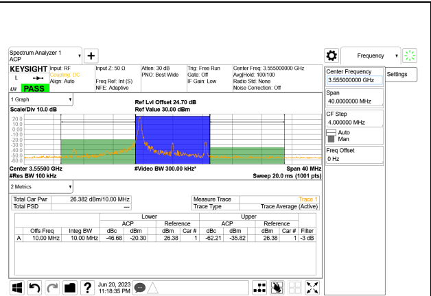
LTE B48 10MHz QPSK Low Channel RB1-0, ID:39004
