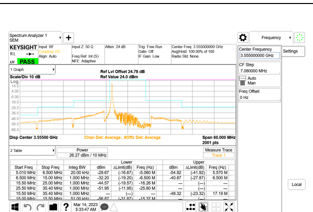
LTE B48 10MHz QPSK Low Channel RB1-0, ID:39004
