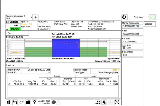
LTE B48 10MHz QPSK High Channel RB50-0, ID:39004
