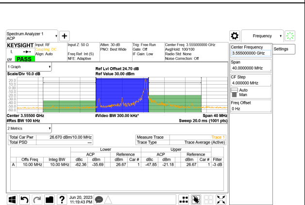
LTE B48 10MHz QPSK Low Channel RB1-49, ID:39004
