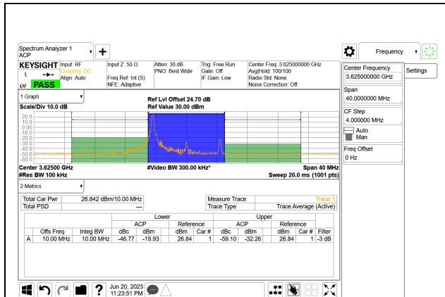
LTE B48 10MHz QPSK Middle Channel RB1-0, ID:39004
