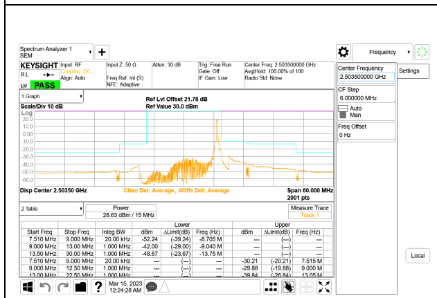
LTE B41 15MHz QPSK Low Channel RB1-74, ID:28567
