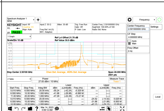
LTE B41 10MHz QPSK Low Channel RB1-49, ID:28567
