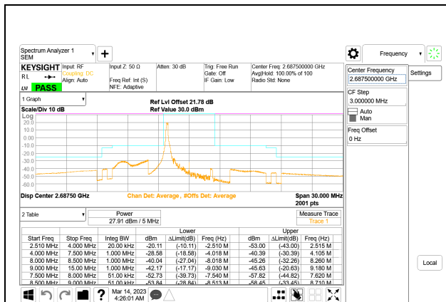
LTE B41 5MHz QPSK High Channel RB1-0, ID:28567
