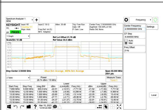
LTE B41 15MHz QPSK Middle Channel RB75-0, ID:28567
