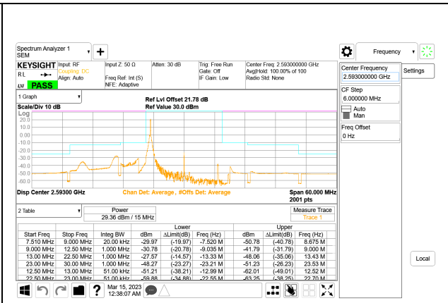
LTE B41 15MHz QPSK Middle Channel RB1-0, ID:28567
