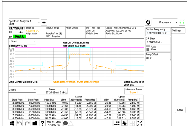
LTE B41 5MHz QPSK High Channel RB25-0, ID:28567
