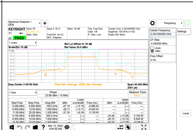
LTE B41 10MHz QPSK Low Channel RB50-0, ID:28567
