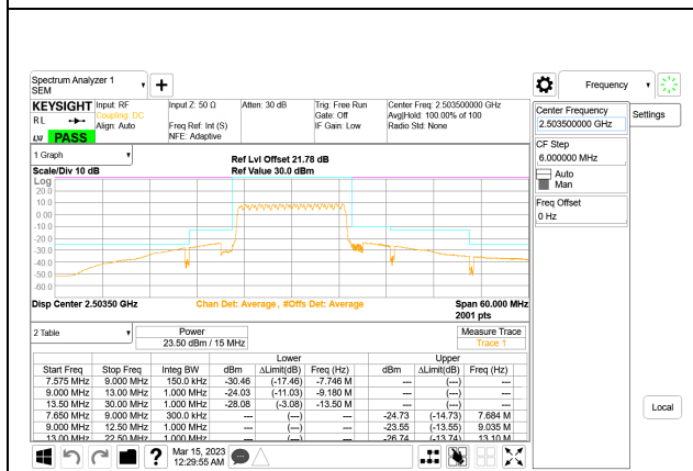
LTE B41 15MHz QPSK Low Channel RB75-0, ID:28567
