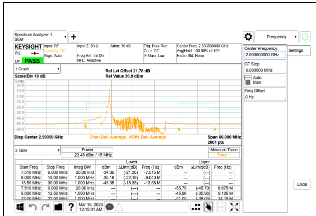
LTE B41 15MHz QPSK Low Channel RB1-0, ID:28567
