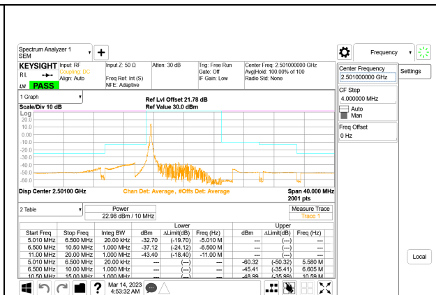
LTE B41 10MHz QPSK Low Channel RB1-0, ID:28567
