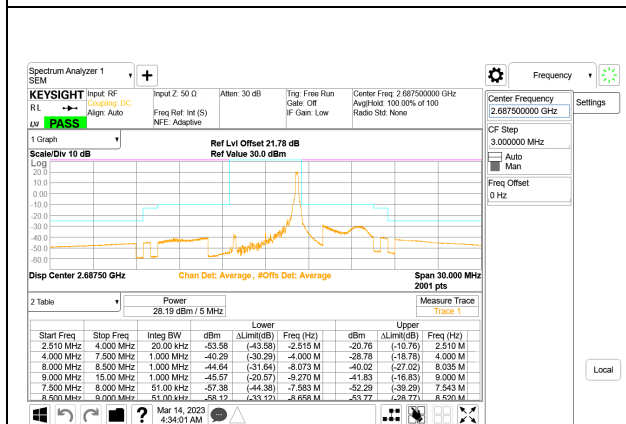
LTE B41 5MHz QPSK High Channel RB1-24, ID:28567
