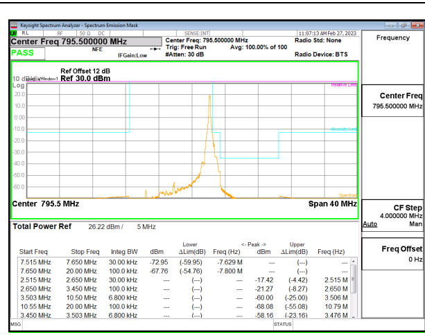
5G NR n14 5MHz BPSK High Channel RB1-24, ID:28568
