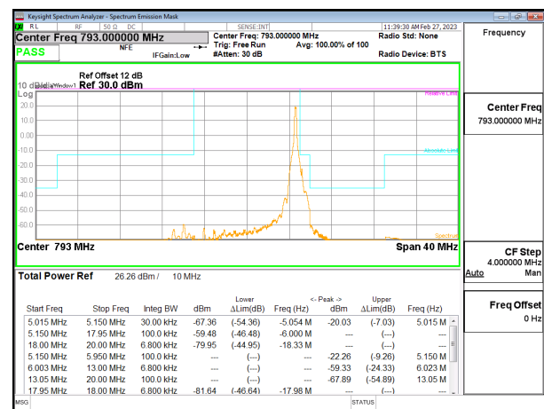
5G NR n14 10MHz BPSK Middle Channel RB1-51, ID:28568
