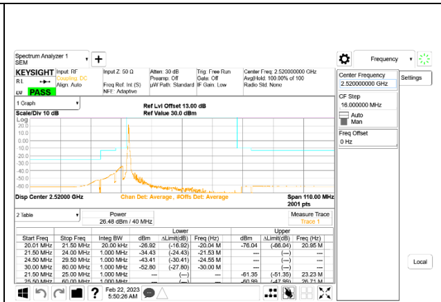
5G NR n7 40MHz BPSK Low Channel RB1-0, ID:27957
