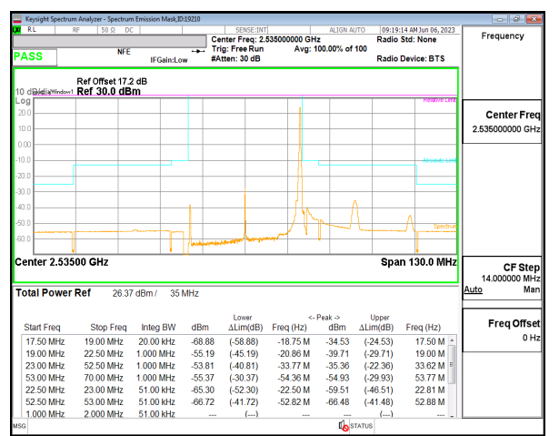
5G NR n7 35MHz BPSK Middle Channel RB1-187
