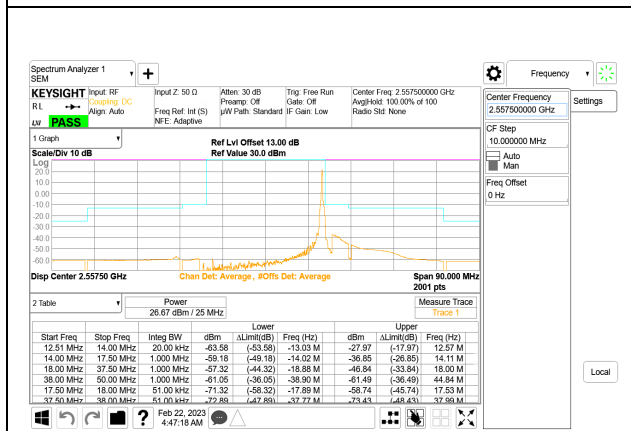
5G NR n7 25MHz BPSK High Channel RB1-132, ID:27957
