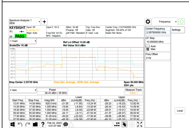
5G NR n7 25MHz BPSK High Channel RB128-0, ID:27957
