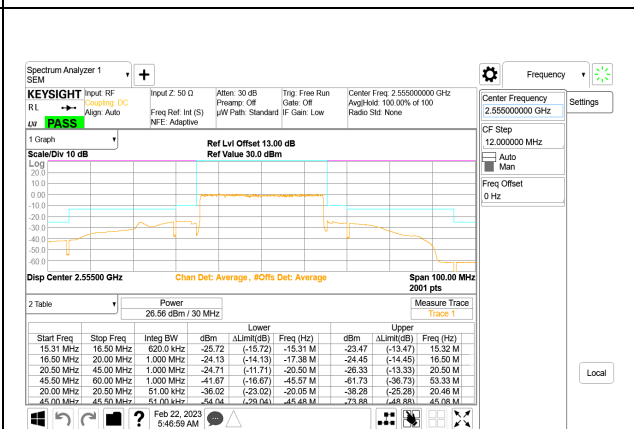
5G NR n7 30MHz BPSK High Channel RB160-0, ID:27957
