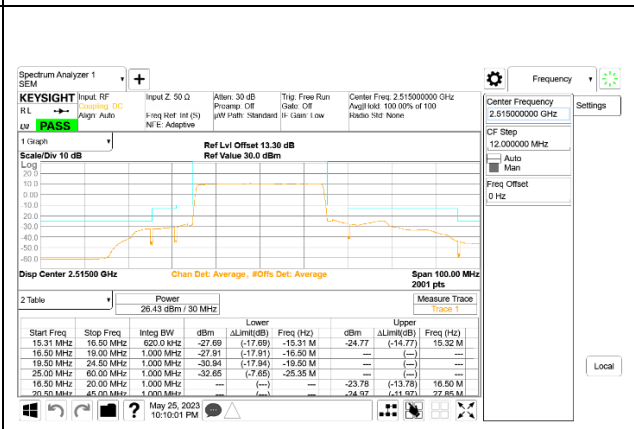
5G NR n7 30MHz BPSK Low Channel RB160-0 ID:19210
