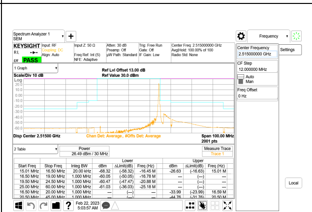
5G NR n7 30MHz BPSK Low Channel RB1-159, ID:27957
