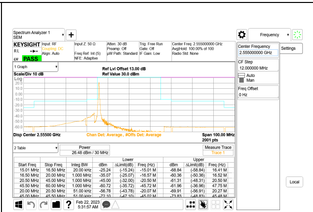
5G NR n7 30MHz BPSK High Channel RB1-0, ID:27957
