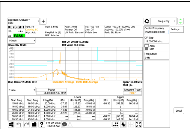
5G NR n7 30MHz BPSK Low Channel RB1-0, ID:27957
