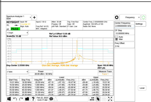
5G NR n7 30MHz BPSK High Channel RB1-159, ID:27957
