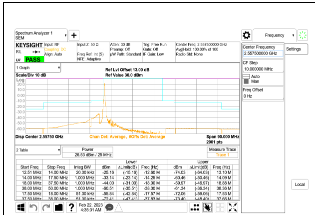
5G NR n7 25MHz BPSK High Channel RB1-0, ID:27957
