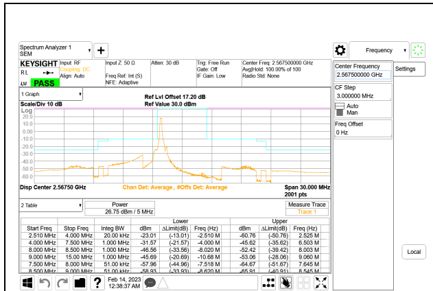
LTE B7 5MHz QPSK High Channel RB1-0, ID:25780
