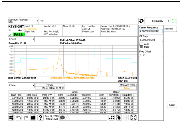
LTE B7 15MHz QPSK High Channel RB1-0, ID:25780
