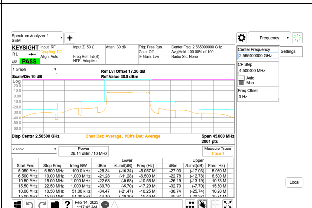
LTE B7 10MHz QPSK High Channel RB50-0, ID:25780
