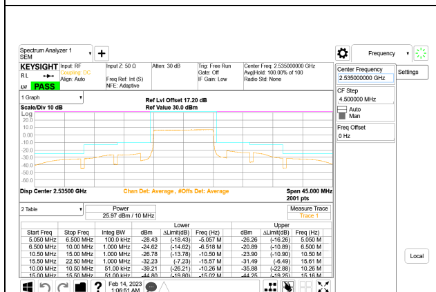
LTE B7 10MHz QPSK Middle Channel RB50-0, ID:25780
