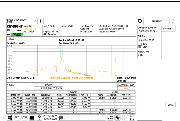
LTE B7 10MHz QPSK Low Channel RB1-0, ID:25780
