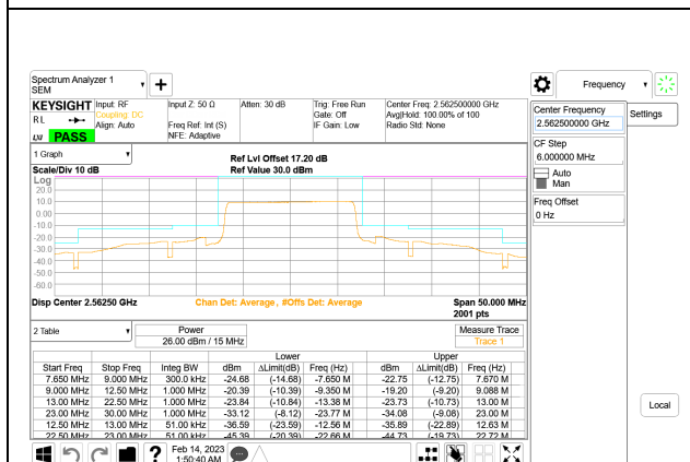
LTE B7 15MHz QPSK High Channel RB75-0, ID:25780
