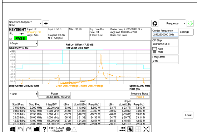
LTE B7 15MHz QPSK High Channel RB1-74, ID:25780
