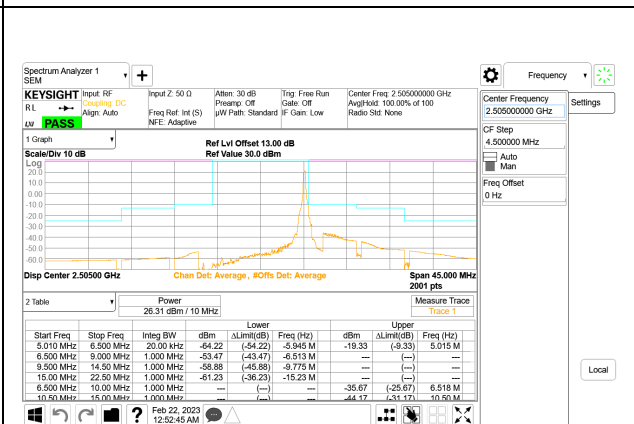
5G NR n7 10MHz BPSK Low Channel RB1-51, ID:27957
