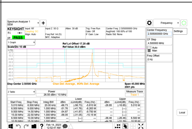
LTE B7 10MHz QPSK Low Channel RB1-49, ID:25780
