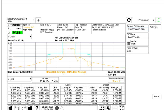
5G NR n7 5MHz BPSK High Channel RB25-0, ID:27957
