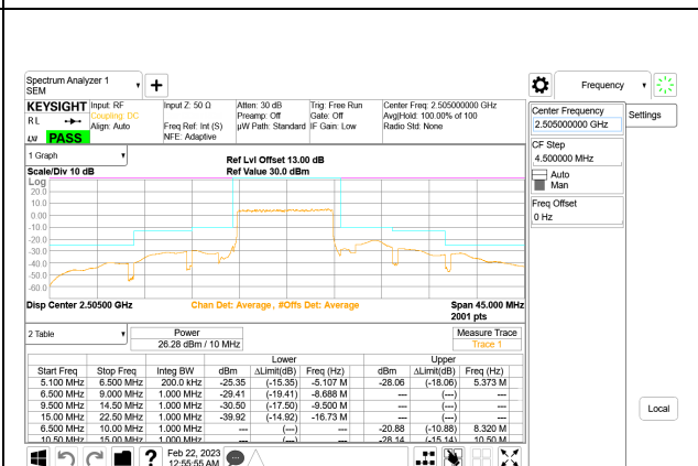
5G NR n7 10MHz BPSK Low Channel RB50-0, ID:27957
