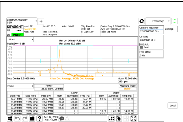
LTE B7 20MHz QPSK Low Channel RB1-0, ID:25780
