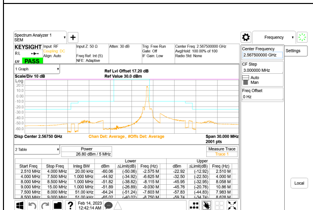
LTE B7 5MHz QPSK High Channel RB1-24, ID:25780
