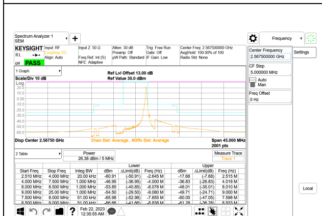
5G NR n7 5MHz BPSK High Channel RB1-24, ID:27957
