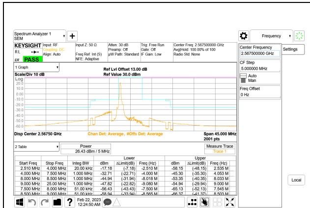
5G NR n7 5MHz BPSK High Channel RB1-0, ID:27957
