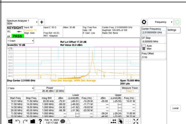
LTE B7 20MHz QPSK Low Channel RB1-99, ID:25780
