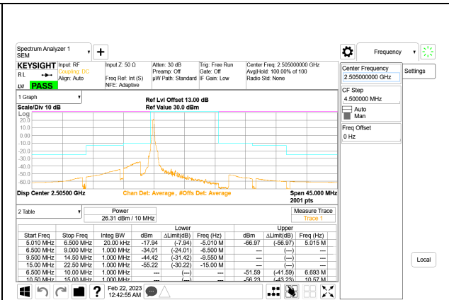
5G NR n7 10MHz BPSK Low Channel RB1-0, ID:27957
