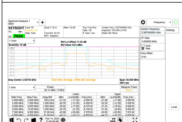
LTE B7 5MHz QPSK High Channel RB25-0, ID:25780
