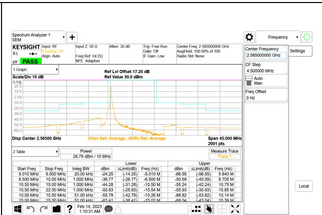
LTE B7 10MHz QPSK High Channel RB1-0, ID:25780
