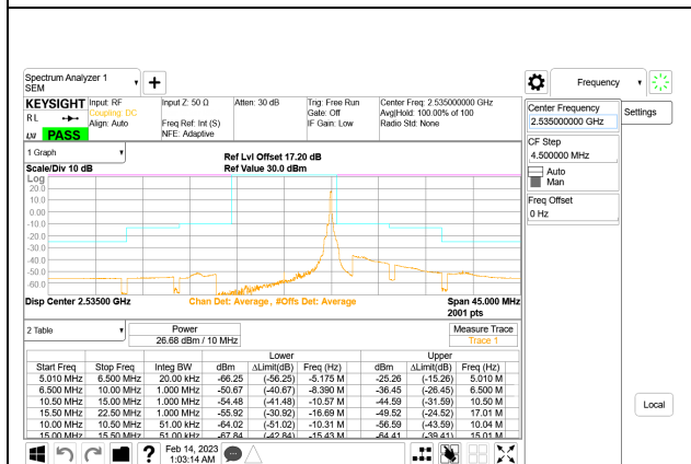
LTE B7 10MHz QPSK Middle Channel RB1-49, ID:25780
