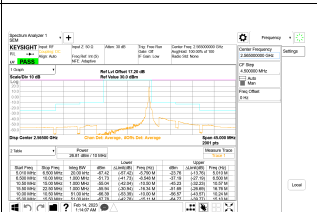
LTE B7 10MHz QPSK High Channel RB1-49, ID:25780
