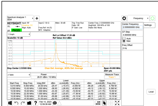
LTE B7 10MHz QPSK Middle Channel RB1-0, ID:25780
