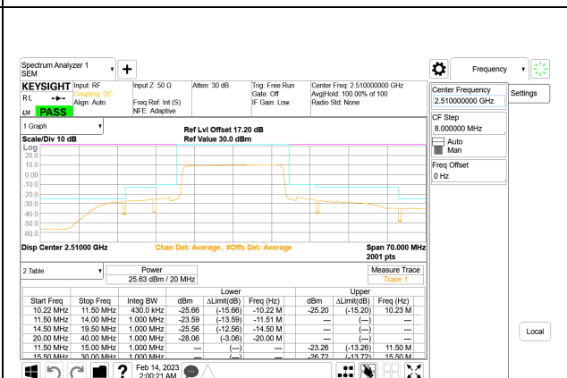
LTE B7 20MHz QPSK Low Channel RB100-0, ID:25780
