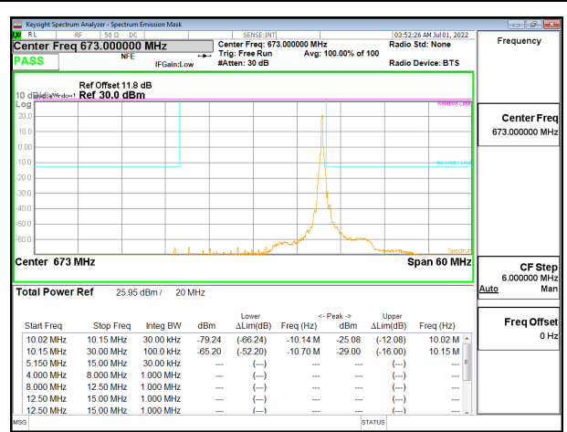
5G NR n71 20MHz BPSK Low Channel RB1-105, ID: 28774
