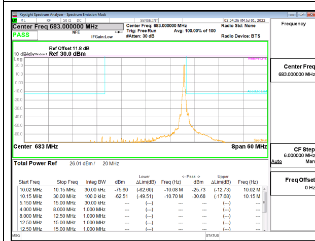
5G NR n71 20MHz BPSK Middle Channel RB1-105, ID: 28774
