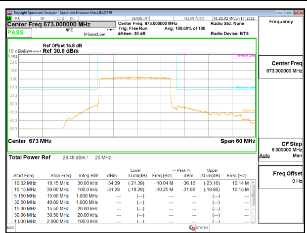
5G NR n71 20MHz BPSK Low Channel RB100-0
