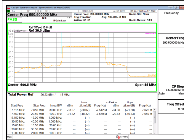
5G NR n71 15MHz BPSK High Channel RB75-0
