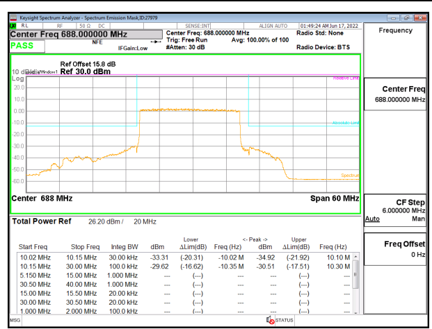
5G NR n71 20MHz BPSK High Channel RB100-0
