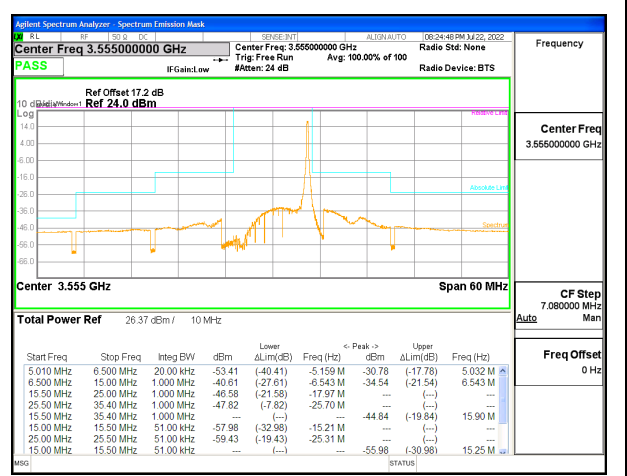
LTE B48 10MHz QPSK Low Channel RB1-49, ID:25780
