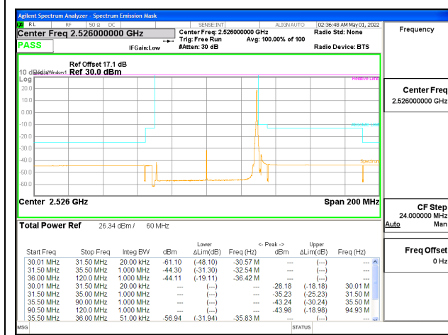
5G NR n41 60MHz BPSK Low Channel RB1-161, ID:25780
