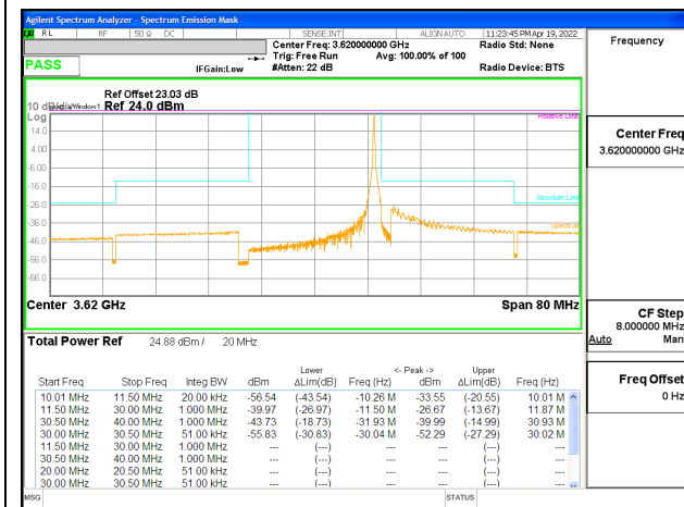
LTE B48 20MHz QPSK Middle Channel RB1-99, ID:25602
