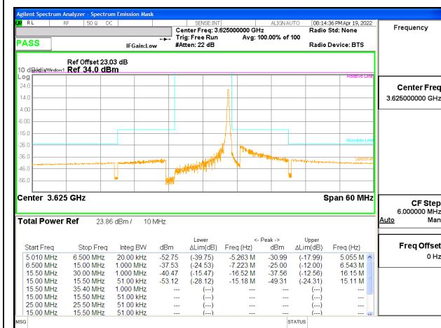
LTE B48 10MHz QPSK Middle Channel RB1-49, ID:25602
