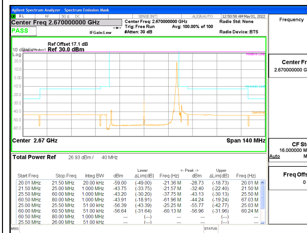
5G NR n41 40MHz BPSK High Channel RB1-105, ID:25780
