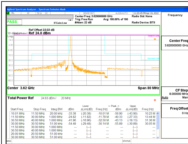
LTE B48 20MHz QPSK Middle Channel RB1-0, ID:25602
