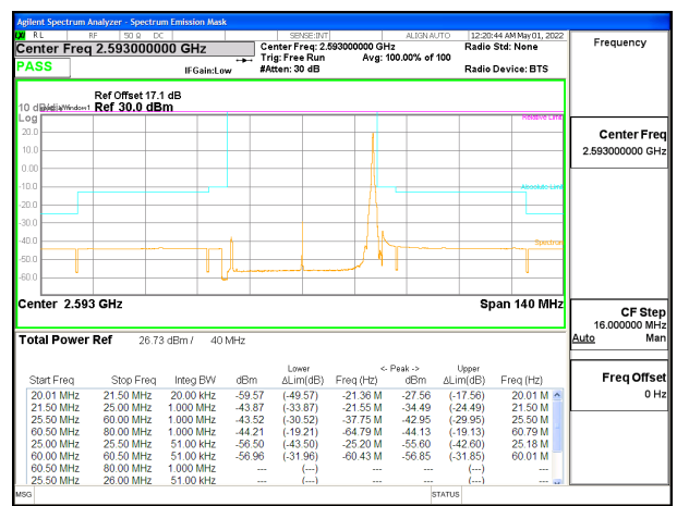
5G NR n41 40MHz BPSK Middle Channel RB1-105, ID:25780
