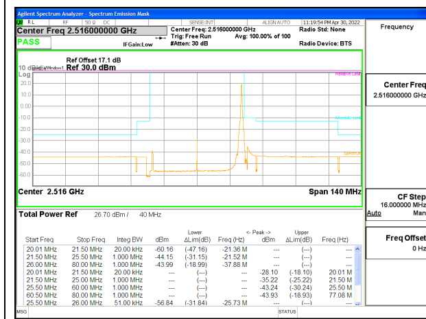
5G NR n41 40MHz BPSK Low Channel RB1-105, ID:25780
