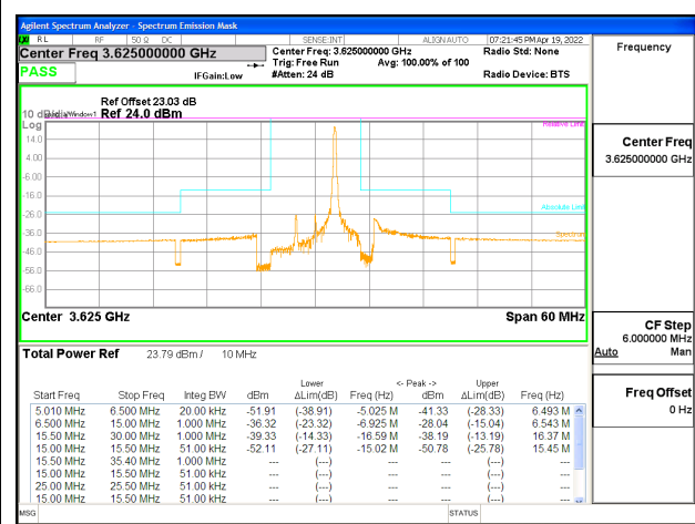
LTE B48 5MHz QPSK Middle Channel RB1-24, ID:25602
