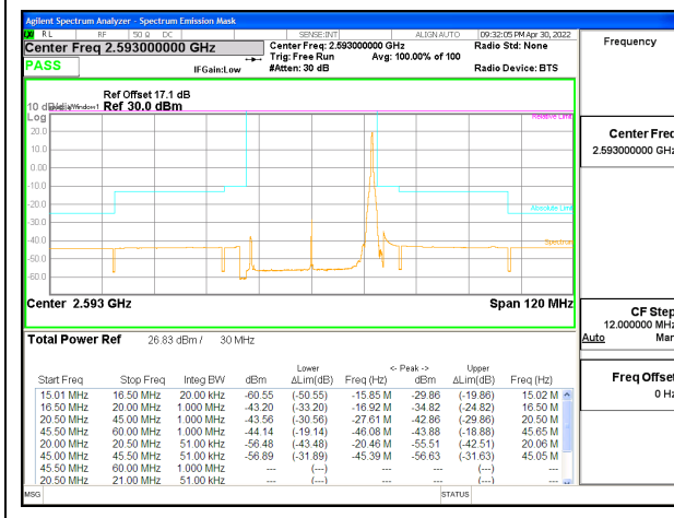
5G NR n41 30MHz BPSK Middle Channel RB1-77, ID:25780
