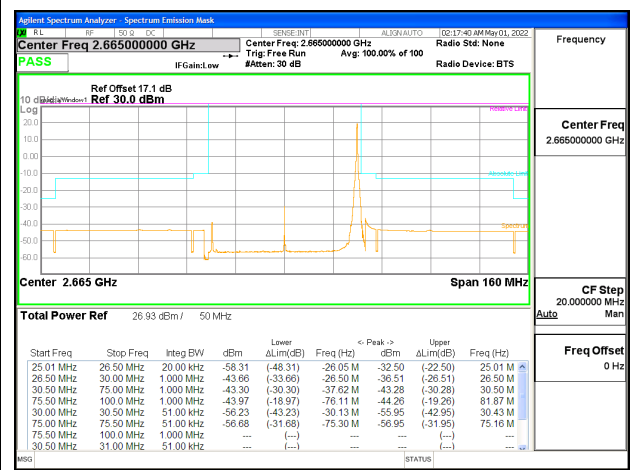
5G NR n41 50MHz BPSK High Channel RB1-132, ID:25780
