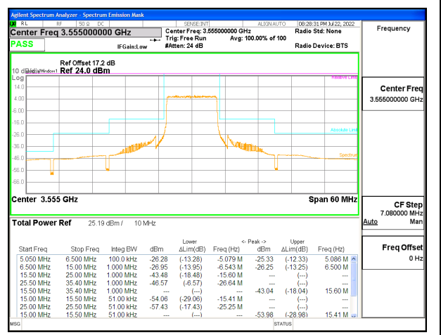
LTE B48 10MHz QPSK Low Channel RB50-0, ID:25780
