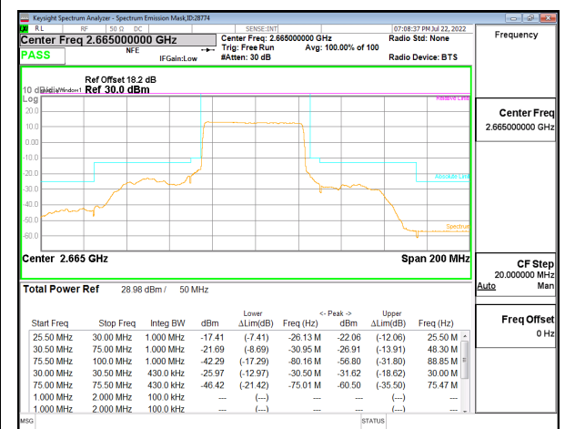
5G NR n41 50MHz BPSK High Channel RB128-0, ID:28774
