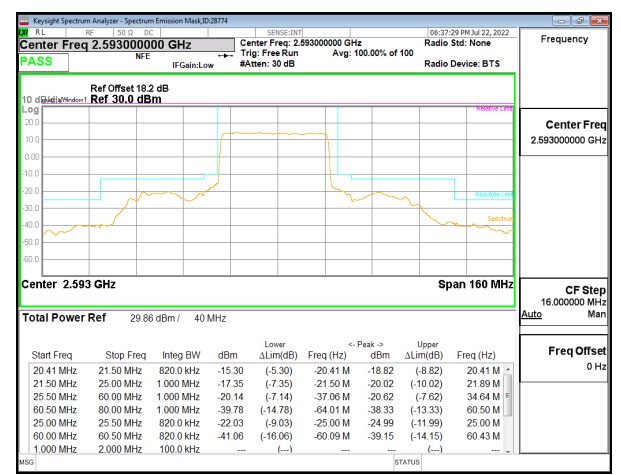
5G NR n41 40MHz BPSK Middle Channel RB100-0, ID:28774
