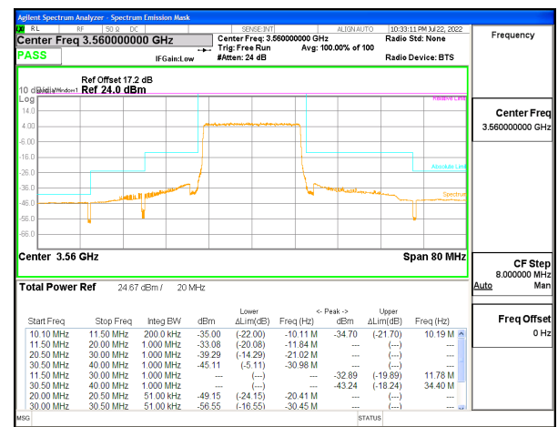
LTE B48 20MHz QPSK Low Channel RB100-0, ID:25780
