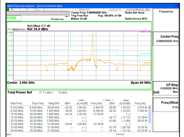
LTE B48 10MHz QPSK High Channel RB1-49, ID:25780
