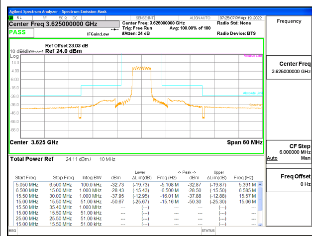
LTE B48 5MHz QPSK Middle Channel RB25-0, ID:25602
