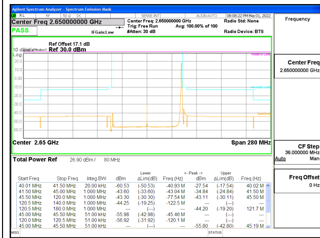
5G NR n41 80MHz BPSK High Channel RB1-216, ID:25780
