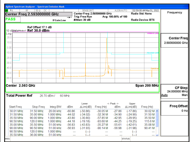
5G NR n41 60MHz BPSK Middle Channel RB1-161, ID:25780
