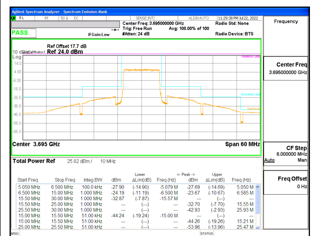
LTE B48 10MHz QPSK High Channel RB50-0, ID:25780
