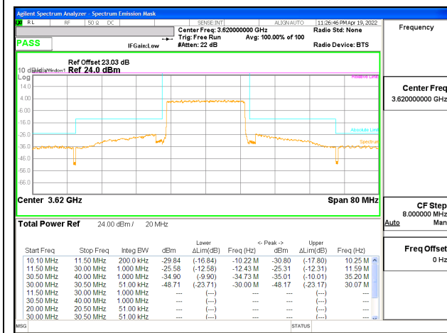
LTE B48 20MHz QPSK Middle Channel RB100-0, ID:25602
