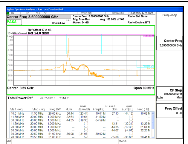
LTE B48 20MHz QPSK High Channel RB1-0, ID:25602
