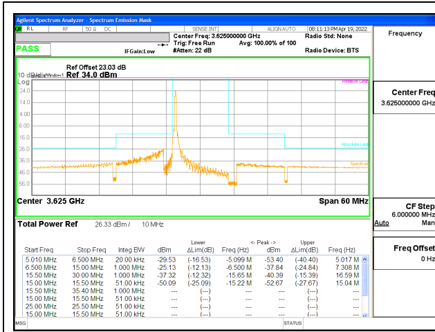
LTE B48 10MHz QPSK Middle Channel RB1-0, ID:25602
