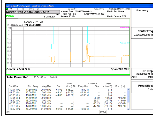
5G NR n41 80MHz BPSK Low Channel RB1-216, ID:25780
