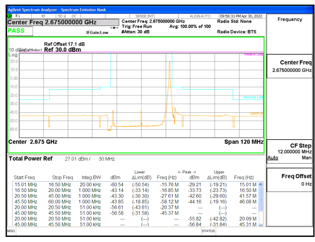
5G NR n41 30MHz BPSK High Channel RB1-77, ID:25780
