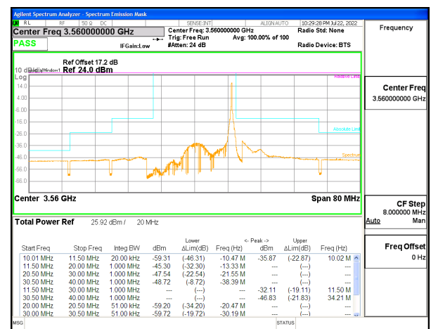
LTE B48 20MHz QPSK Low Channel RB1-99, ID:25780
