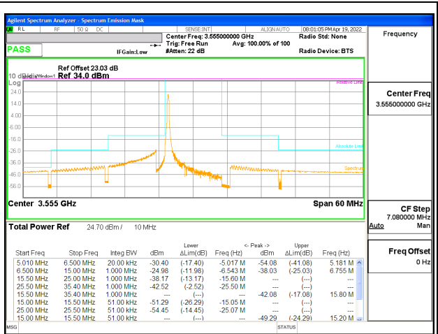
LTE B48 10MHz QPSK Low Channel RB1-0, ID:25602
