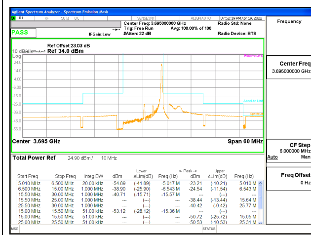
LTE B48 5MHz QPSK High Channel RB1-24, ID:25602
