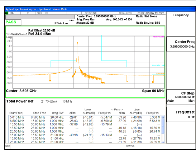
LTE B48 10MHz QPSK High Channel RB1-0, ID:25602
