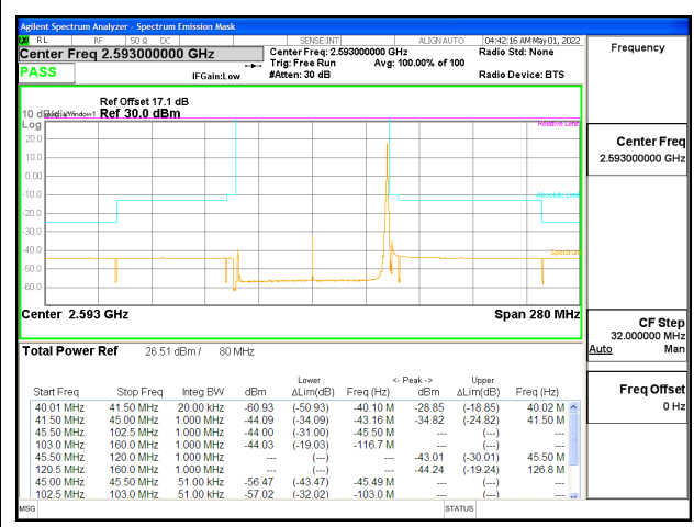
5G NR n41 80MHz BPSK Middle Channel RB1-216, ID:25780
