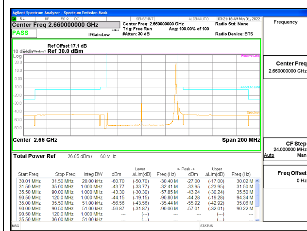
5G NR n41 60MHz BPSK High Channel RB1-161, ID:25780
