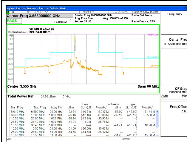
LTE B48 5MHz QPSK Low Channel RB1-0, ID:25602
