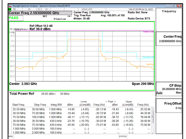
5G NR n41 50MHz BPSK Middle Channel RB128-0, ID:28774
