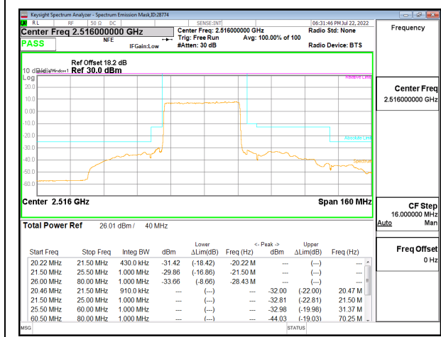
5G NR n41 40MHz BPSK Low Channel RB100-0, ID:28774
