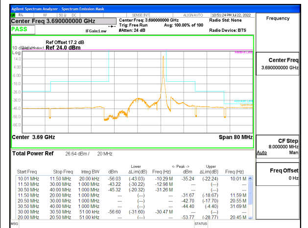
LTE B48 20MHz QPSK High Channel RB1-99, ID:25780
