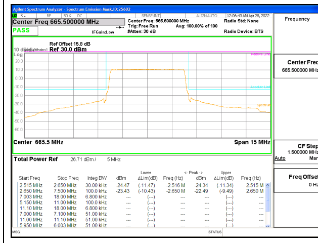
LTE B71 5MHz QPSK Low Channel RB25-0
