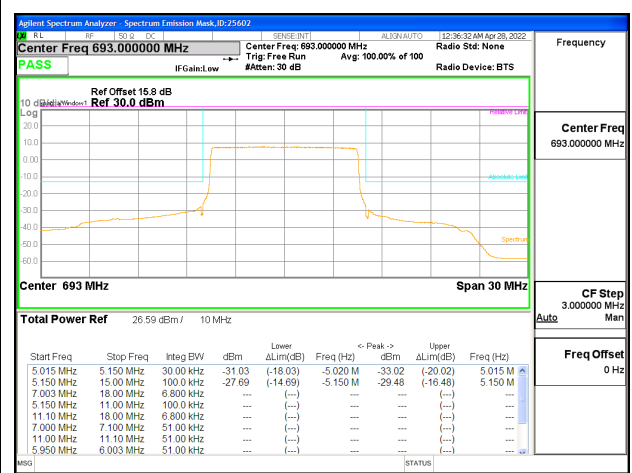
LTE B71 10MHz QPSK High Channel RB50-0
