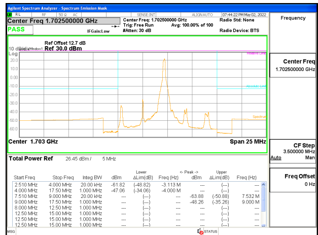
NR n70 5MHz BPSK Middle Channel (Lower Block) RB1-25, ID:12482
