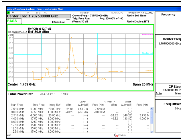
5G NR n70 5MHz BPSK High Channel (Upper Block) RB1-0, ID:12482
