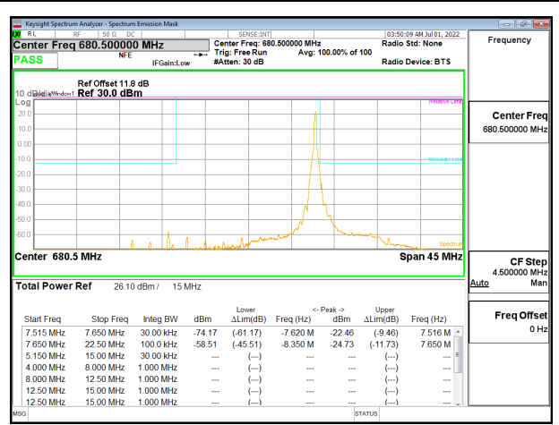
5G NR n71 15MHz BPSK Middle Channel RB1-78, ID: 28774
