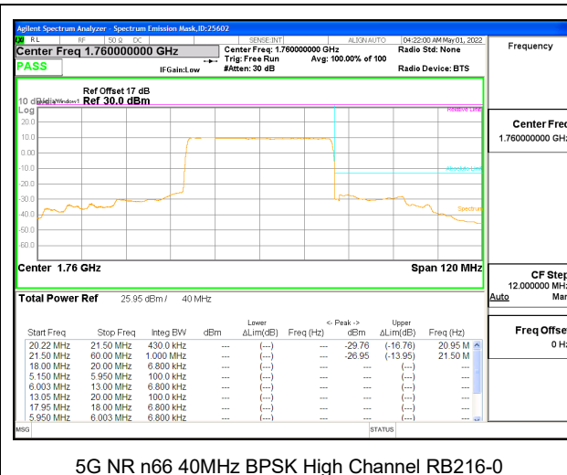
5G NR n66 40MHz BPSK High Channel RB216-0
