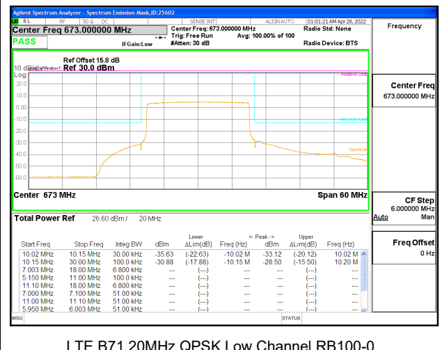
LTE B71 20MHz QPSK Low Channel RB100-0
