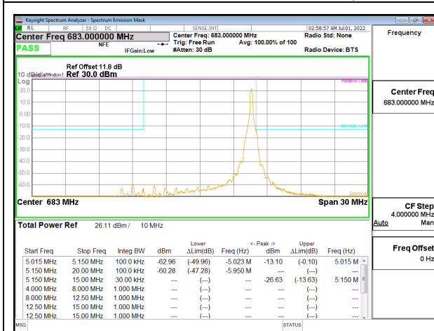
5G NR n71 10MHz BPSK Middle Channel RB1-51, ID: 28774
