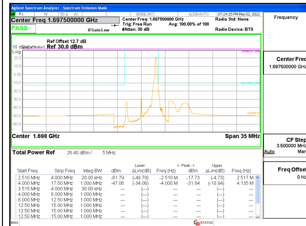
5G NR n70 5MHz BPSK Low Channel (Lower Block) RB1-25, ID:12482
