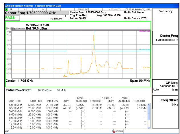
5G NR n70 10MHz BPSK High Channel (Upper Block) RB1-51
