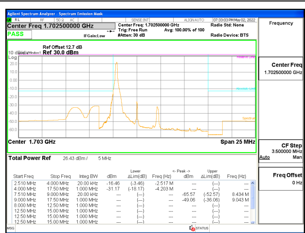
NR n70 5MHz BPSK Middle Channel (Lower Block) RB1-0, ID:12482
