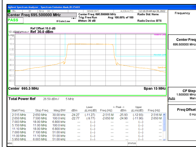
LTE B71 5MHz QPSK High Channel RB25-0
