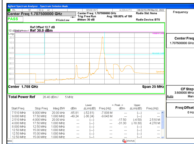
5G NR n70 5MHz BPSK High Channel (Upper Block) RB1-25
