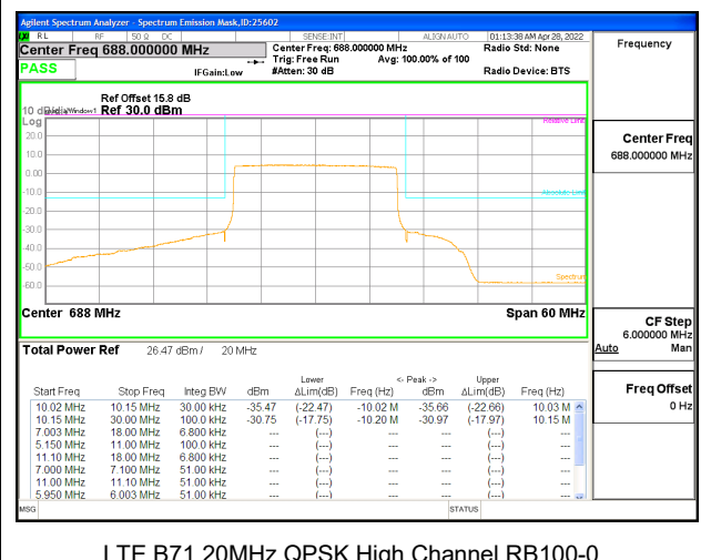
LTE B71 20MHz QPSK High Channel RB100-0
