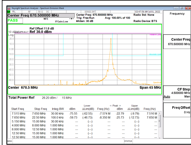
5G NR n71 15MHz BPSK Low Channel RB1-78, ID: 28774
