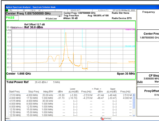
5G NR n70 5MHz BPSK Low Channel (Lower Block) RB1-0, ID:12482
