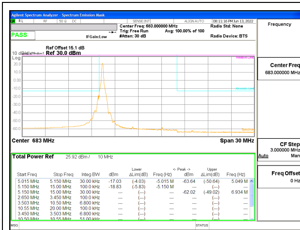
5G NR n71 10MHz BPSK Middle Channel RB1-0, ID: 28774
