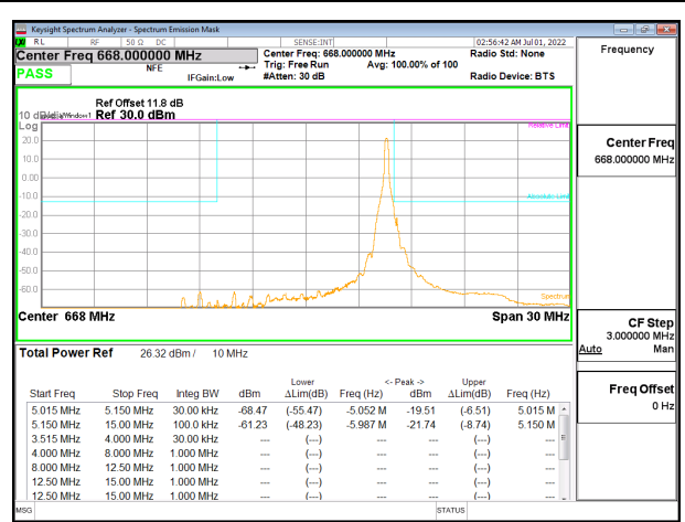
5G NR n71 10MHz BPSK Low Channel RB1-51 ID 28774
