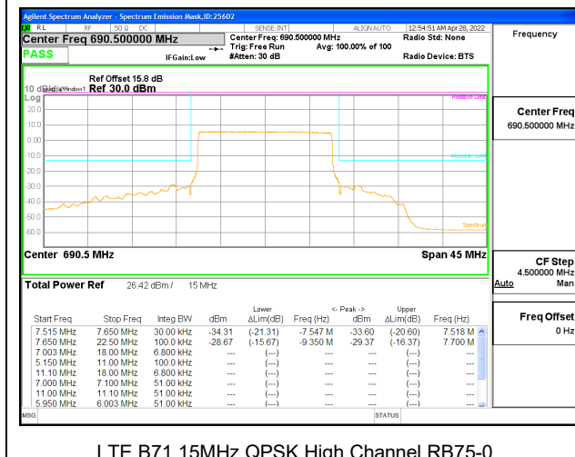
LTE B71 15MHz QPSK High Channel RB75-0
