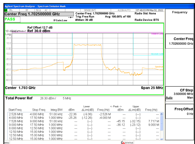
5G NR n70 5MHz BPSK Middle Channel (Lower Block) RB25-0, ID:12482
