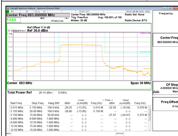
5G NR n71 10MHz BPSK Middle Channel RB50-0 ID 28774
