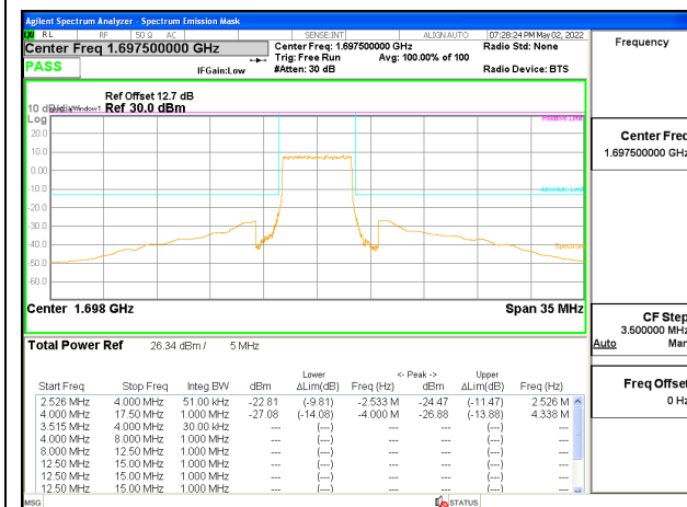
5G NR n70 5MHz BPSK Low Channel (Lower Block) RB25-0, ID:12482
