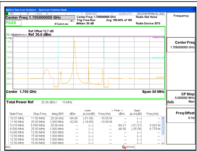
5G NR n70 10MHz BPSK High Channel (Lower Block) RB1-0, ID:12482
