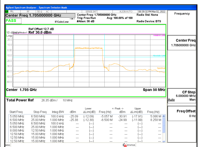
5G NR n70 10MHz BPSK High Channel (Upper Block) RB50-0, ID:12482
