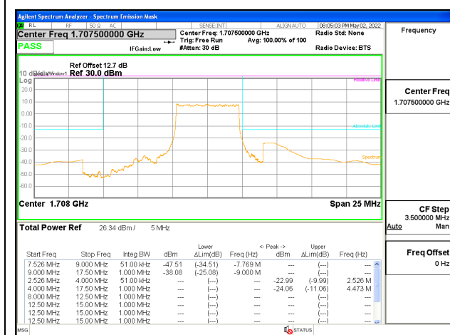
5G NR n70 5MHz BPSK High Channel (Upper Block) RB25-0, ID:12482
