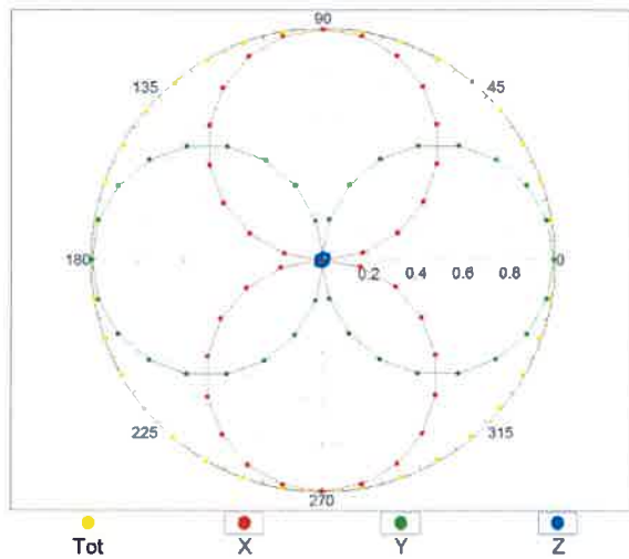
f=1800 MHz,R22,0°
