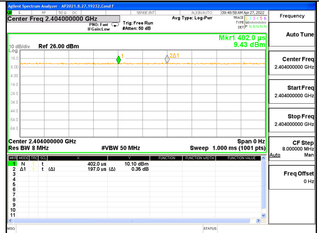
DUTY CYCLE HDR8
