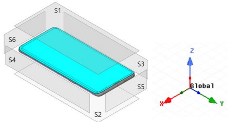
Figure 3-1: EUT surface definition
